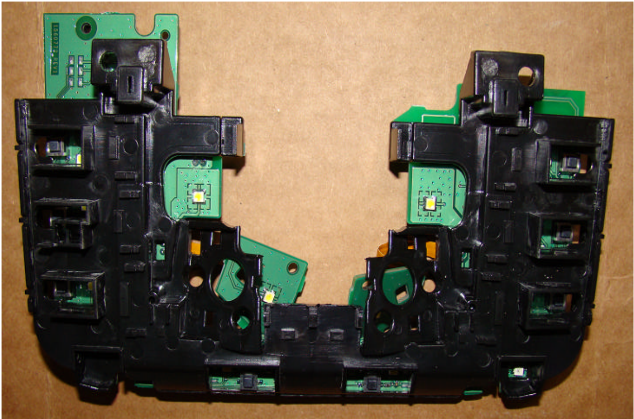
Internal View- Rear
