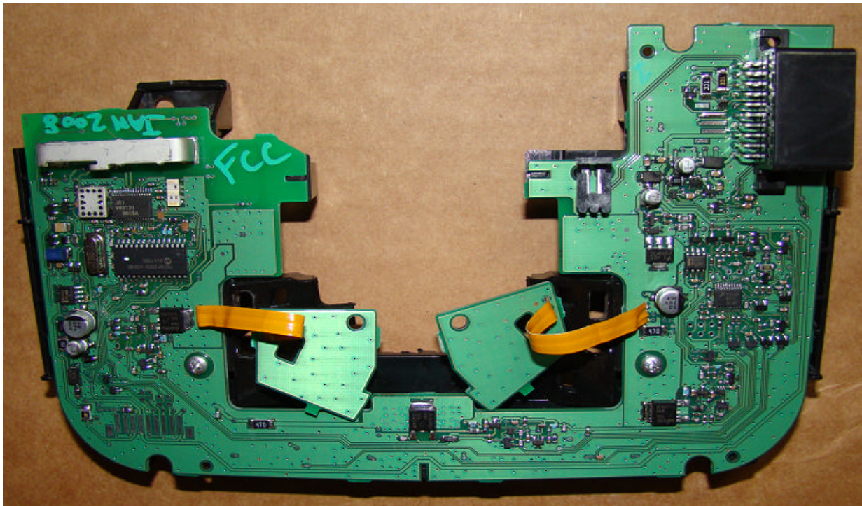
Internal View- Front
