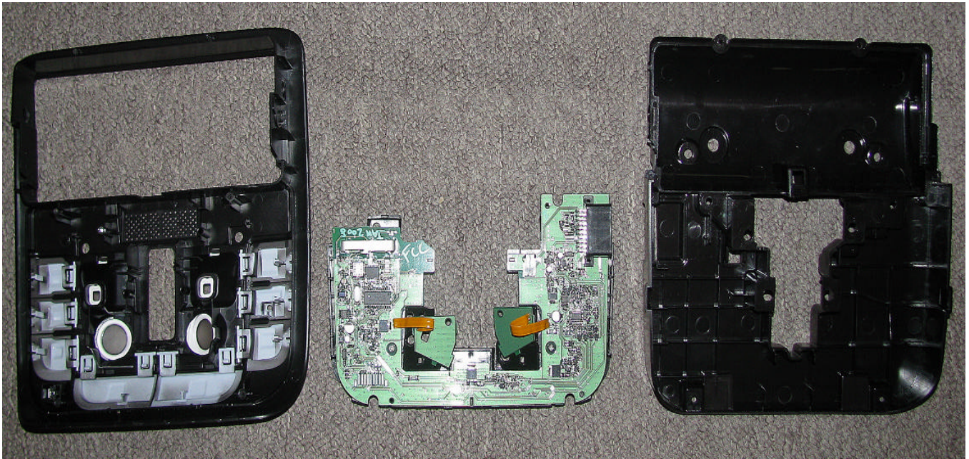
Unit Disassembled View
