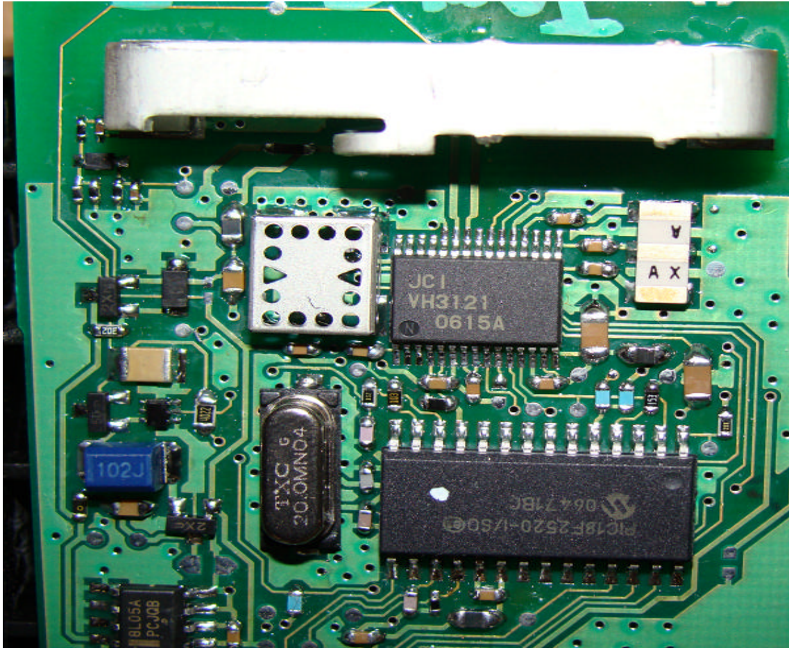
Close-up of Homelink RF
