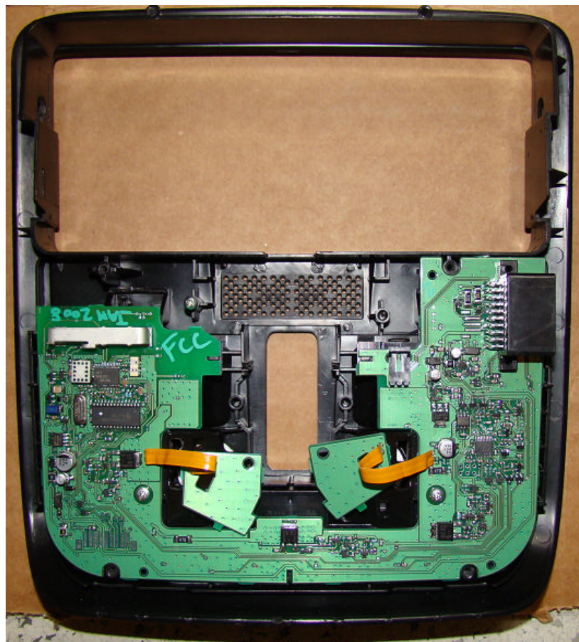
Internal View- Rear
