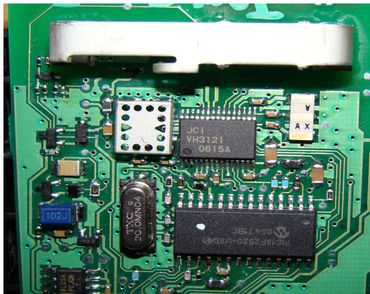
Figure 8.6.3 Close-up of Homelink RF Section.
