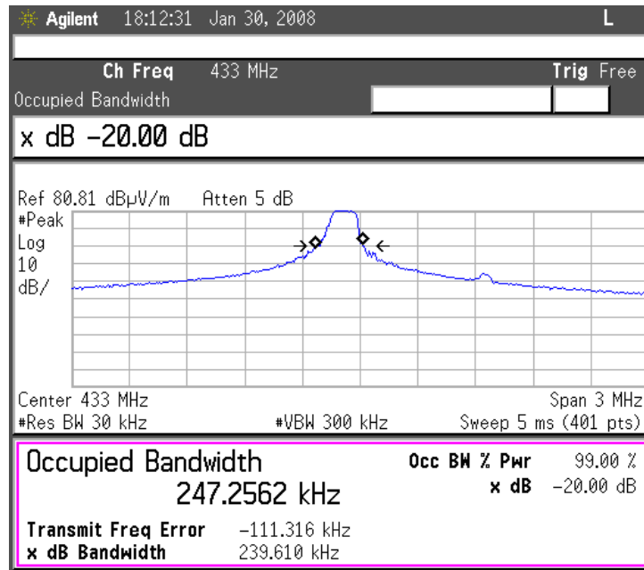
Measuring Occupied Bandwidth at -20dB points [ 433MHz ]
