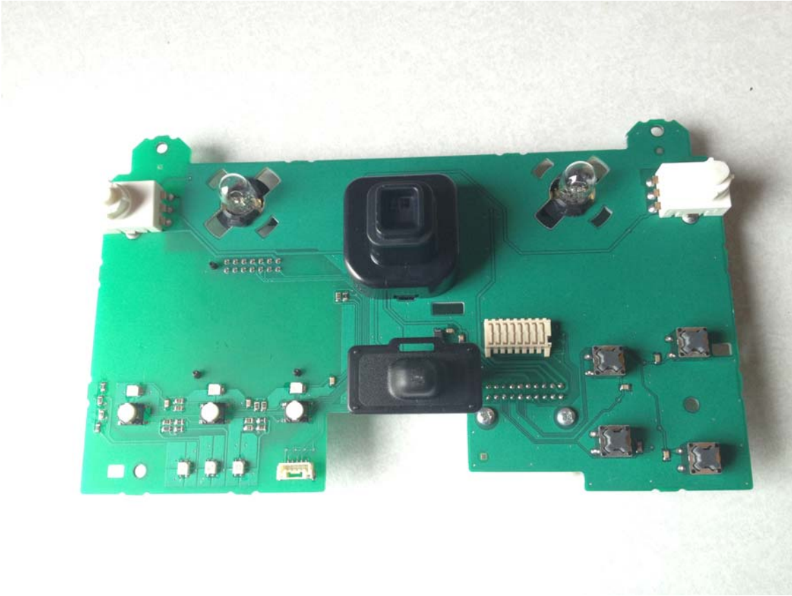
Internal View- Front Lighting Board
