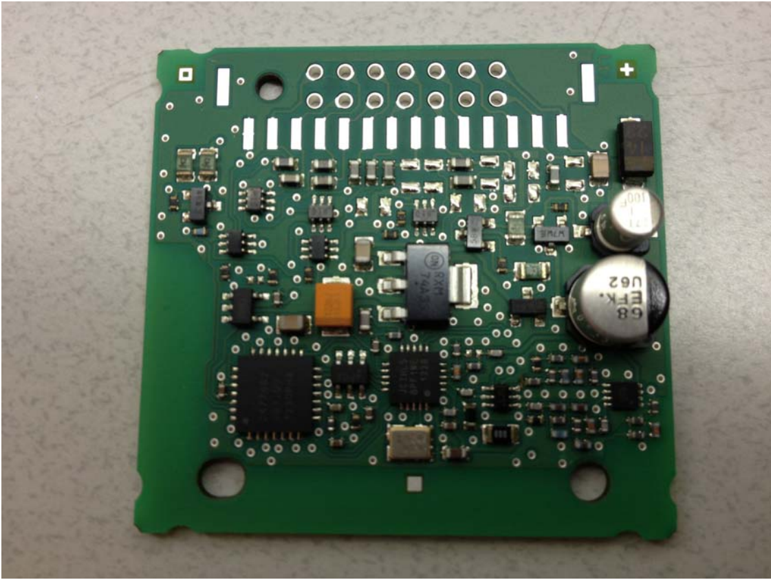
Internal View- Front HomeLink Board
