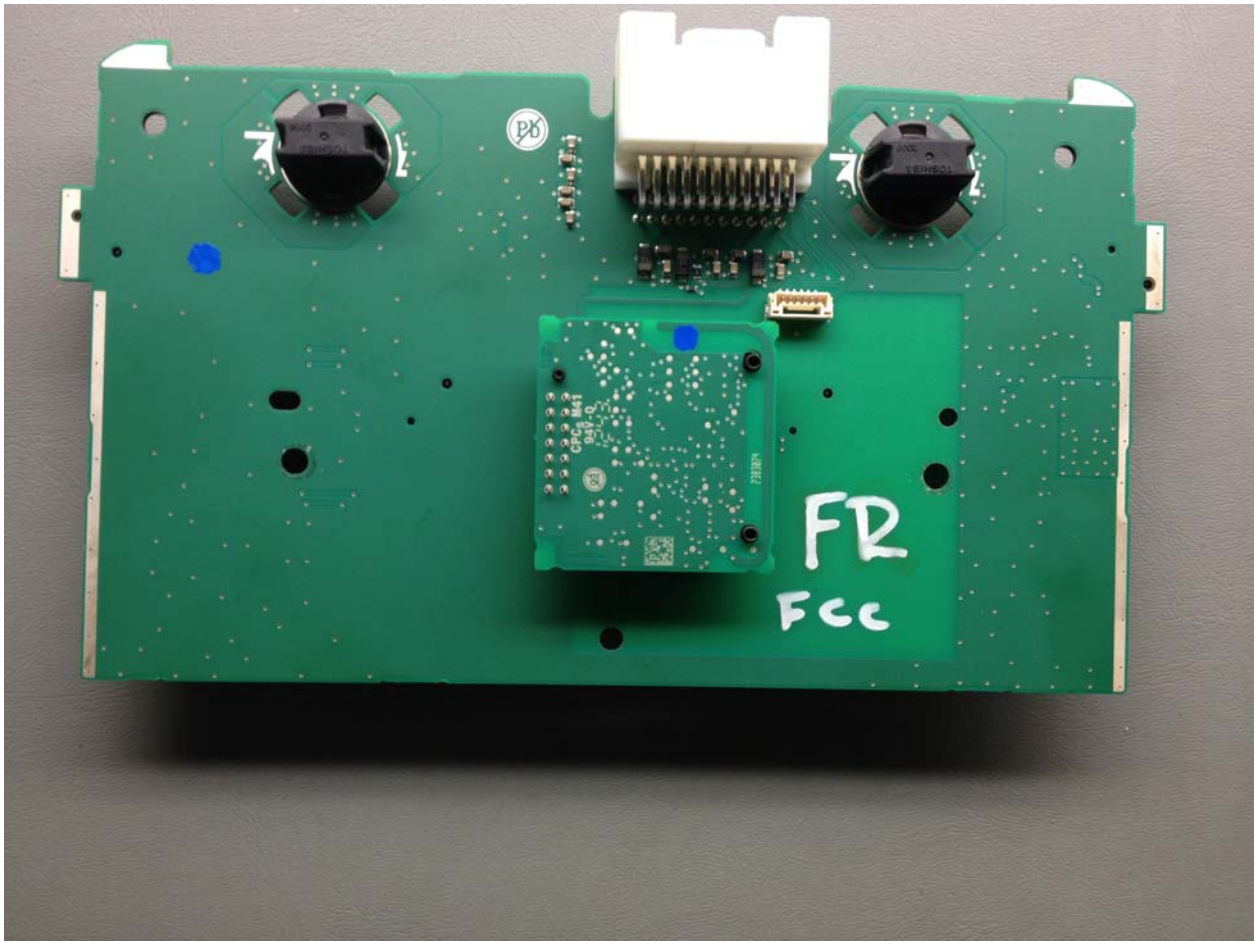
Internal View- Rear PCB side
