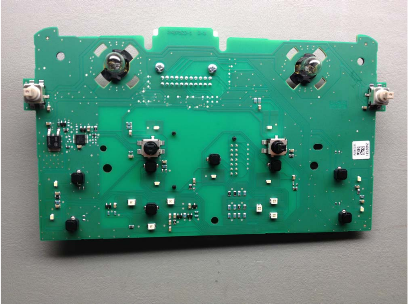
Internal View- Front Lighting Board
