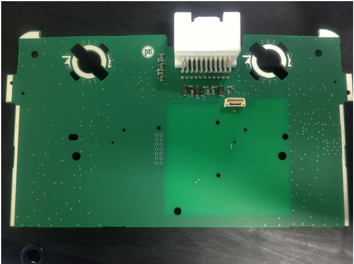
Internal View- Rear Lighting Board
