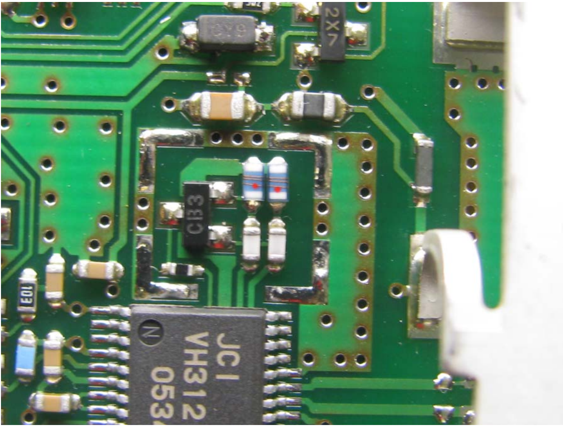
Close-up of Homelink RF shield removed
