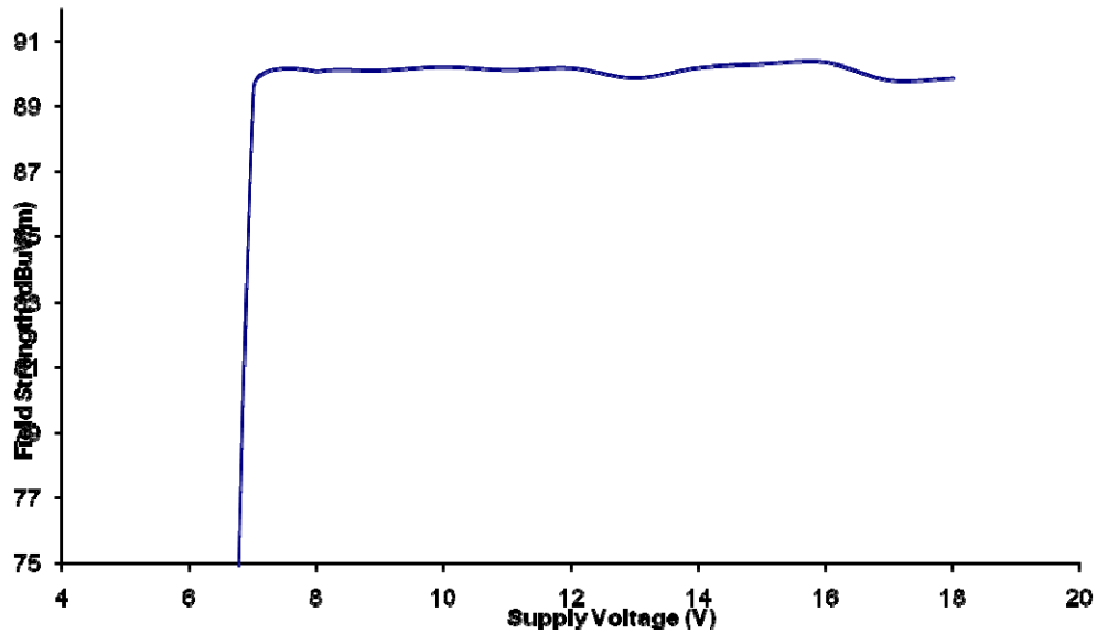
Output Field Strength vs. Supply Voltage
