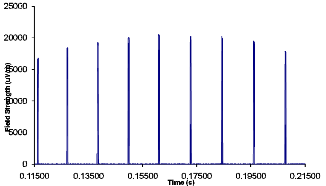
433 MHz, 30 % Duty Cycle Tuning Pulse (100 msec window)
