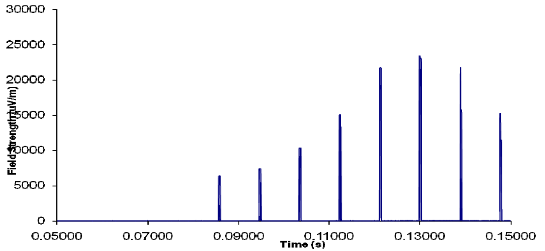
310 MHz, 30 % Duty Cycle Tuning Pulse
