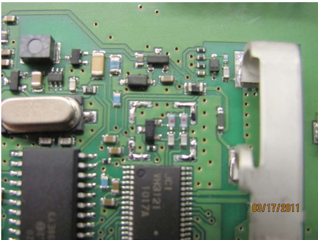
Close-up of Homelink RF shield removed
