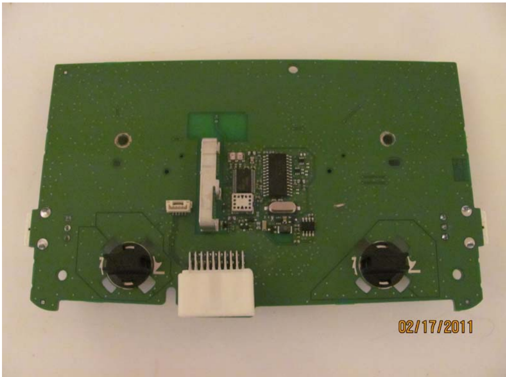
Internal View- Rear
