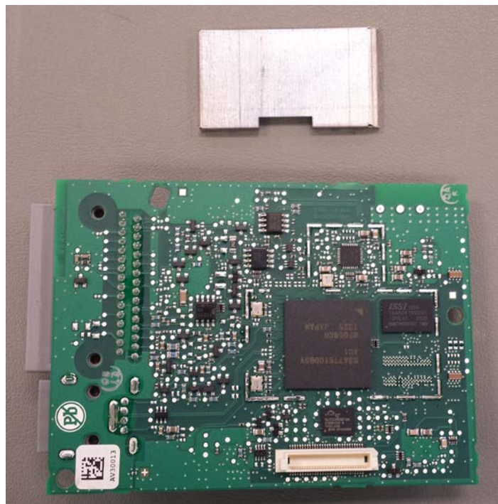
Product Interior – Bottom Side with EMC Shield Removed
