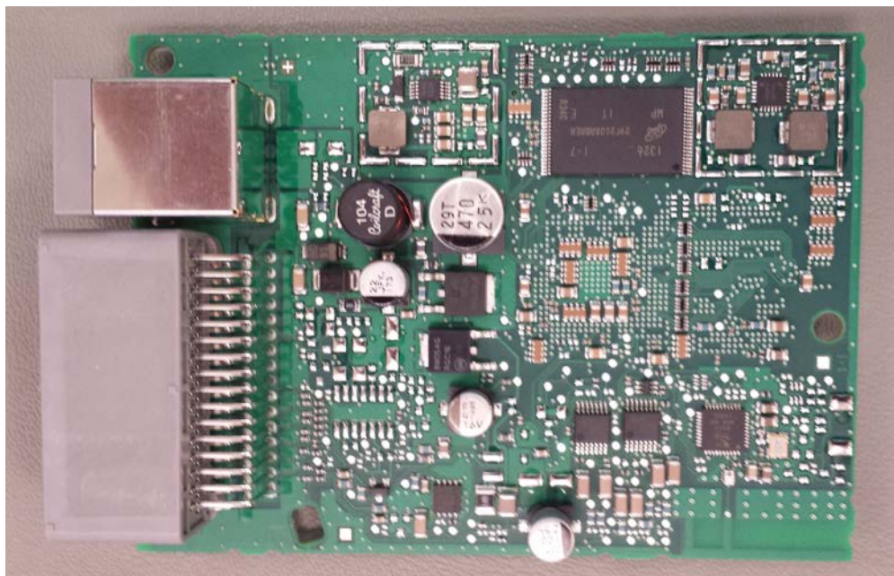
Product Interior – Top Side
