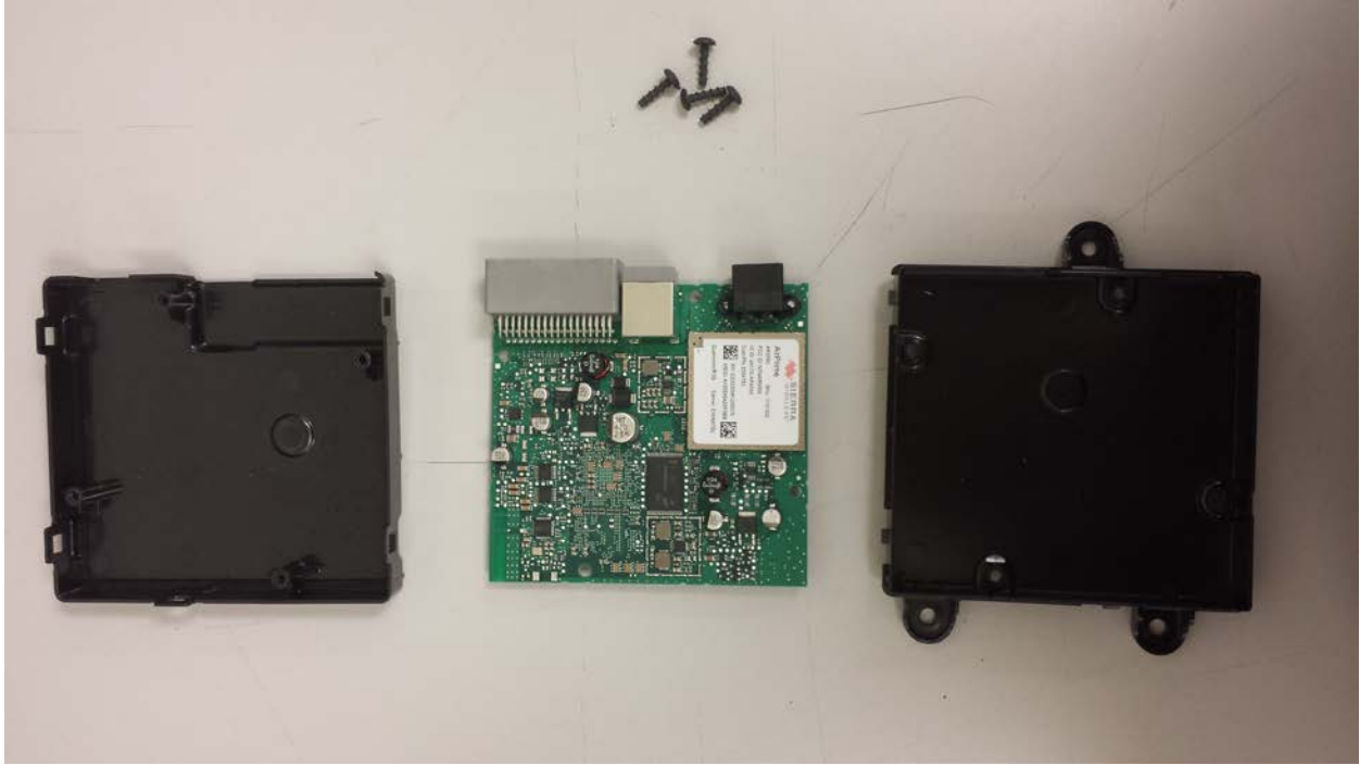
Assembly View
