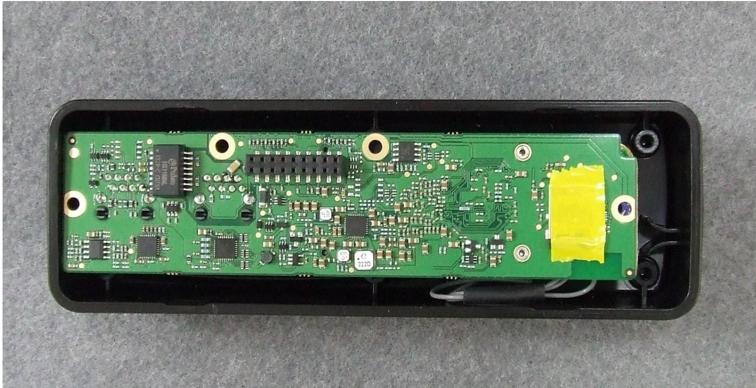
Photograph 04: Rear view
