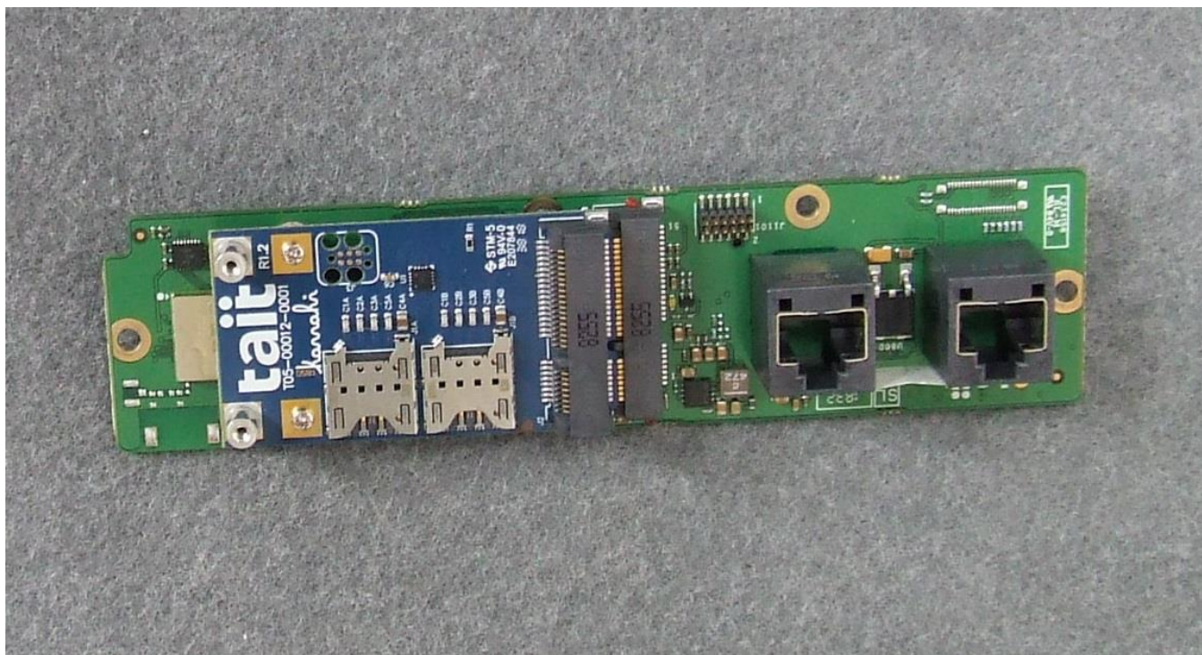
Photograph 10: TUFM4B Dual SIM Interposer connected
