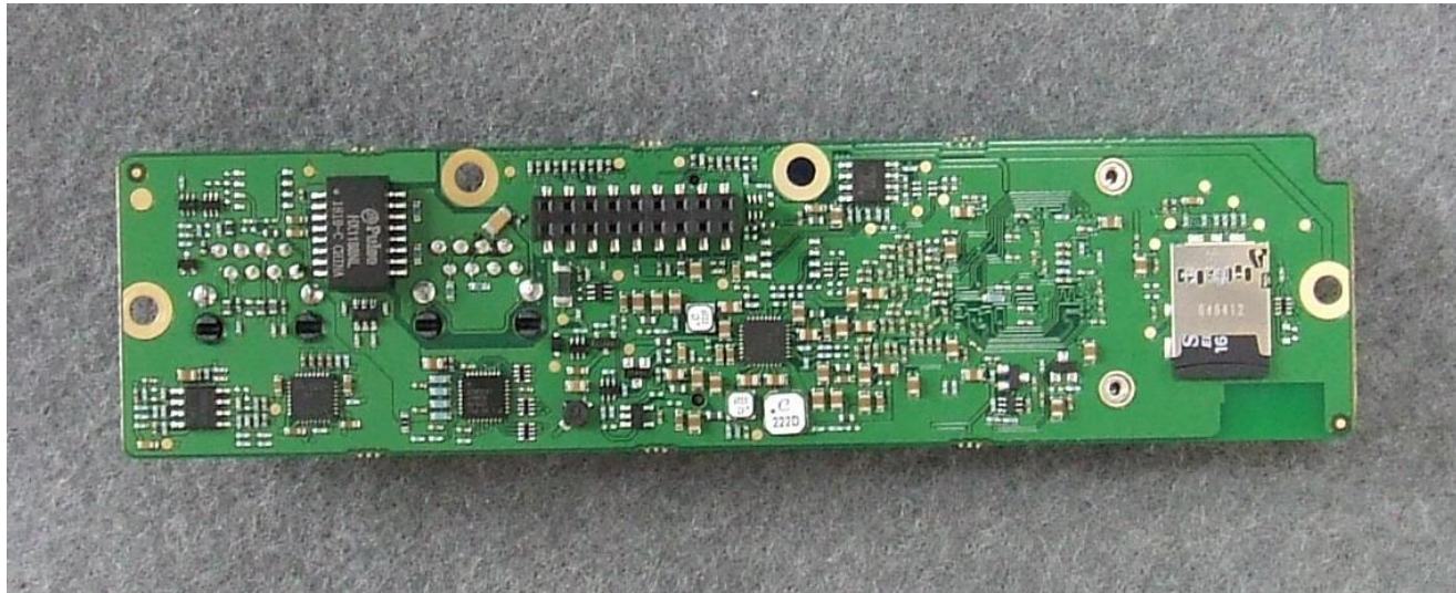
Photograph 03 Backside Main Board (without shields)
