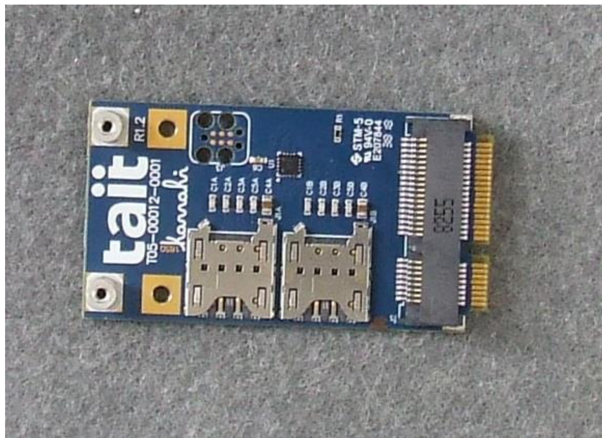
Photograph 11: Front Dual SIM Interposer
