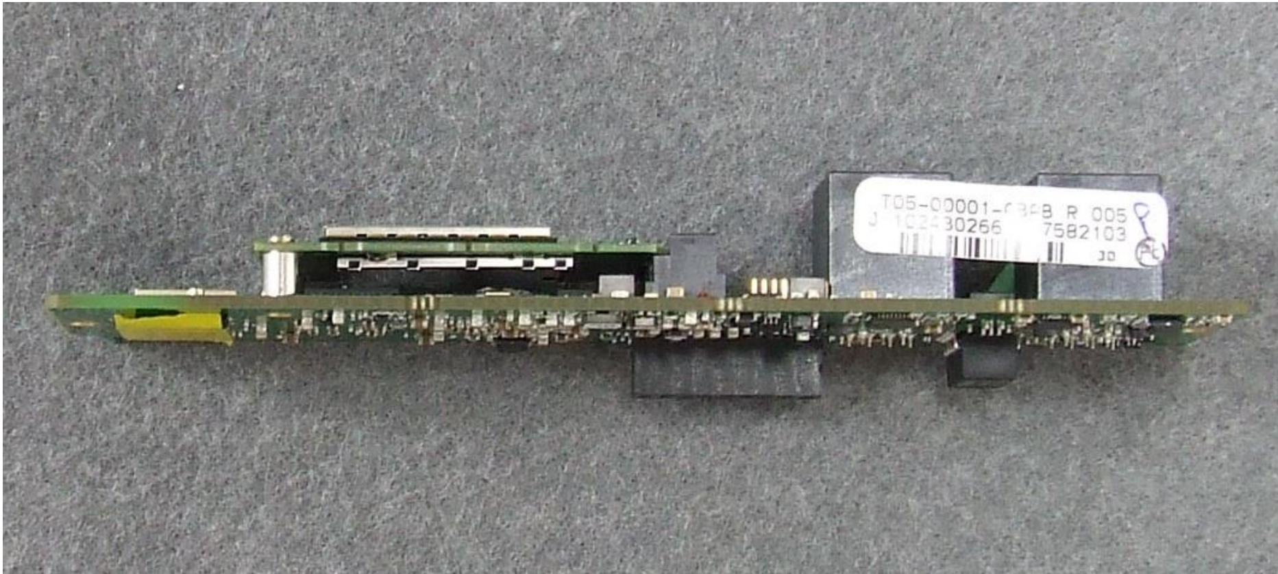
Photograph 07: Side TUFM4B with Dual SIM and Cellular Module
