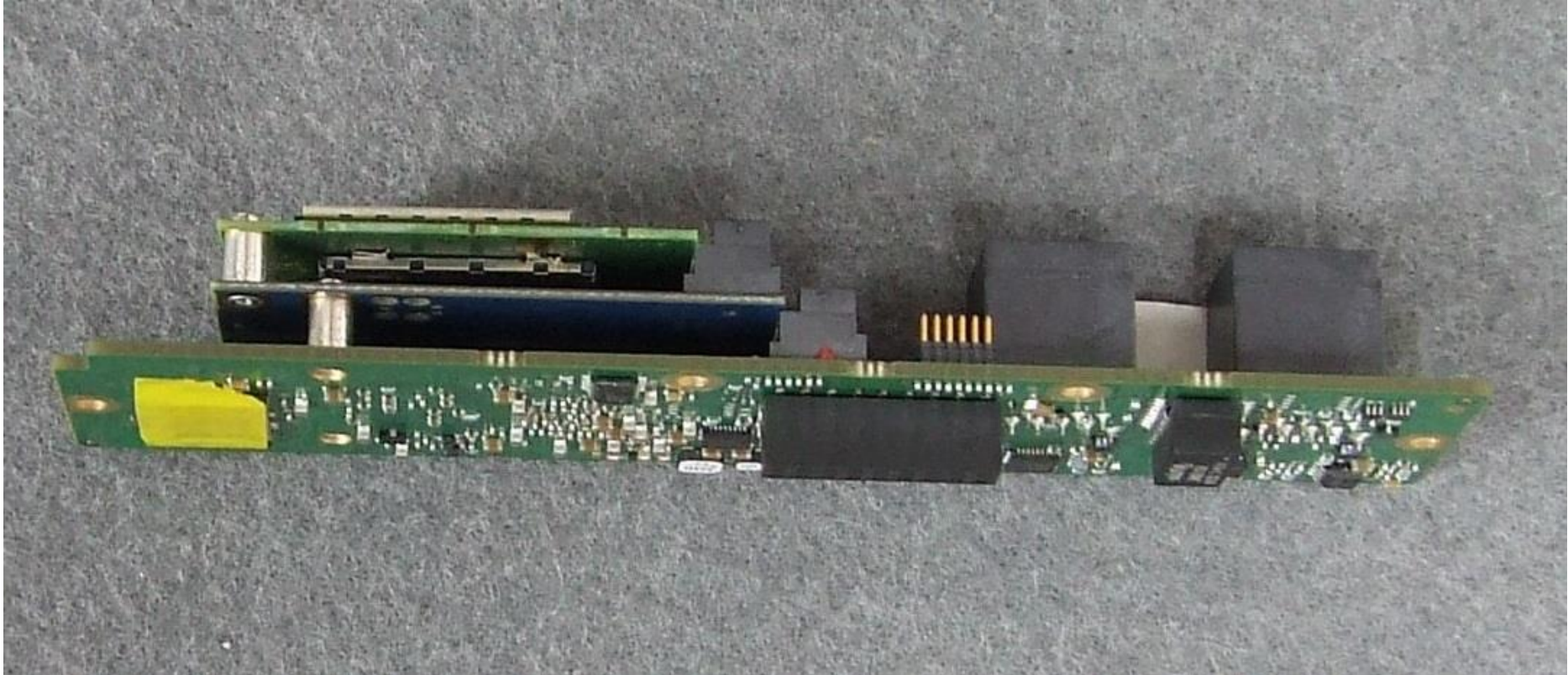
Photograph 05: Side TUFM4B with Dual SIM and Cellular Module
