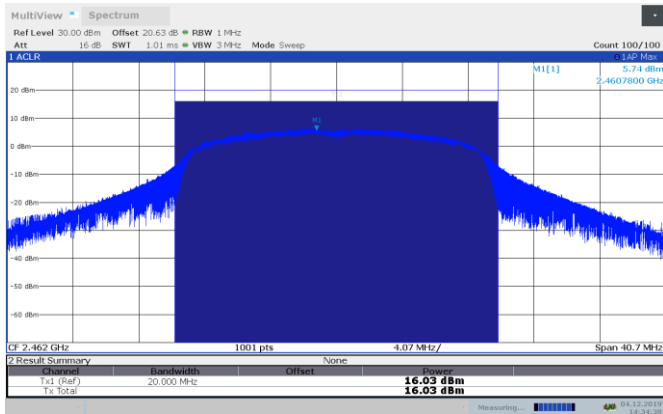
Figure 8.4-1: Conducted output power 802.11b, sample plot
