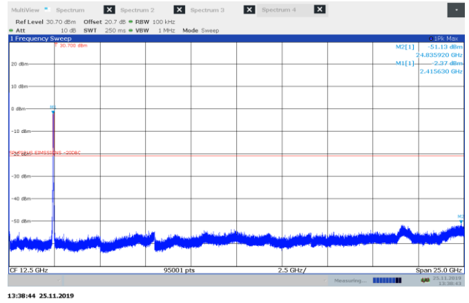
Figure 8.5-10: Conducted spurious emissions for 802.11n 40, low channel
