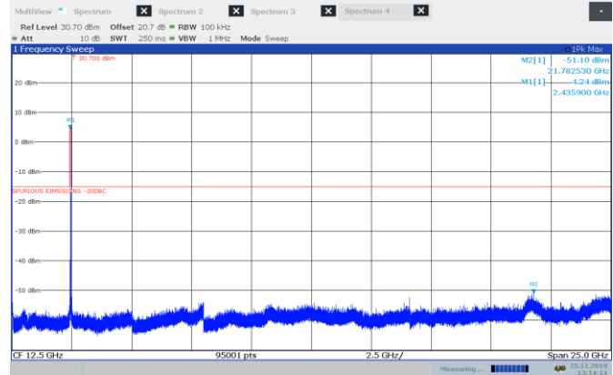
Figure 8.5-2: Conducted spurious emissions for 802.11 b, mid channel
