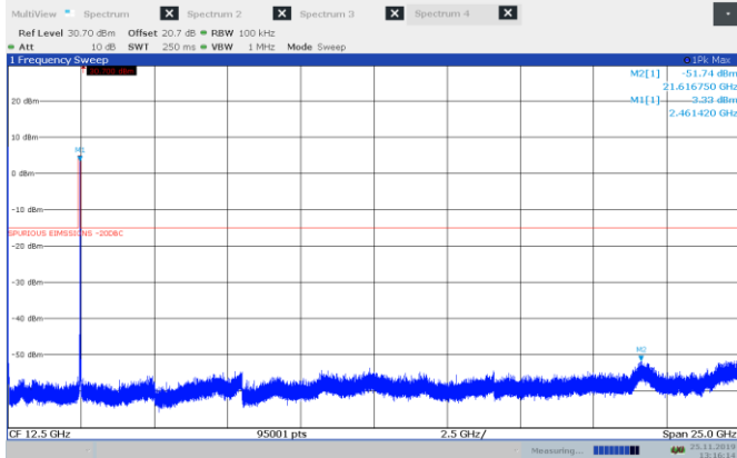
Figure 8.5-3: Conducted spurious emissions for 802.11 b, high channel
