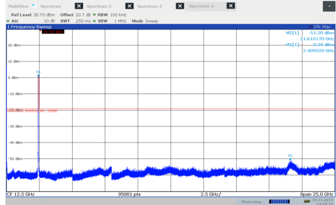
Figure 8.5-4: Conducted spurious emissions for 802.11 g, low channel
