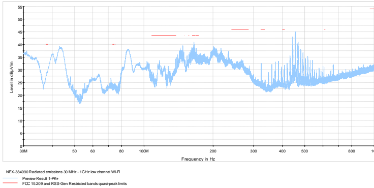
Figure 8.5-13: Radiated spurious emissions below 1 GHz, low channel
