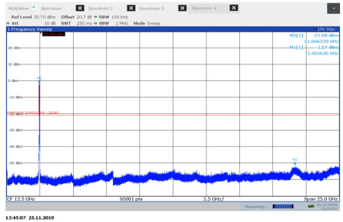
Figure 8.5-12: Conducted spurious emissions for 802.11n 40high channel
