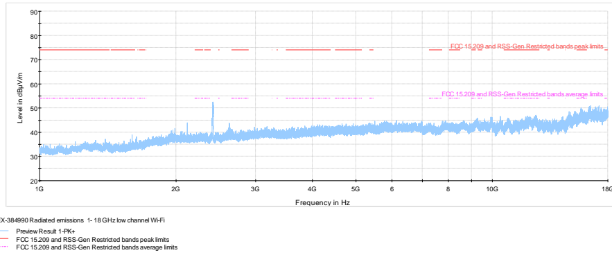
Figure 8.5-16: Radiated spurious emissions within 1–18 GHz, low channel
