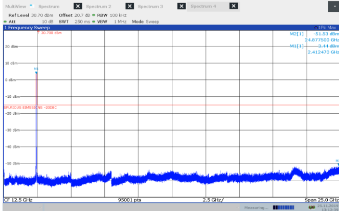
Figure 8.5-1: Conducted spurious emissions for 802.11 b, low channel
