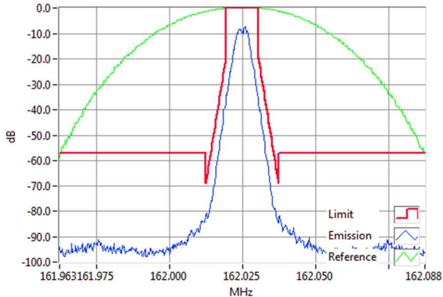
DMR 162.0250MHz Mask D 5W RBW=100Hz, VBW=1000Hz, Detector Mode=Peak Result=Pass
