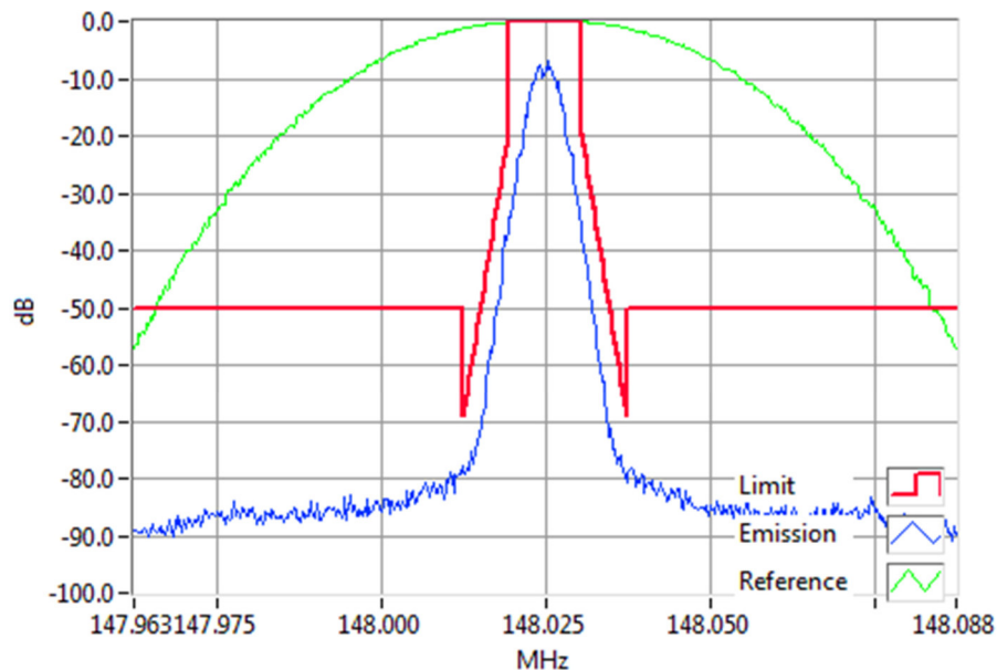
DMR 148.0250MHz Mask D 1W RBW=100Hz, VBW=1000Hz, Detector Mode=Peak Result=Pass
