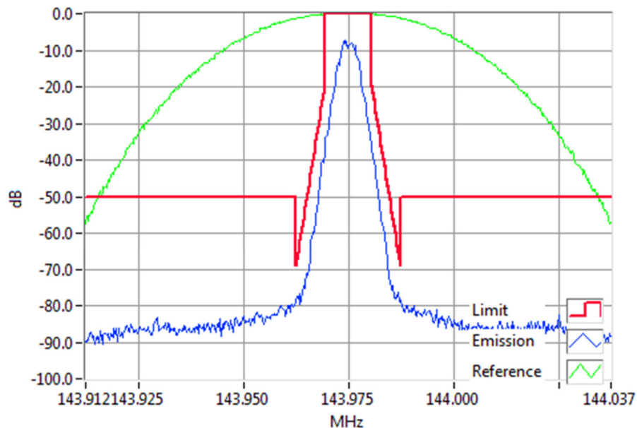
DMR 143.9750MHz Mask D 1W RBW=100Hz, VBW=1000Hz, Detector Mode=Peak Result=Pass
