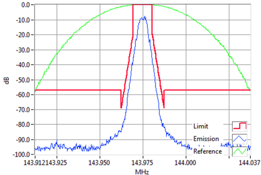
DMR 143.9750MHz Mask D 5W RBW=100Hz, VBW=1000Hz, Detector Mode=Peak Result=Pass
