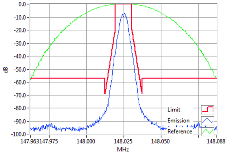
DMR 148.0250MHz Mask D 5W RBW=100Hz, VBW=1000Hz, Detector Mode=Peak Result=Pass
