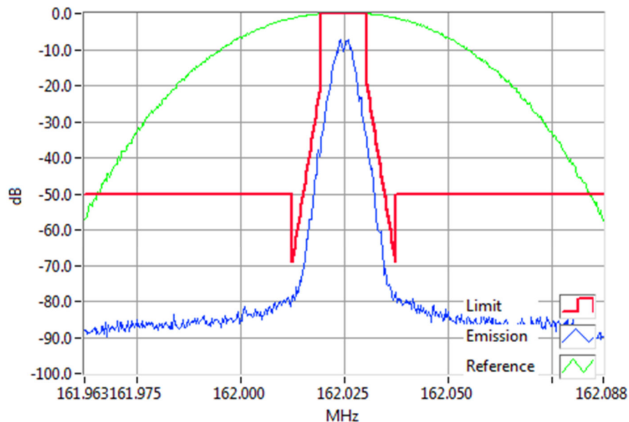
DMR 162.0250MHz Mask D 1W RBW=100Hz, VBW=1000Hz, Detector Mode=Peak Result=Pass
