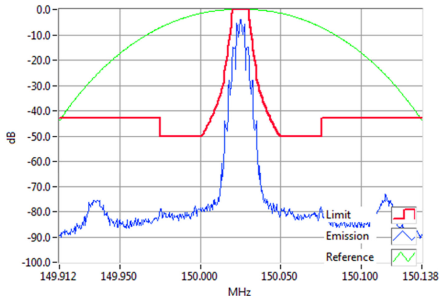
FFSK2400 150.0250MHz Mask C 1W RBW=300Hz, VBW=3000Hz, Detector Mode=Peak Result=Pass
