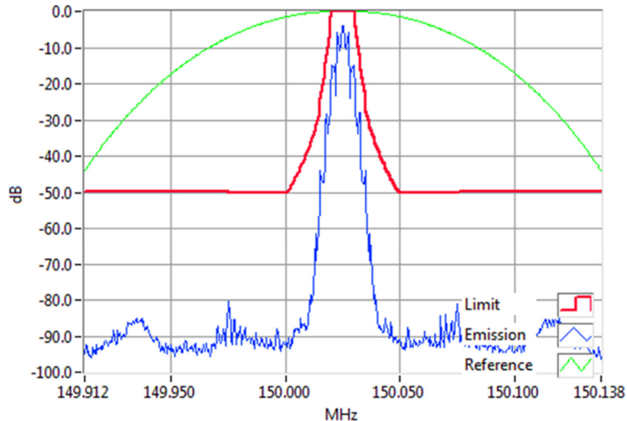
FFSK2400 150.0250MHz Mask C 5W RBW=300Hz, VBW=3000Hz, Detector Mode=Peak Result=Pass
