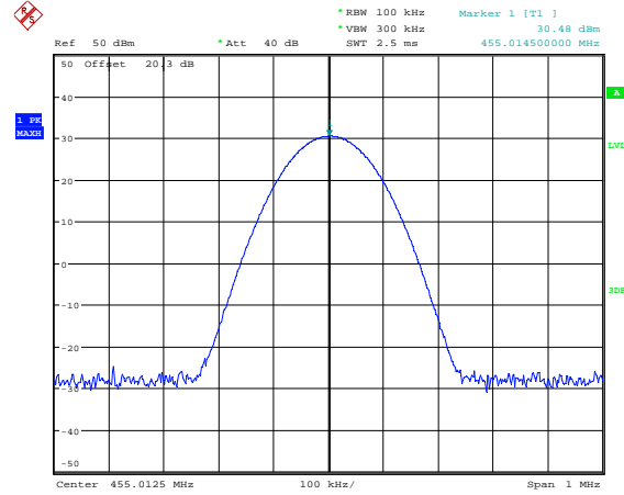
Additional Channel, Part 74, 455.0125 MHz Low Power
