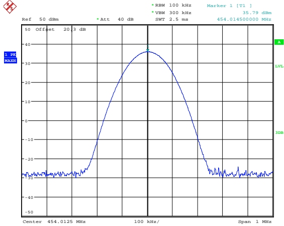
Additional Channel, Part 22, 454.0125 MHz High Power
