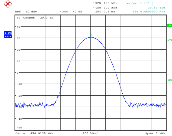
Additional Channel, Part 22, 454.0125 MHz Low Power
