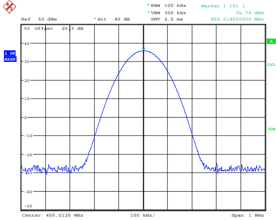
Additional Channel, Part 74, 455.0125 MHz High Power
