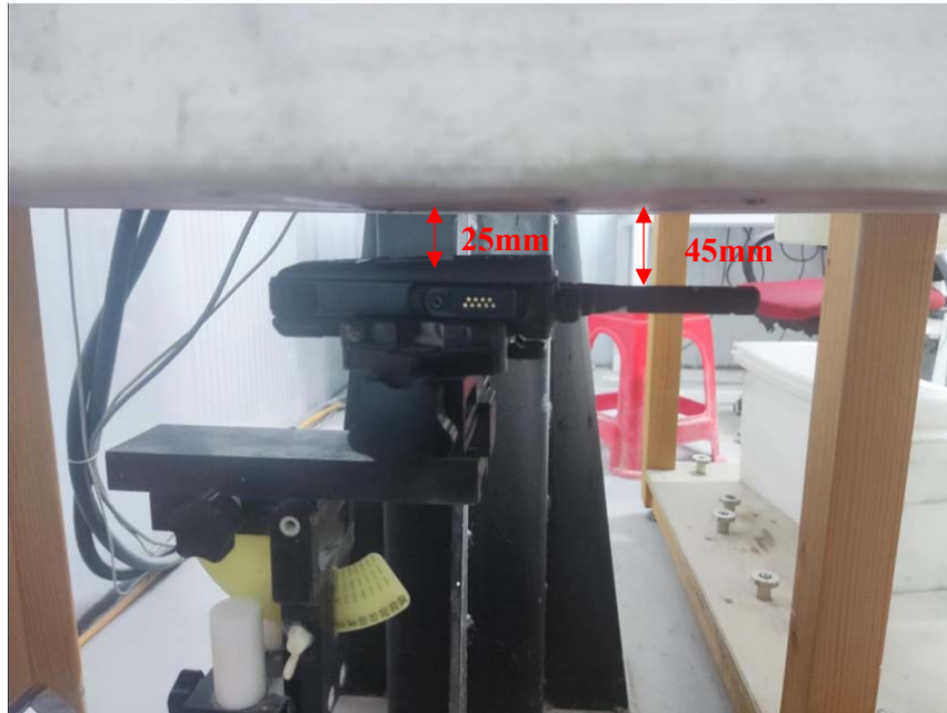
Face Up Setup Photo (25mm)-Antenna 1
