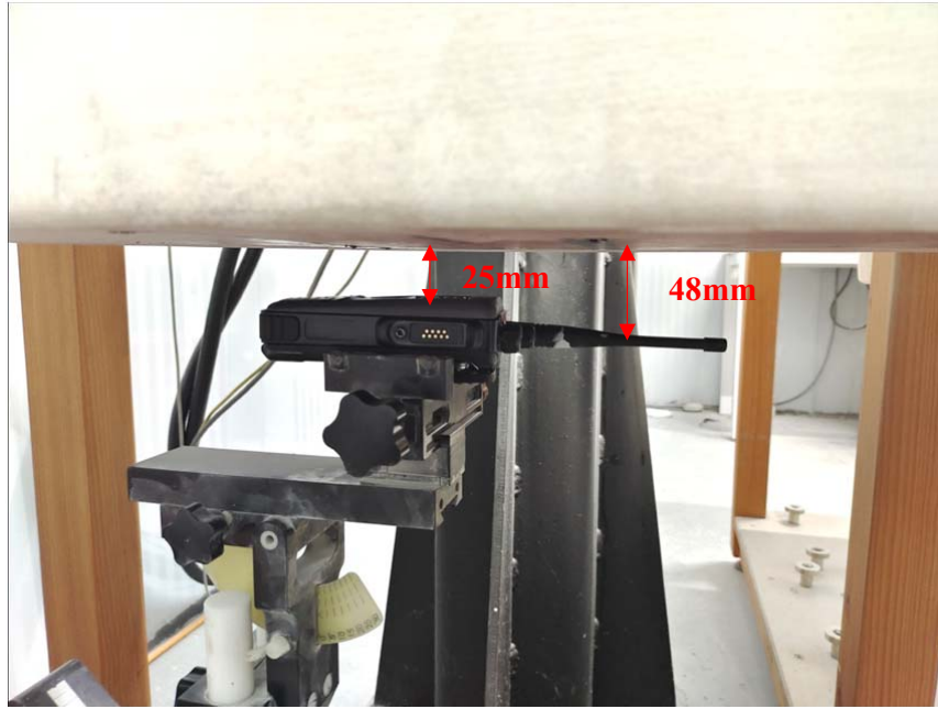
Face Up Setup Photo (25mm) -Antenna 2
