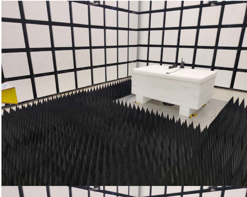
Radiated Emissions Above 1G Rear View-Model: T03-00312-HCDA
