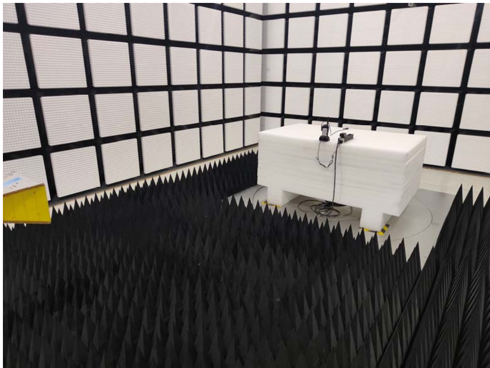
Radiated Emissions Above 1G Rear View-Model: T03-00312-HCDA
