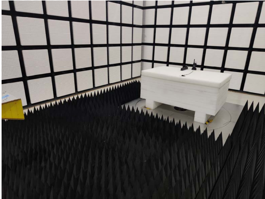
Radiated Emissions Above 1G Rear View-Model: T03-00312-HBAA
