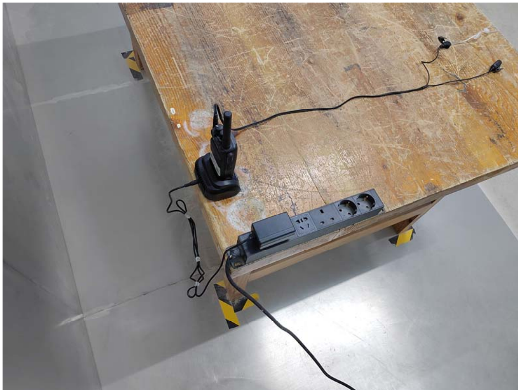
Conducted Emissions Side View-Model: T03-00312-HAAA
