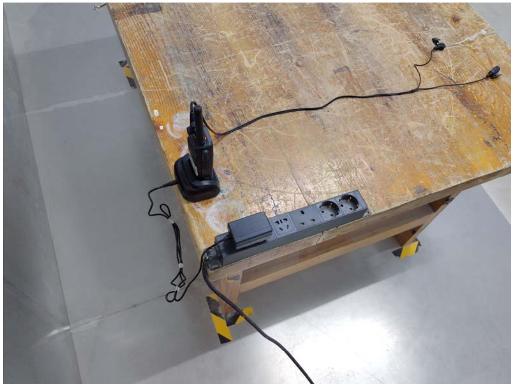
Conducted Emissions Side View-Model: T03-00312-HBAA
