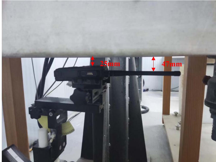
Face Up Setup Photo (25mm)( Long antenna)
