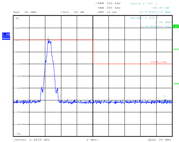
Figure 8.6-11: Conducted spurious emissions at the low upper er band edge for \pi/4 -DQPSK modulation, hopping off
