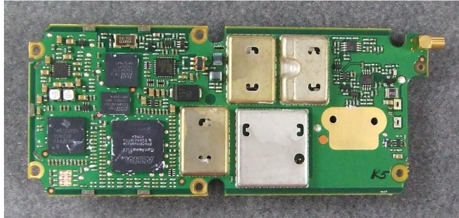
Photograph 04: Rx-Tx PCB - bottom (with shields)
