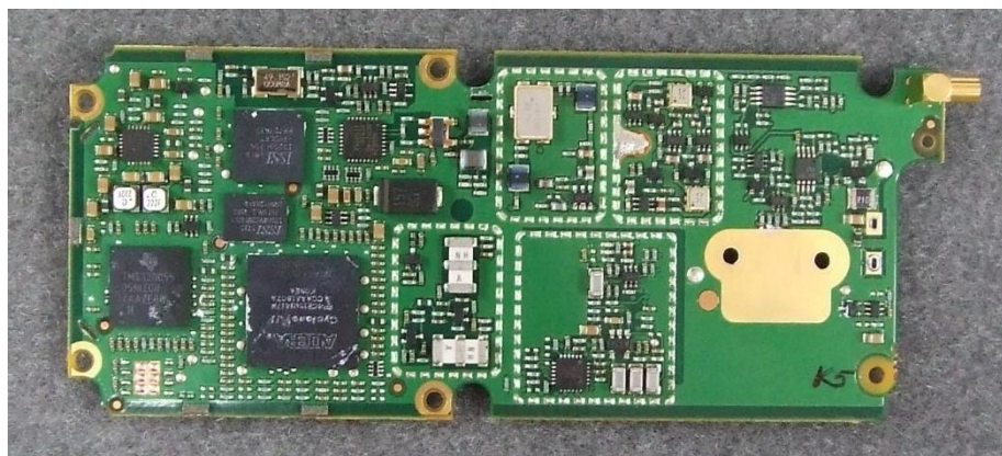
Photograph 05: Rx-Tx PCB - bottom (without shields)
