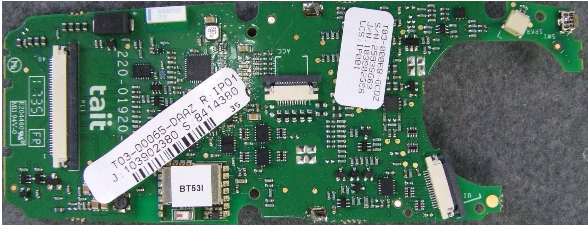
Photograph 06: Control PCB - Bottom
