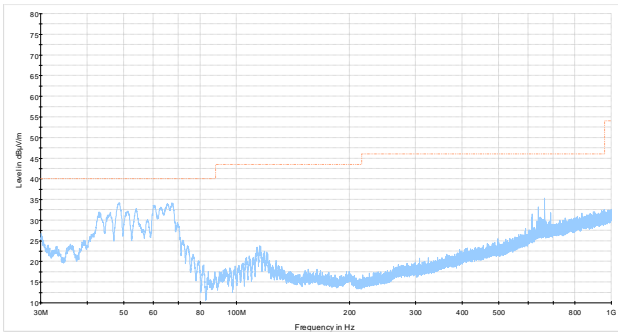
Plot 8.2-3: Radiated spurious emissions on mid channel
