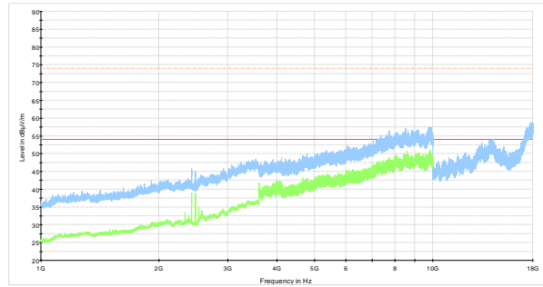
Plot 8.2-6: Radiated spurious emissions on high channel
