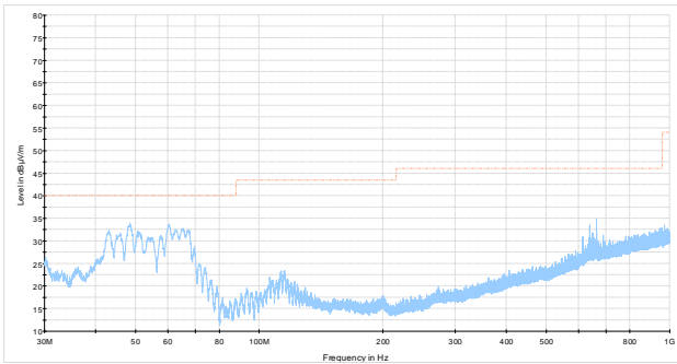
Plot 8.2-5: Radiated spurious emissions on high channel
