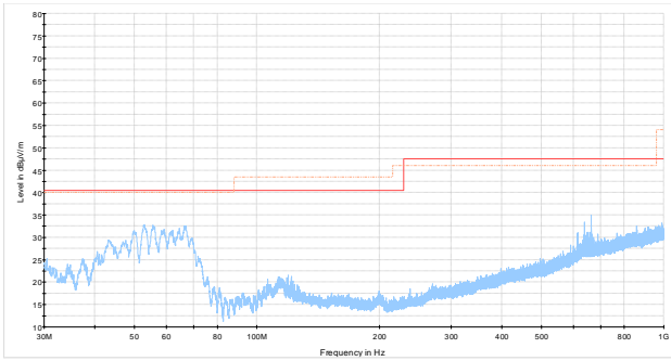
Plot 8.2-1: Radiated spurious emissions on low channel
