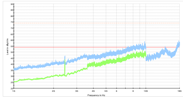
Plot 8.2-2: Radiated spurious emissions on low channel
