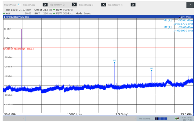
Figure 8.6-16: Conducted spurious emissions for GFSK, mid channel
