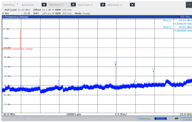
Figure 8.6-17: Conducted spurious emissions for GFSK, high channel
