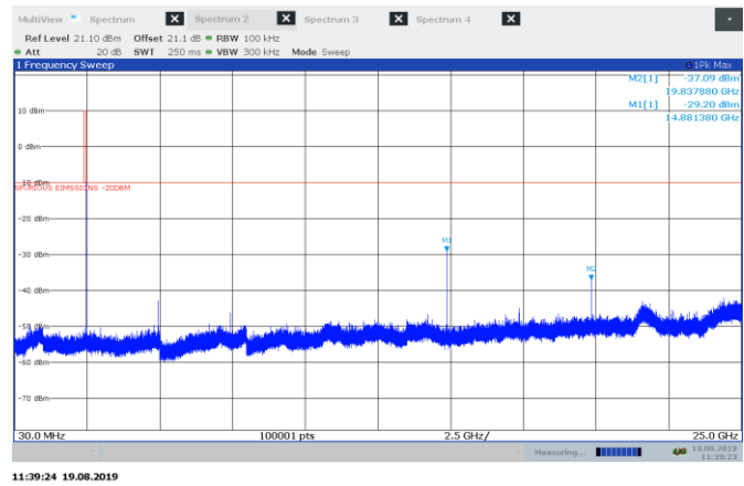
Figure 8.6-26: Conducted spurious emissions for BLE, high channel
