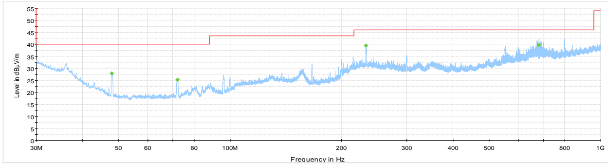
NEX- 379389 Radiated spurious 30 MHz - 1GHz low channel Preview Result 1-PK+ FCC 15.209 and RSS-210 limit line RB Final_Result PK+
