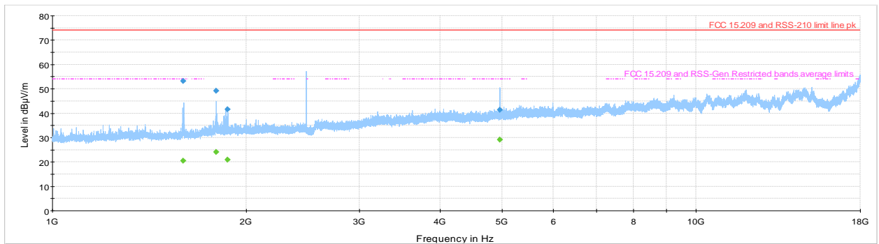
NEX- 379389 Radiated spurious 1 - 18 GHz high channel Preview Result 1-PK+ FCC 15.209 and RSS-210 limit line pk FCC 15.209 and RSS-Gen Restricted bands average limits Final_Result PK+ Final_Result CAV
