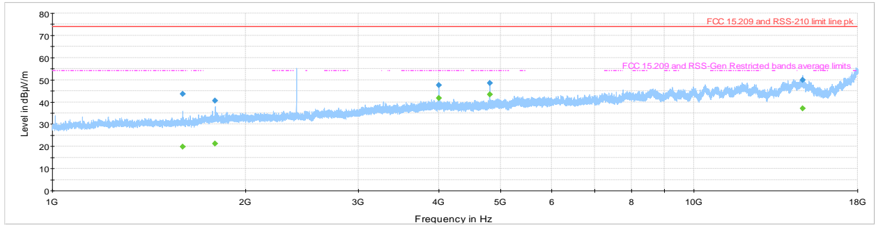
NEX- 379389 Radiated spurious 1 - 18 GHz low channel Preview Result 1-PK+ FCC 15.209 and RSS-210 limit line pk FCC 15.209 and RSS-Gen Restricted bands average limits Final_Result PK+ Final_Result CAV
