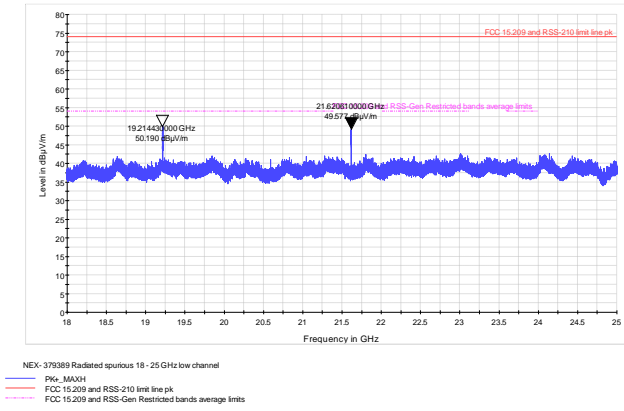
Figure 8.6-33: Radiated spurious emissions above 18 GHz, low channel
