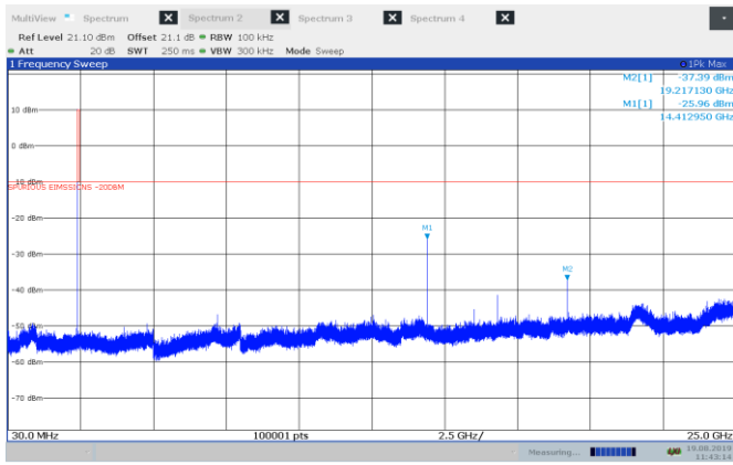
Figure 8.6-15: Conducted spurious emissions for GFSK, low channel
