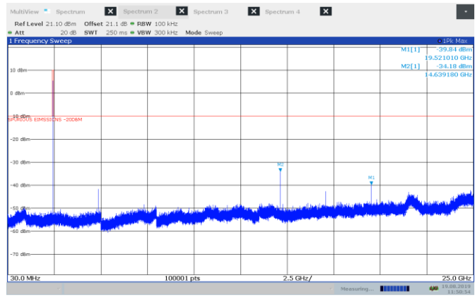
Figure 8.6-18: Conducted spurious emissions for \pi/4 -DQPSK, low channel
