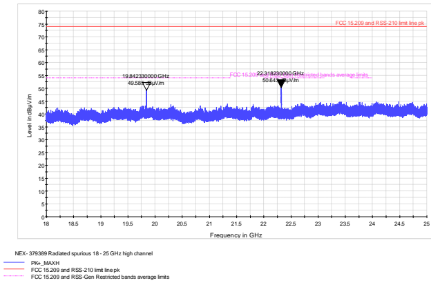
Figure 8.6-35: Radiated spurious emissions above 18 GHz, high channel
