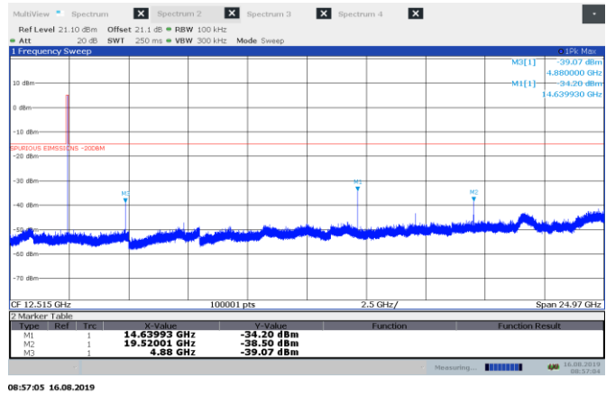
Figure 8.6-22: Conducted spurious emissions for 8DPSK, mid channel
