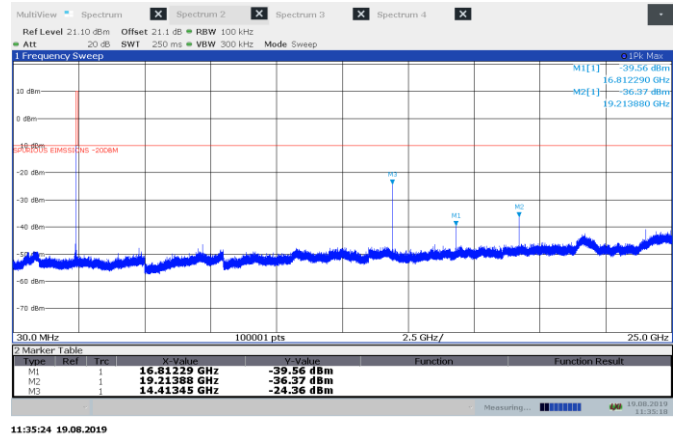
Figure 8.6-24: Conducted spurious emissions for BLE, low channel
