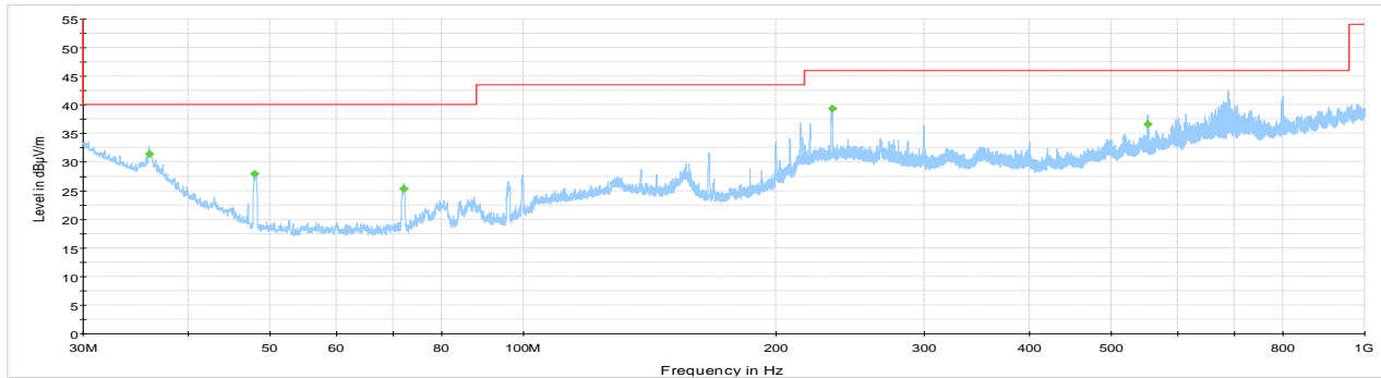
NEX- 379389 Radiated spurious 30 MHz - 1GHz mid channel Preview Result 1-PK+ FCC 15.209 and RSS-210 limit line RB Final_Result PK+
