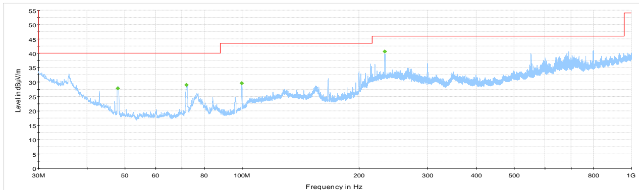
NEX- 379389 Radiated spurious 30 MHz - 1GHz high channel Preview Result 1-PK+ FCC 15.209 and RSS-210 limit line RB Final_Result PK+
