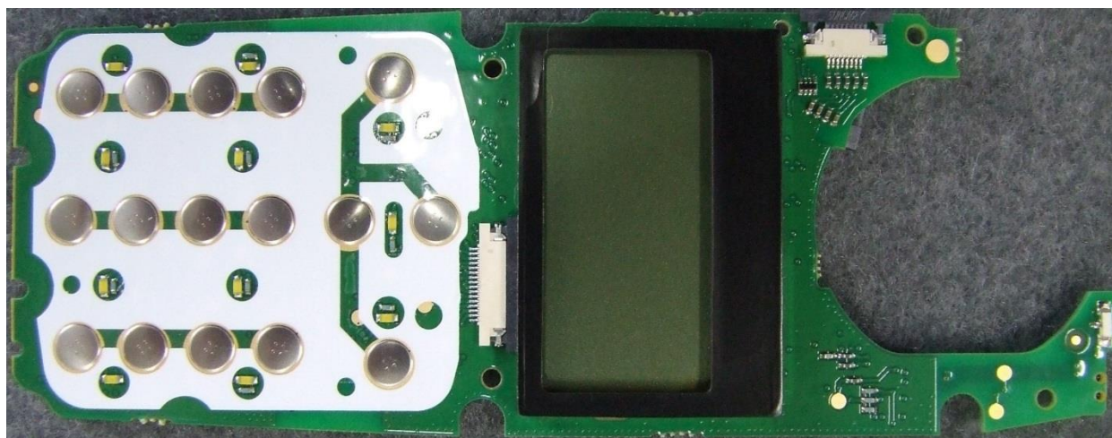
Photograph 05: Control PCB – top
