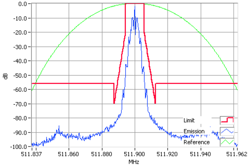
FFSK 1200 bps 511.9000MHz Mask D 4W RBW=100Hz, VBW=1000Hz, Detector Mode=Peak Result=Pass
