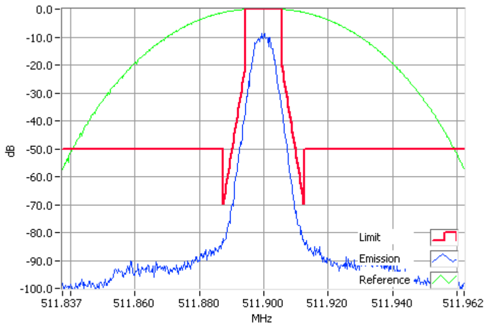
P25 Phase 2 511.9000MHz Mask D 1W RBW=100Hz, VBW=1000Hz, Detector Mode=Peak Result=Pass
