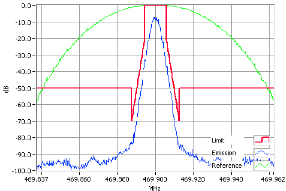
P25 Phase 1 469.9000MHz Mask D 1W RBW=100Hz, VBW=1000Hz, Detector Mode=Peak Result=Pass
