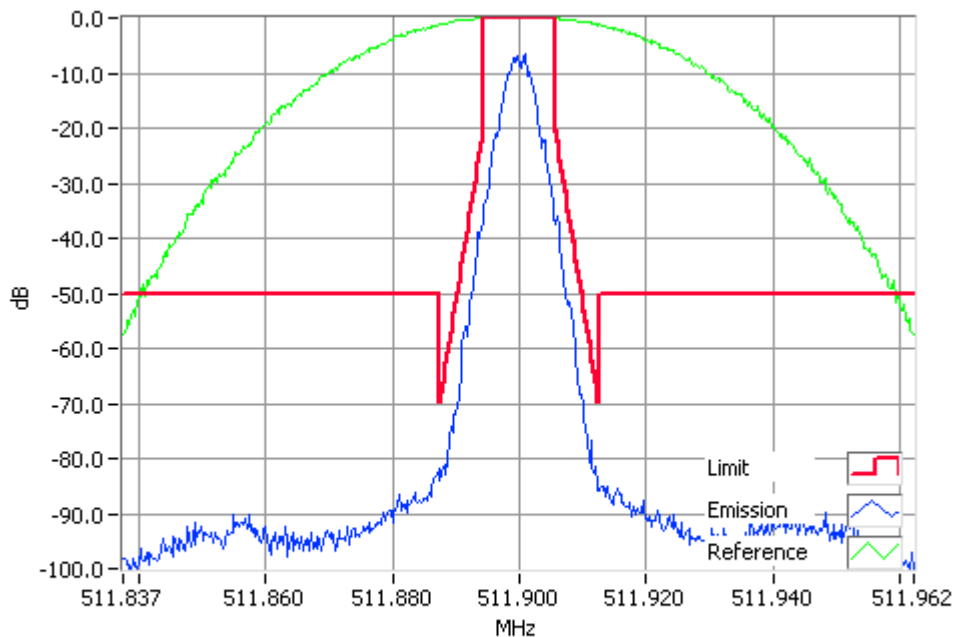
P25 Phase 1 511.9000MHz Mask D 1W RBW=100Hz, VBW=1000Hz, Detector Mode=Peak Result=Pass
