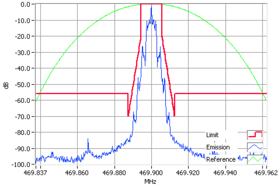
FFSK 2400 bps 469.9000MHz Mask D 4W RBW=100Hz, VBW=1000Hz, Detector Mode=Peak Result=Pass
