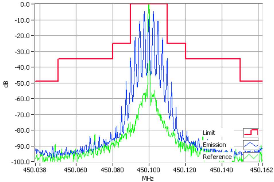
Analogue Modulation 450.1000MHz Mask B 4W RBW=300Hz, VBW=3000Hz, Detector Mode=Peak Result=Pass
