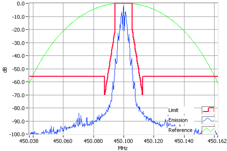
FFSK 1200 bps 450.1000MHz Mask D 4W RBW=100Hz, VBW=1000Hz, Detector Mode=Peak Result=Pass
