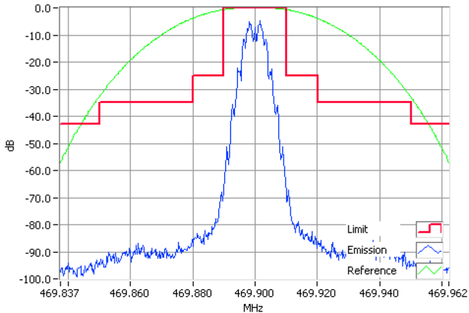
FFSK 1200 bps 469.9000MHz Mask B 1W RBW=300Hz, VBW=3000Hz, Detector Mode=Peak Result=Pass
