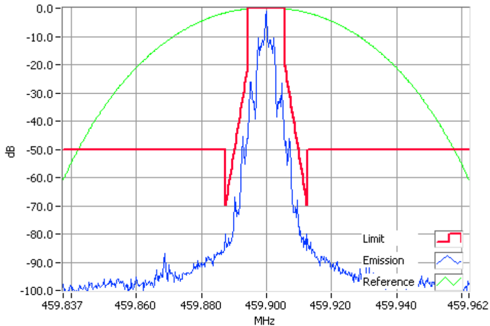
FFSK 2400 bps 459.9000MHz Mask D 1W RBW=100Hz, VBW=1000Hz, Detector Mode=Peak Result=Pass
