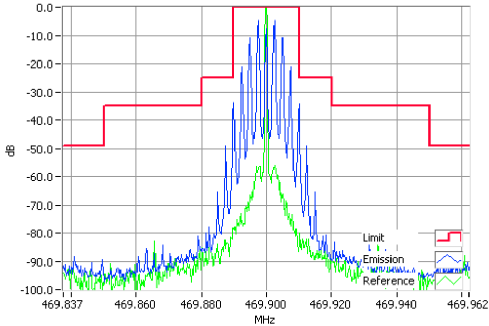
Analogue Modulation 469.9000MHz Mask B 4W RBW=300Hz, VBW=3000Hz, Detector Mode=Peak Result=Pass
