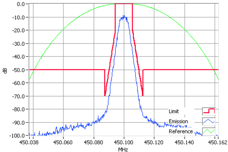
P25 Phase 2 450.1000MHz Mask D 1W RBW=100Hz, VBW=1000Hz, Detector Mode=Peak Result=Pass
