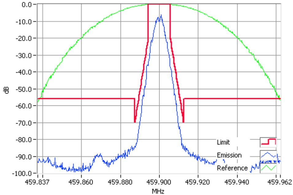
P25 Phase 1 459.9000MHz Mask D 4W RBW=100Hz, VBW=1000Hz, Detector Mode=Peak Result=Pass
