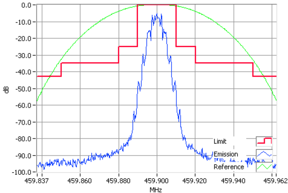
FFSK 2400 bps 459.9000MHz Mask B 1W RBW=300Hz, VBW=3000Hz, Detector Mode=Peak Result=Pass
