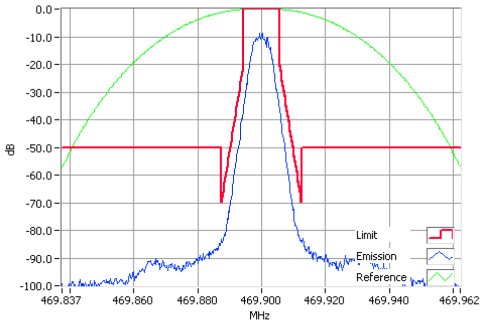
P25 Phase 2 469.9000MHz Mask D 1W RBW=100Hz, VBW=1000Hz, Detector Mode=Peak Result=Pass
