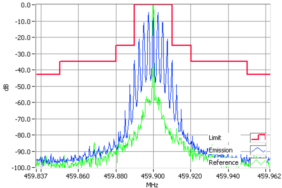
Analogue Modulation 459.9000MHz Mask B 1W RBW=300Hz, VBW=3000Hz, Detector Mode=Peak Result=Pass
