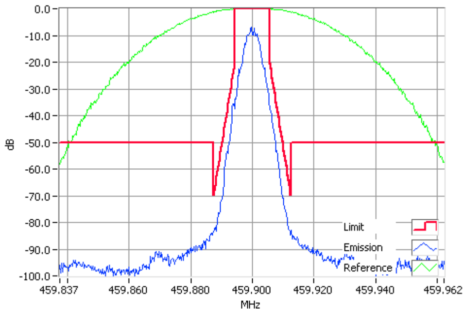
P25 Phase 1 459.9000MHz Mask D 1W RBW=100Hz, VBW=1000Hz, Detector Mode=Peak Result=Pass
