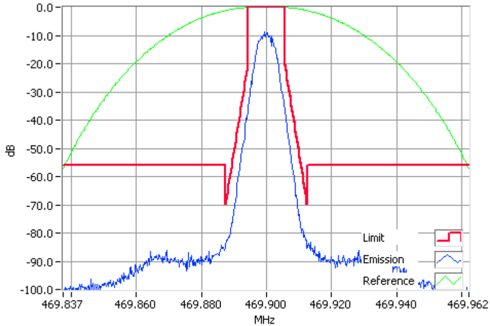
P25 Phase 2 469.9000MHz Mask D 4W RBW=100Hz, VBW=1000Hz, Detector Mode=Peak Result=Pass
