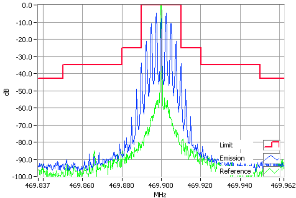
Analogue Modulation 469.9000MHz Mask B 1W RBW=300Hz, VBW=3000Hz, Detector Mode=Peak Result=Pass
