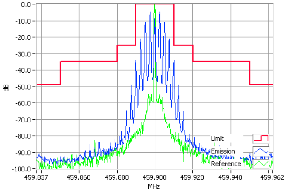
Analogue Modulation 459.9000MHz Mask B 4W RBW=300Hz, VBW=3000Hz, Detector Mode=Peak Result=Pass
