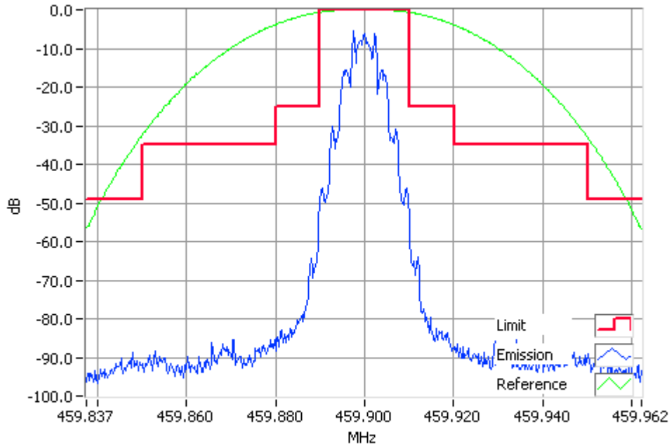
FFSK 2400 bps 459.9000MHz Mask B 4W RBW=300Hz, VBW=3000Hz, Detector Mode=Peak Result=Pass
