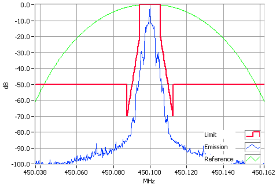
FFSK 2400 bps 450.1000MHz Mask D 1W RBW=100Hz, VBW=1000Hz, Detector Mode=Peak Result=Pass
