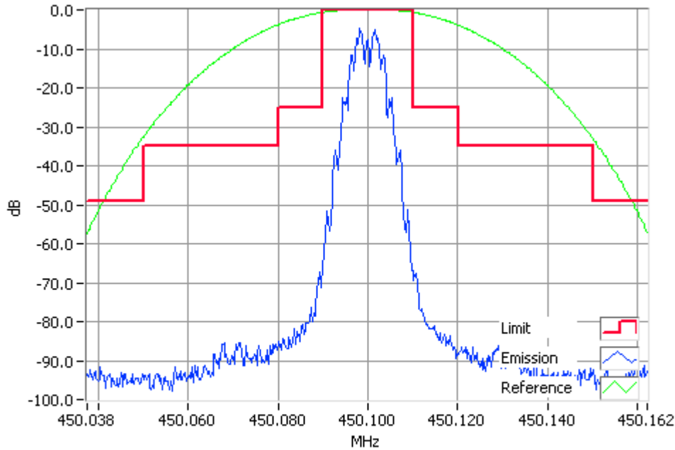
FFSK 1200 bps 450.1000MHz Mask B 4W RBW=300Hz, VBW=3000Hz, Detector Mode=Peak Result=Pass
