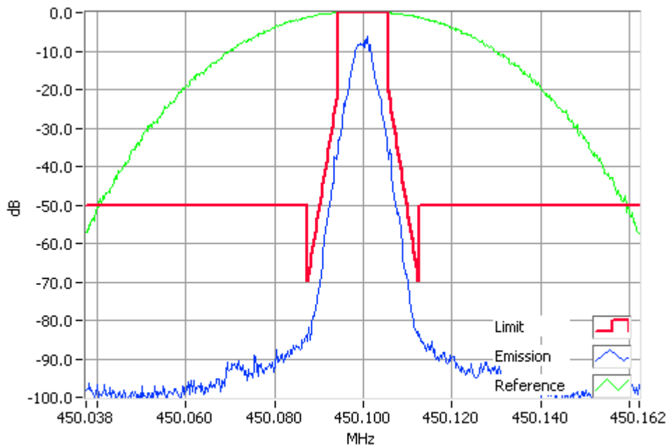
P25 Phase 1 450.1000MHz Mask D 1W RBW=100Hz, VBW=1000Hz, Detector Mode=Peak Result=Pass
