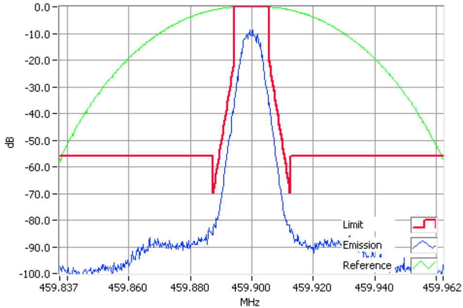
P25 Phase 2 459.9000MHz Mask D 4W RBW=100Hz, VBW=1000Hz, Detector Mode=Peak Result=Pass
