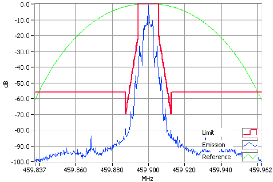
FFSK 2400 bps 459.9000MHz Mask D 4W RBW=100Hz, VBW=1000Hz, Detector Mode=Peak Result=Pass
