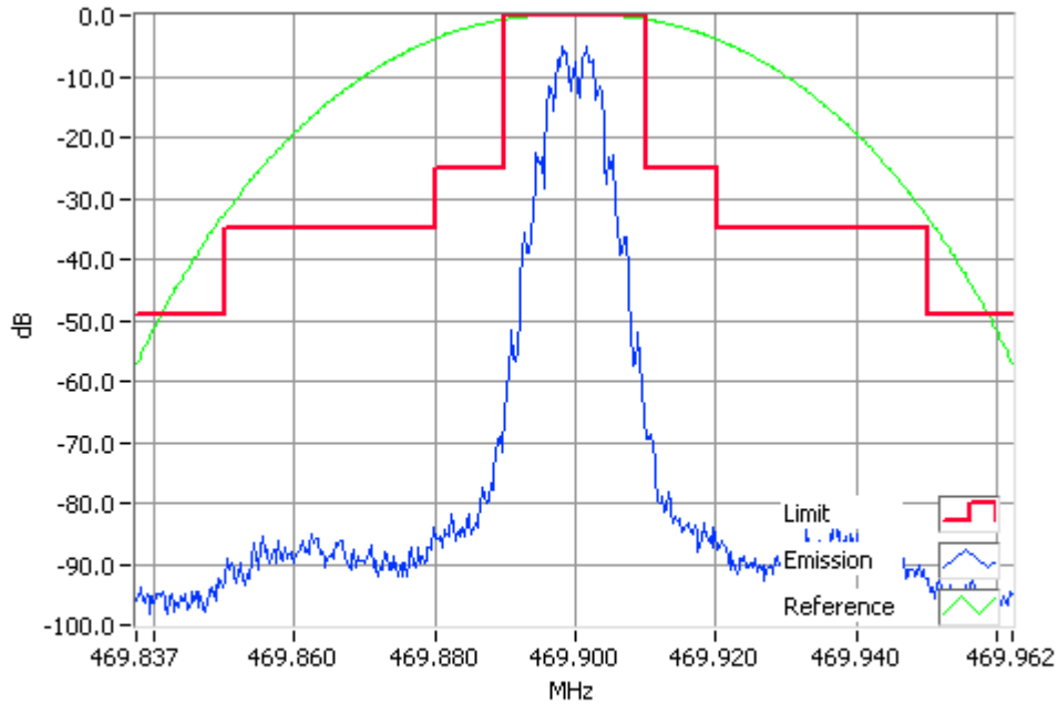
FFSK 1200 bps 469.9000MHz Mask B 4W RBW=300Hz, VBW=3000Hz, Detector Mode=Peak Result=Pass
