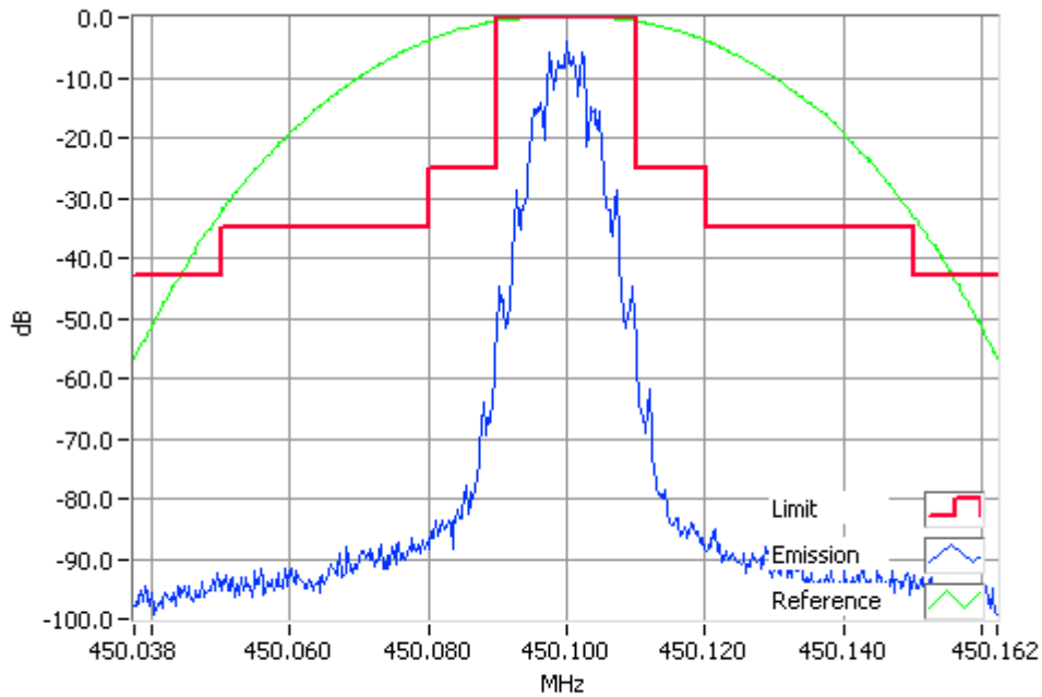
FFSK 2400 bps 450.1000MHz Mask B 1W RBW=300Hz, VBW=3000Hz, Detector Mode=Peak Result=Pass
