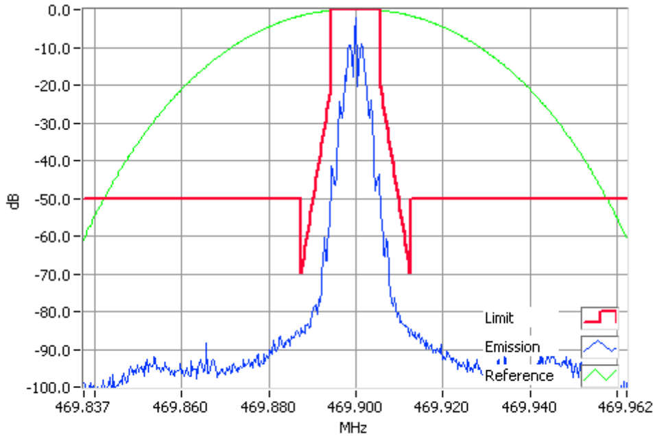
FFSK 1200 bps 469.9000MHz Mask D 1W RBW=100Hz, VBW=1000Hz, Detector Mode=Peak Result=Pass
