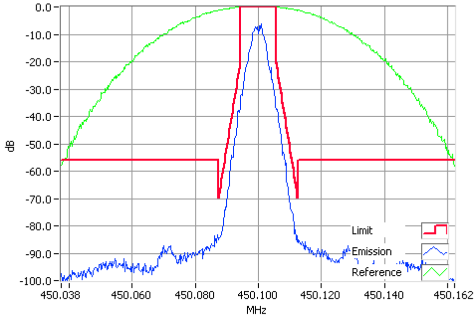
P25 Phase 1 450.1000MHz Mask D 4W RBW=100Hz, VBW=1000Hz, Detector Mode=Peak Result=Pass
