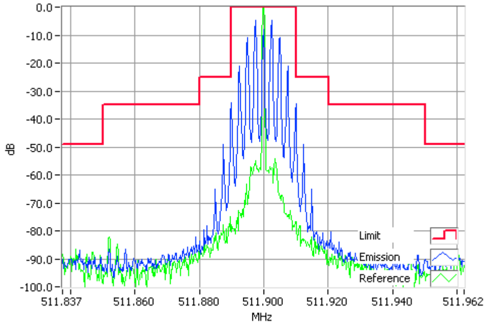
Analogue Modulation 511.9000MHz Mask B 4W RBW=300Hz, VBW=3000Hz, Detector Mode=Peak Result=Pass
