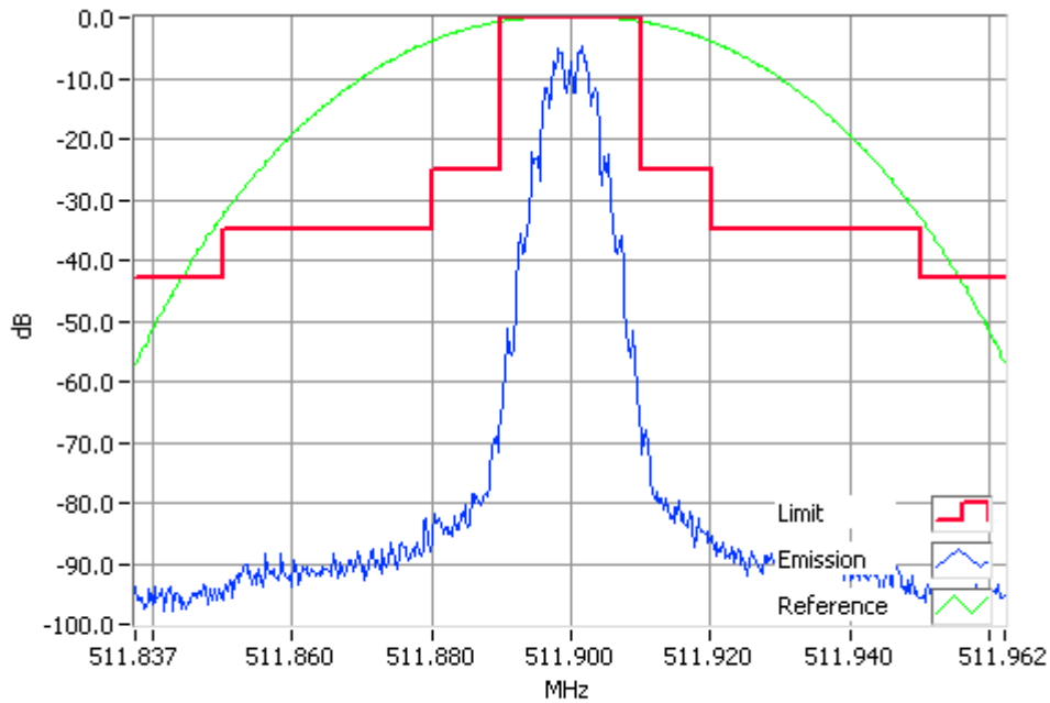
FFSK 1200 bps 511.9000MHz Mask B 1W RBW=300Hz, VBW=3000Hz, Detector Mode=Peak Result=Pass
