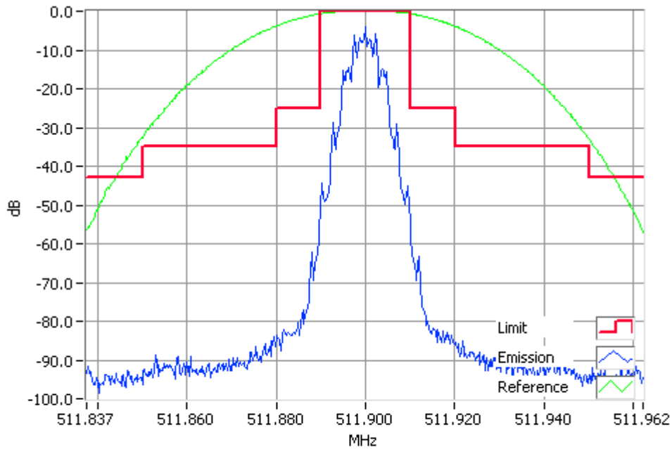
FFSK 2400 bps 511.9000MHz Mask B 1W RBW=300Hz, VBW=3000Hz, Detector Mode=Peak Result=Pass
