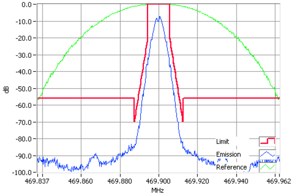
P25 Phase 1 469.9000MHz Mask D 4W RBW=100Hz, VBW=1000Hz, Detector Mode=Peak Result=Pass
