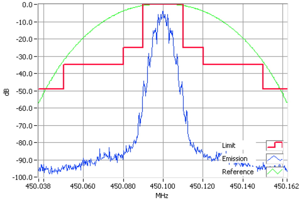
FFSK 2400 bps 450.1000MHz Mask B 4W RBW=300Hz, VBW=3000Hz, Detector Mode=Peak Result=Pass
