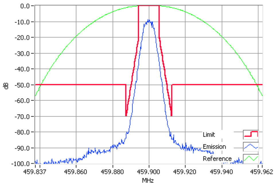
P25 Phase 2 459.9000MHz Mask D 1W RBW=100Hz, VBW=1000Hz, Detector Mode=Peak Result=Pass
