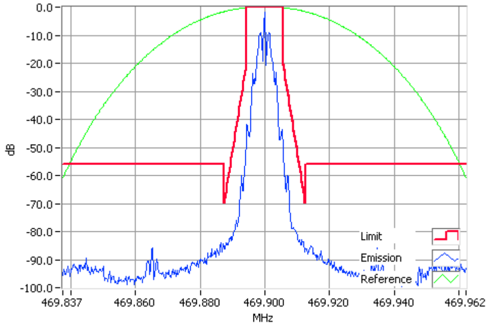
FFSK 1200 bps 469.9000MHz Mask D 4W RBW=100Hz, VBW=1000Hz, Detector Mode=Peak Result=Pass
