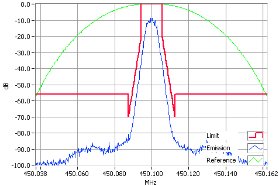
P25 Phase 2 450.1000MHz Mask D 4W RBW=100Hz, VBW=1000Hz, Detector Mode=Peak Result=Pass
