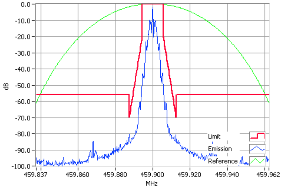
FFSK 1200 bps 459.9000MHz Mask D 4W RBW=100Hz, VBW=1000Hz, Detector Mode=Peak Result=Pass
