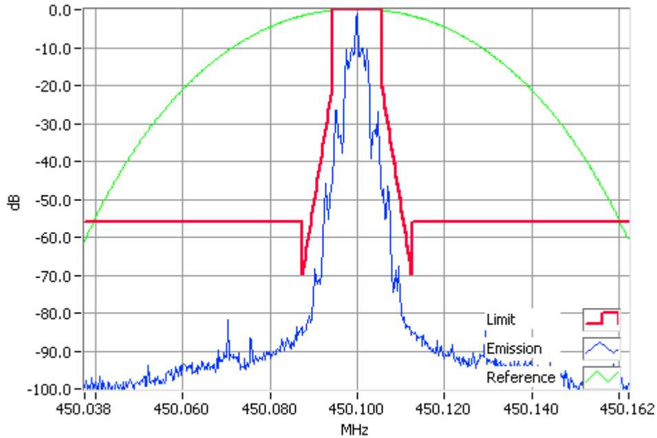
FFSK 2400 bps 450.1000MHz Mask D 4W RBW=100Hz, VBW=1000Hz, Detector Mode=Peak Result=Pass
