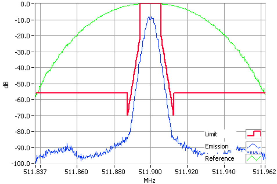
P25 Phase 1 511.9000MHz Mask D 4W RBW=100Hz, VBW=1000Hz, Detector Mode=Peak Result=Pass
