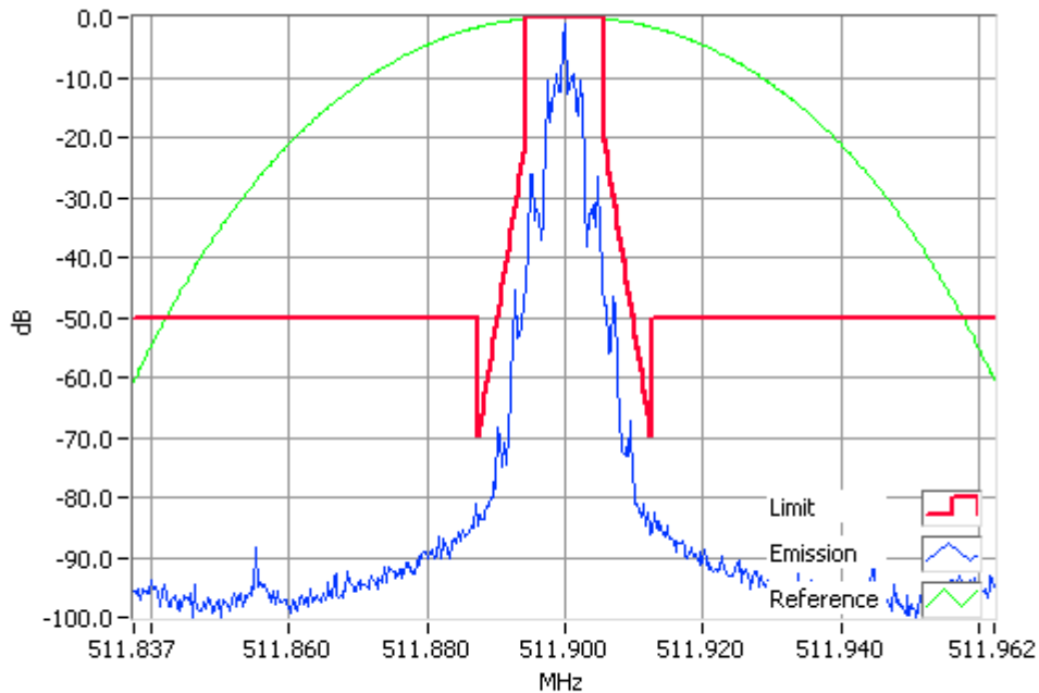
FFSK 2400 bps 511.9000MHz Mask D 1W RBW=100Hz, VBW=1000Hz, Detector Mode=Peak Result=Pass
