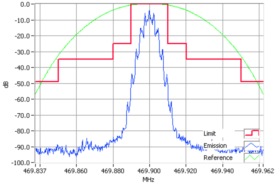
FFSK 2400 bps 469.9000MHz Mask B 4W RBW=300Hz, VBW=3000Hz, Detector Mode=Peak Result=Pass
