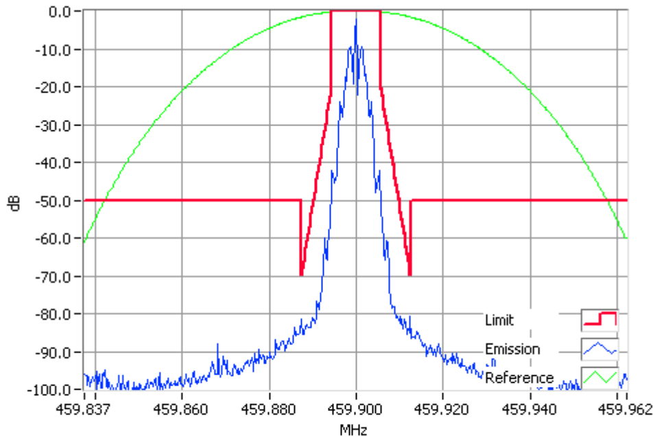
FFSK 1200 bps 459.9000MHz Mask D 1W RBW=100Hz, VBW=1000Hz, Detector Mode=Peak Result=Pass
