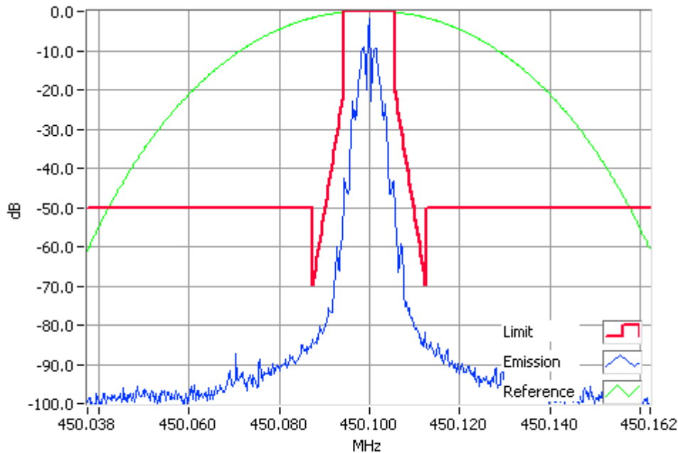
FFSK 1200 bps 450.1000MHz Mask D 1W RBW=100Hz, VBW=1000Hz, Detector Mode=Peak Result=Pass
