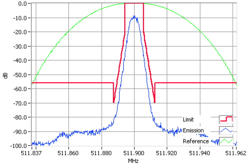
P25 Phase 2 511.9000MHz Mask D 4W RBW=100Hz, VBW=1000Hz, Detector Mode=Peak Result=Pass
