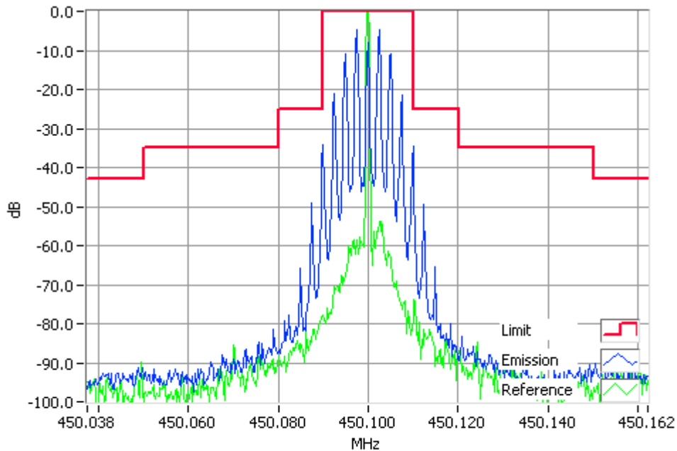
Analogue Modulation 450.1000MHz Mask B 1W RBW=300Hz, VBW=3000Hz, Detector Mode=Peak Result=Pass
