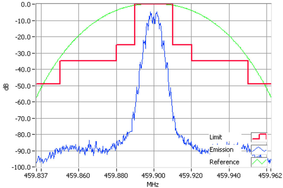
FFSK 1200 bps 459.9000MHz Mask B 4W RBW=300Hz, VBW=3000Hz, Detector Mode=Peak Result=Pass
