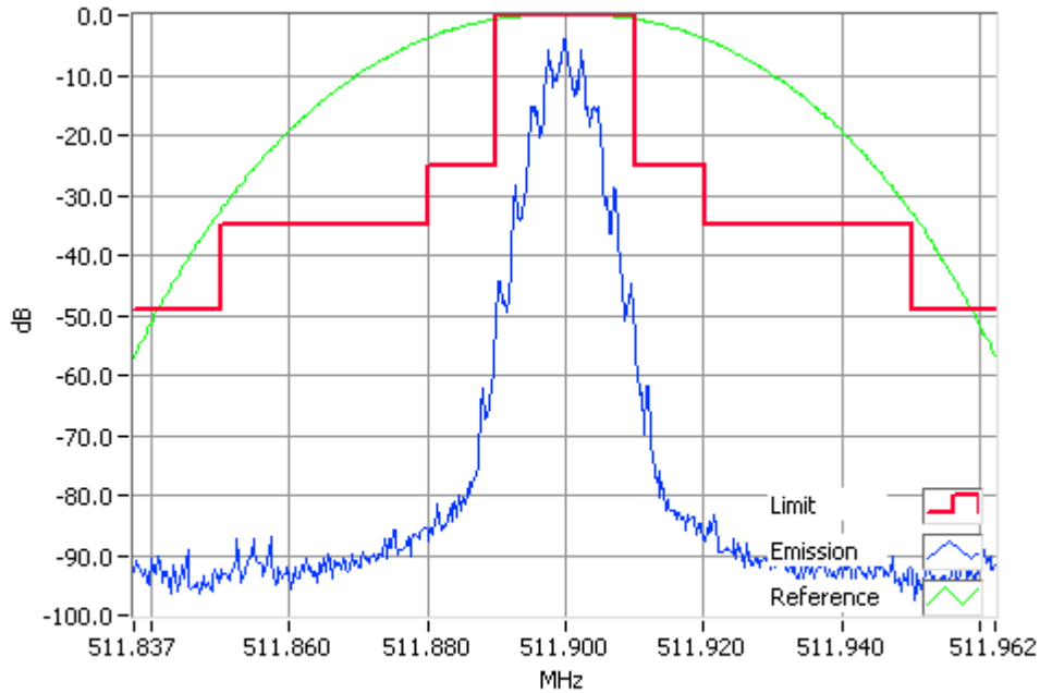
FFSK 2400 bps 511.9000MHz Mask B 4W RBW=300Hz, VBW=3000Hz, Detector Mode=Peak Result=Pass
