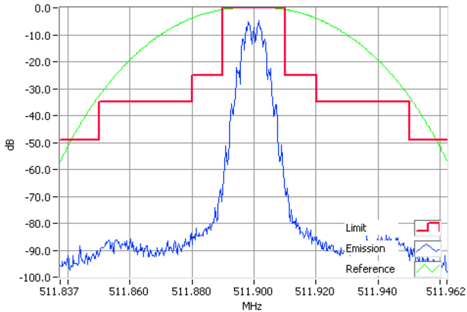
FFSK 1200 bps 511.9000MHz Mask B 4W RBW=300Hz, VBW=3000Hz, Detector Mode=Peak Result=Pass
