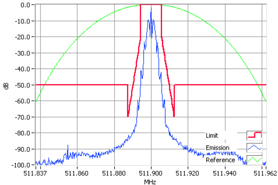
FFSK 1200 bps 511.9000MHz Mask D 1W RBW=100Hz, VBW=1000Hz, Detector Mode=Peak Result=Pass
