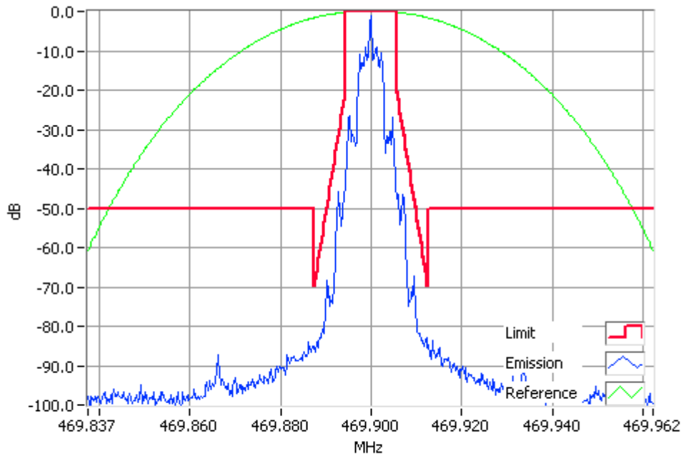
FFSK 2400 bps 469.9000MHz Mask D 1W RBW=100Hz, VBW=1000Hz, Detector Mode=Peak Result=Pass
