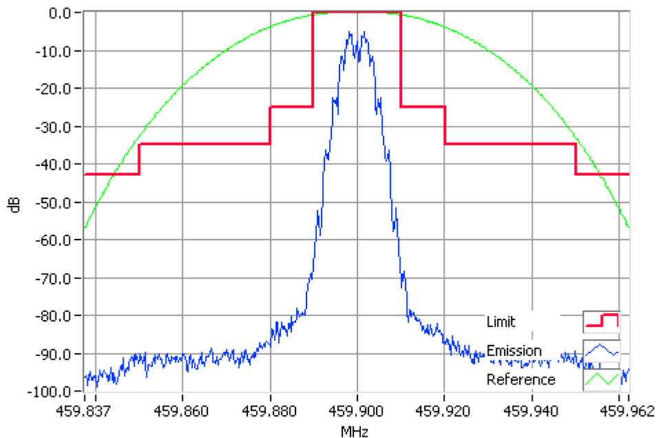
FFSK 1200 bps 459.9000MHz Mask B 1W RBW=300Hz, VBW=3000Hz, Detector Mode=Peak Result=Pass
