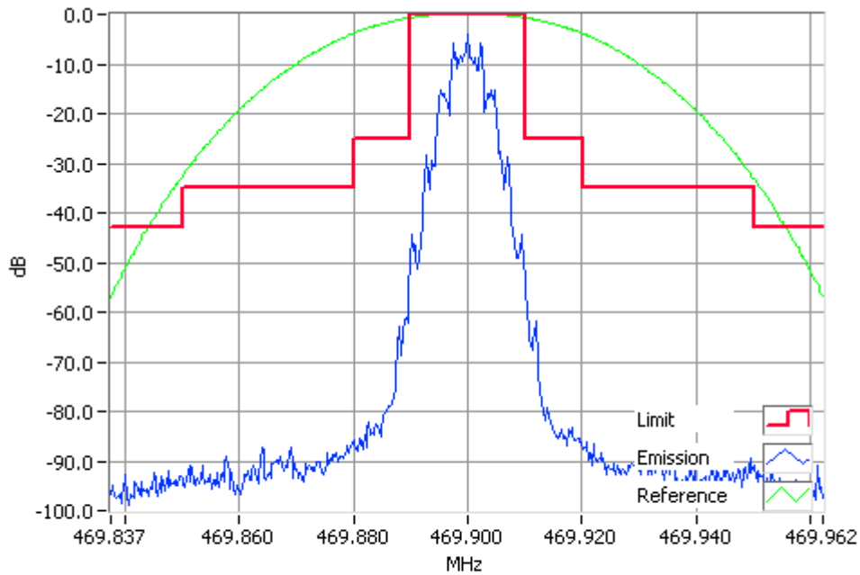
FFSK 2400 bps 469.9000MHz Mask B 1W RBW=300Hz, VBW=3000Hz, Detector Mode=Peak Result=Pass
