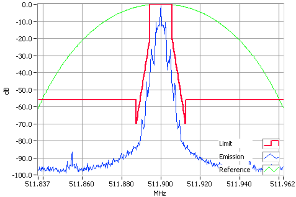
FFSK 2400 bps 511.9000MHz Mask D 4W RBW=100Hz, VBW=1000Hz, Detector Mode=Peak Result=Pass
