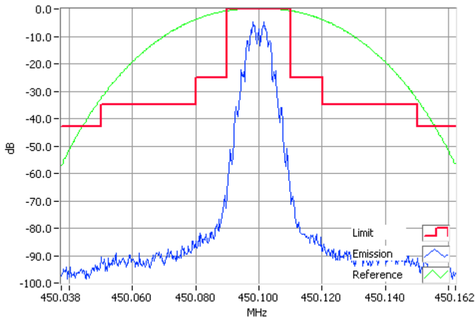
FFSK 1200 bps 450.1000MHz Mask B 1W RBW=300Hz, VBW=3000Hz, Detector Mode=Peak Result=Pass
