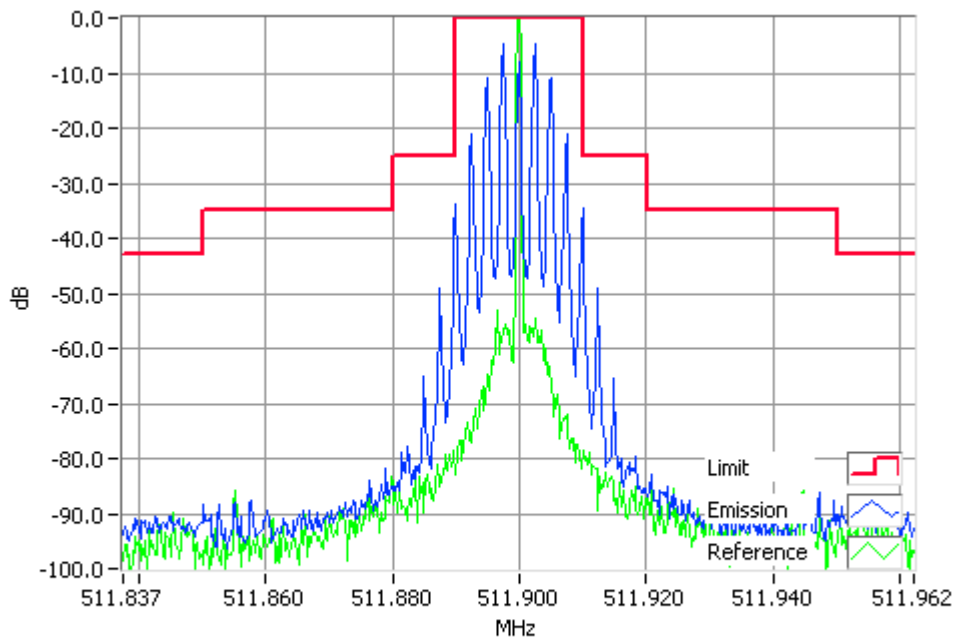
Analogue Modulation 511.9000MHz Mask B 1W RBW=300Hz, VBW=3000Hz, Detector Mode=Peak Result=Pass
