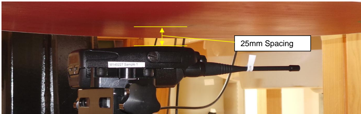
Face Frontal Position 25mm Spacing (Antenna Whip)
