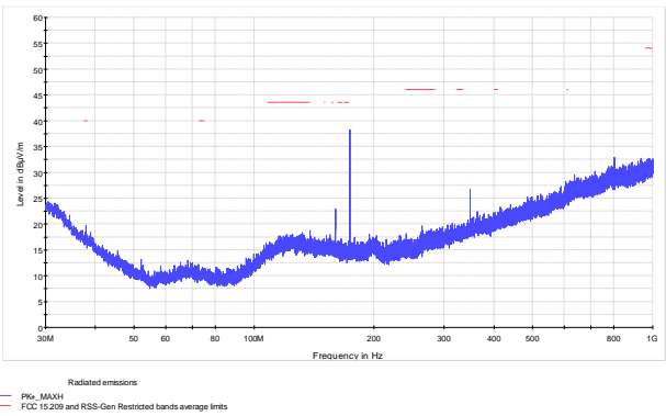
Figure 8.6-30: Radiated spurious emissions below 1 GHz, VHF radio on
