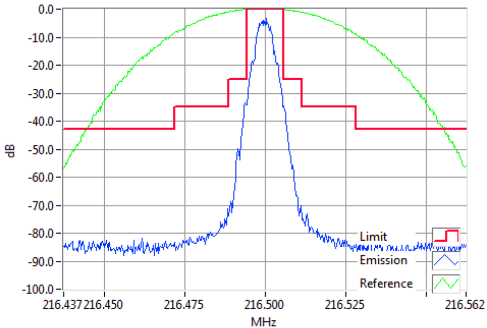
DMR 216.5000MHz Mask B 1W RBW=300Hz, VBW=3000Hz, Detector Mode=Peak Result=Pass
