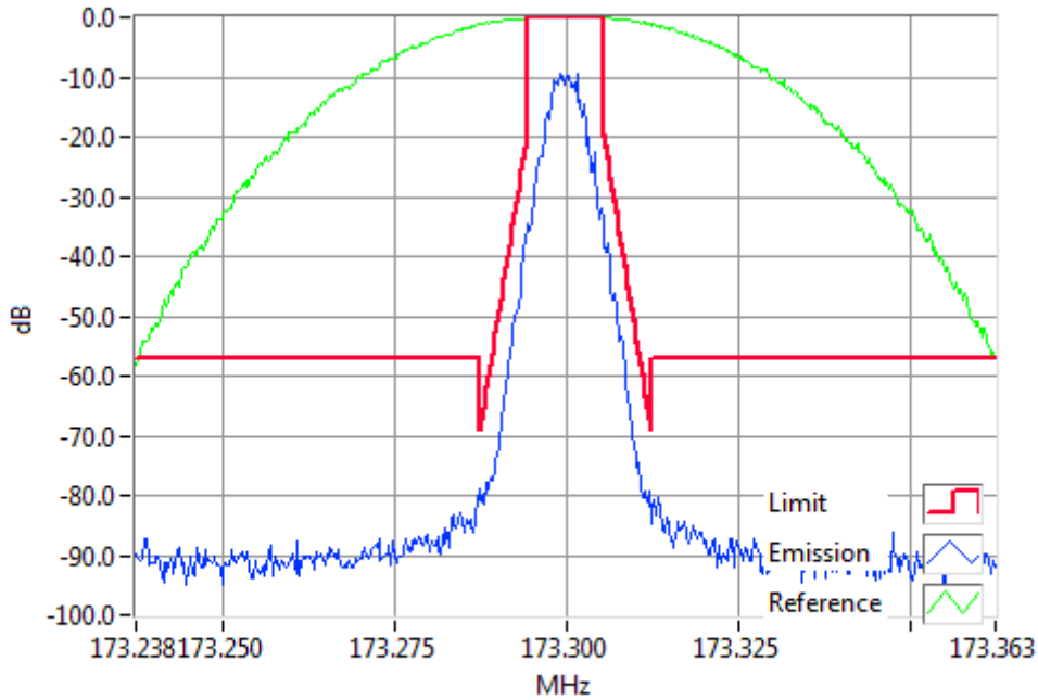
P25I 173.3000MHz Mask D 5W RBW=100Hz, VBW=1000Hz, Detector Mode=Peak Result=Pass
