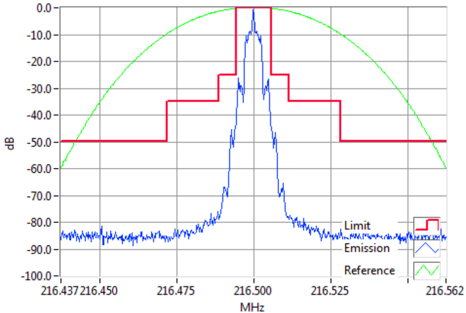
FFSK2400 216.5000MHz Mask B 5W RBW=300Hz, VBW=3000Hz, Detector Mode=Peak Result=Pass
