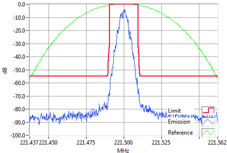
DMR 221.5000MHz Mask Fx4 1W RBW=300Hz, VBW=3000Hz, Detector Mode=Peak Result=Pass
