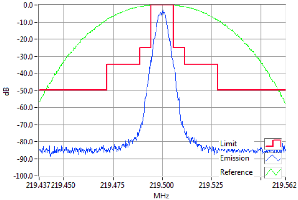
DMR 219.5000MHz Mask B 5W RBW=300Hz, VBW=3000Hz, Detector Mode=Peak Result=Pass
