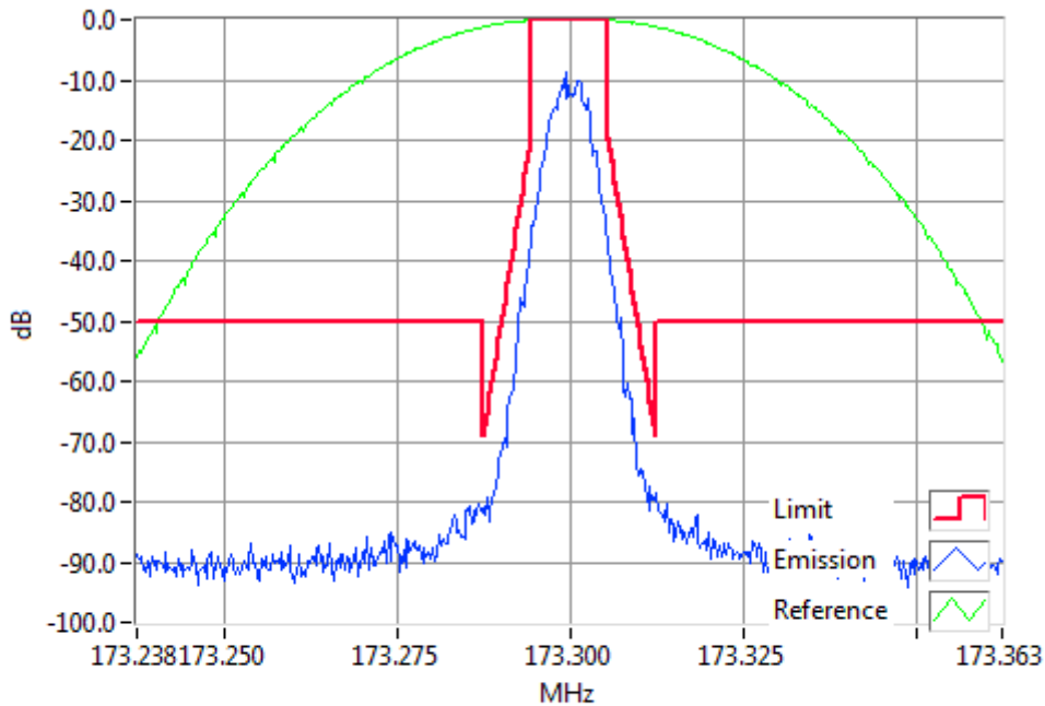
P25II 173.3000MHz Mask D 1W RBW=100Hz, VBW=1000Hz, Detector Mode=Peak Result=Pass
