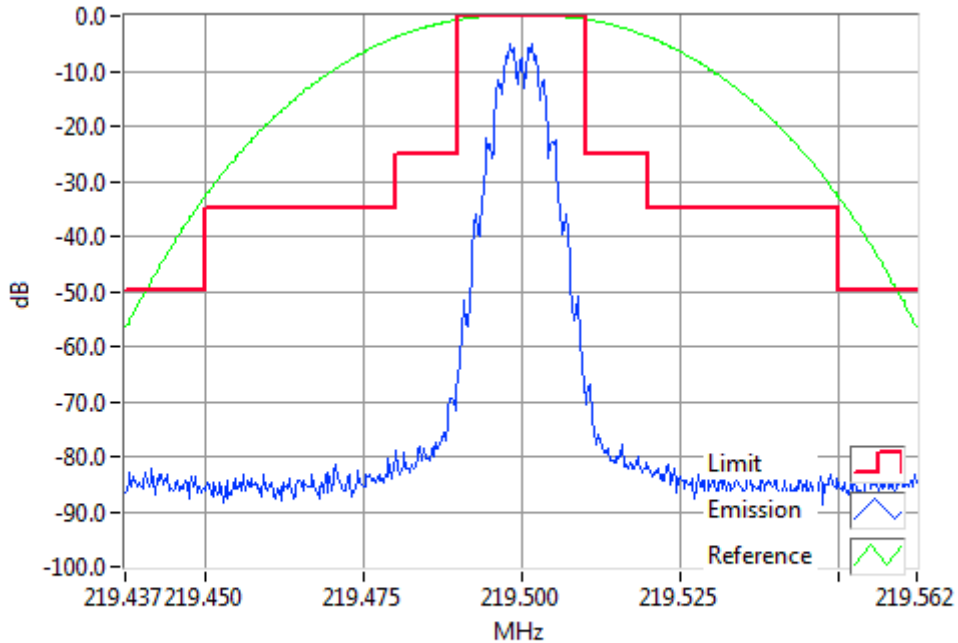
FFSK1200 219.5000MHz Mask B 5W RBW=300Hz, VBW=3000Hz, Detector Mode=Peak Result=Pass
