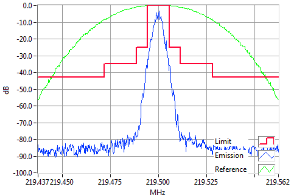
P25I 219.5000MHz Mask B 1W RBW=300Hz, VBW=3000Hz, Detector Mode=Peak Result=Pass
