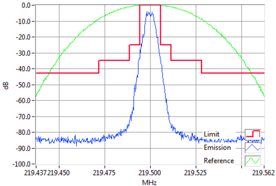
DMR 219.5000MHz Mask B 1W RBW=300Hz, VBW=3000Hz, Detector Mode=Peak Result=Pass
