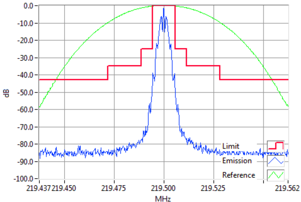
FFSK1200 219.5000MHz Mask B 1W RBW=300Hz, VBW=3000Hz, Detector Mode=Peak Result=Pass
