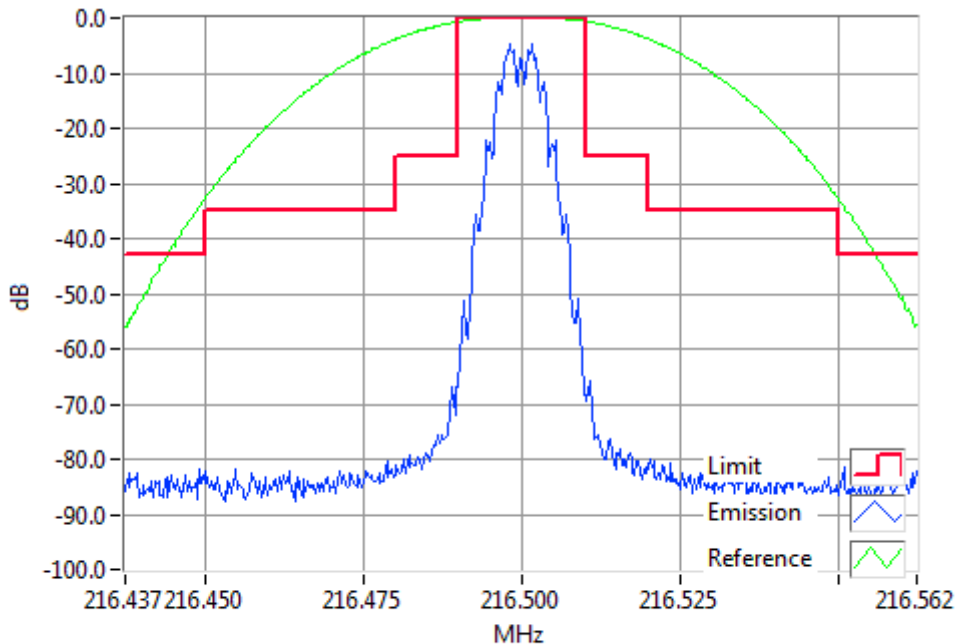
FFSK1200 216.5000MHz Mask B 1W RBW=300Hz, VBW=3000Hz, Detector Mode=Peak Result=Pass
