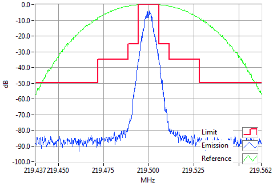
P25I 219.5000MHz Mask B 5W RBW=300Hz, VBW=3000Hz, Detector Mode=Peak Result=Pass
