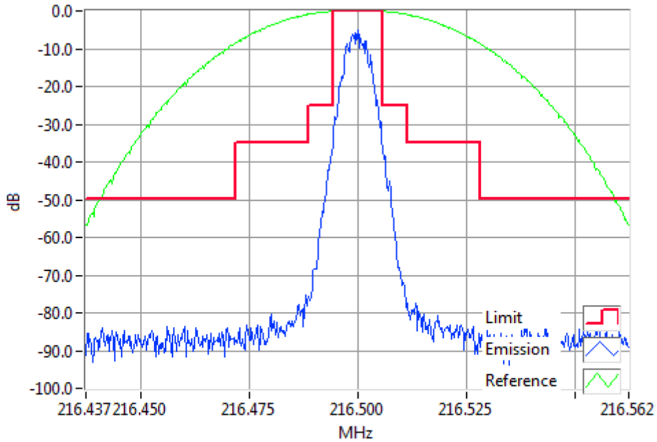
P25II 216.5000MHz Mask B 5W RBW=300Hz, VBW=3000Hz, Detector Mode=Peak Result=Pass
