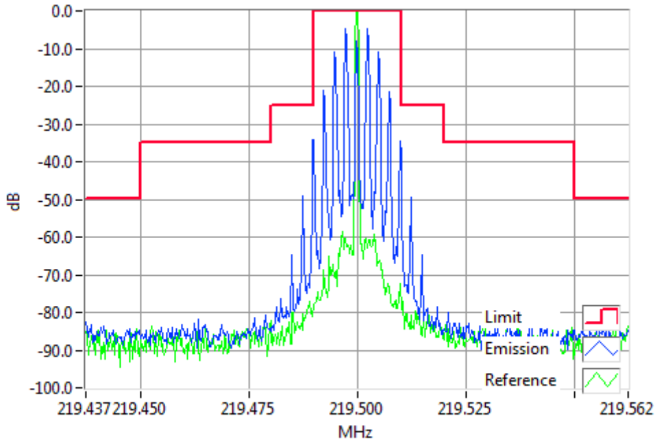
Analogue Modulation 219.5000MHz Mask B 5W RBW=300Hz, VBW=3000Hz, Detector Mode=Peak Result=Pass
