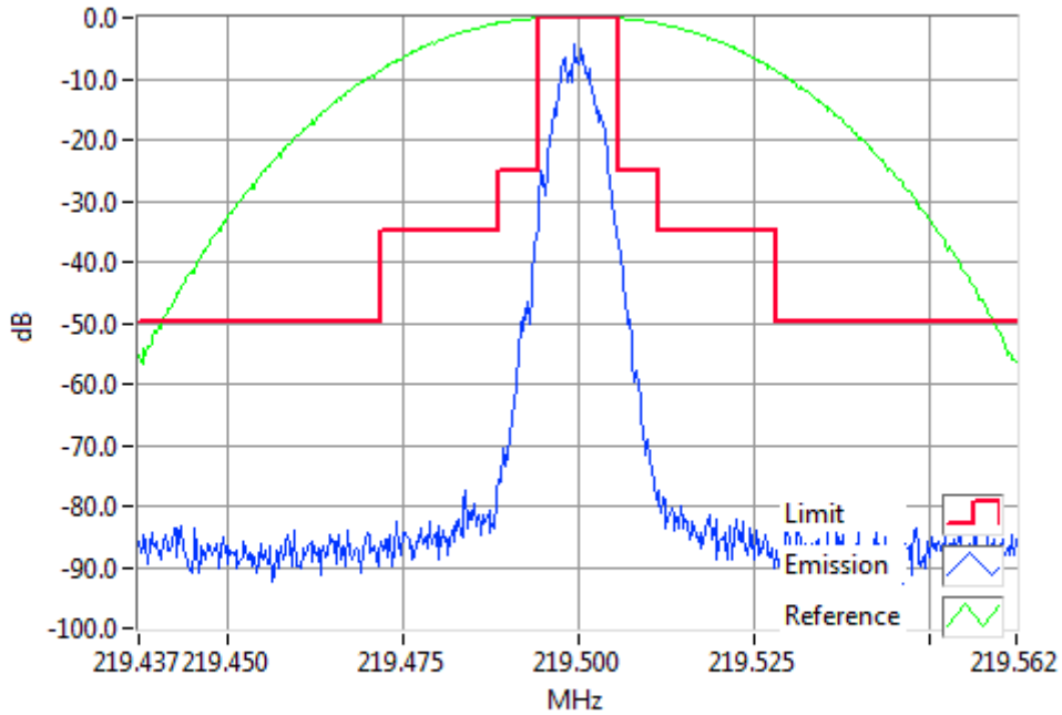
P25II 219.5000MHz Mask B 5W RBW=300Hz, VBW=3000Hz, Detector Mode=Peak Result=Pass
