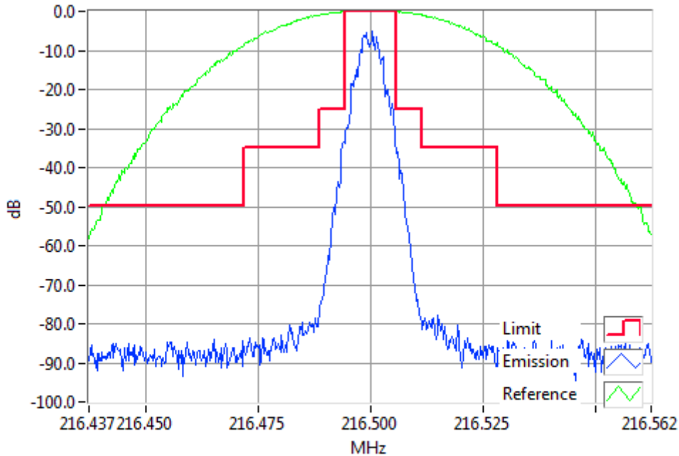
P25I 216.5000MHz Mask B 5W RBW=300Hz, VBW=3000Hz, Detector Mode=Peak Result=Pass
