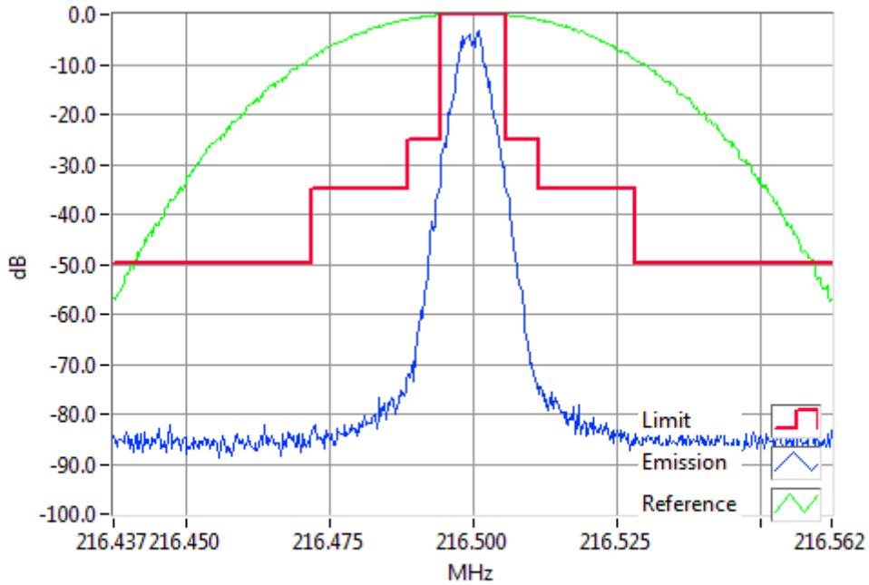
DMR 216.5000MHz Mask B 5W RBW=300Hz, VBW=3000Hz, Detector Mode=Peak Result=Pass
