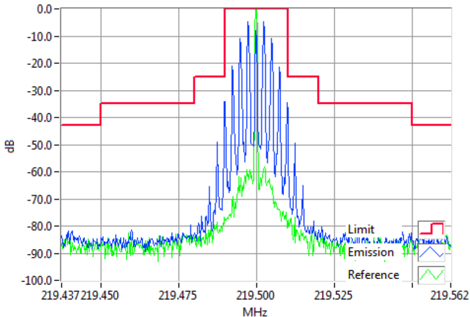
Analogue Modulation 219.5000MHz Mask B 1W RBW=300Hz, VBW=3000Hz, Detector Mode=Peak Result=Pass
