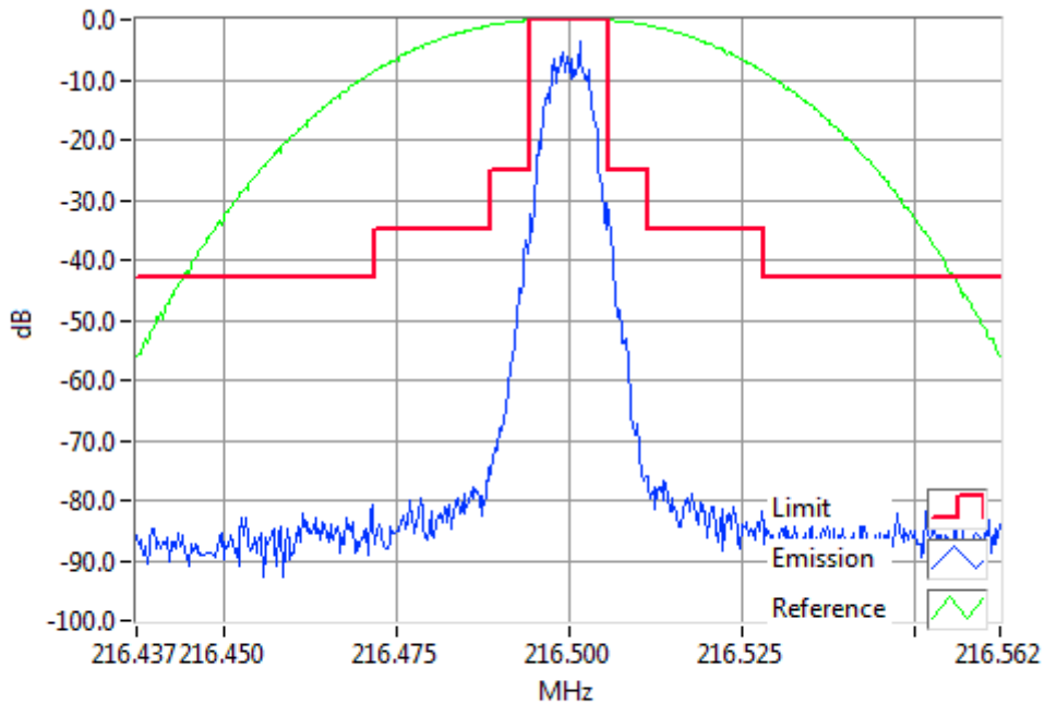
P25II 216.5000MHz Mask B 1W RBW=300Hz, VBW=3000Hz, Detector Mode=Peak Result=Pass
