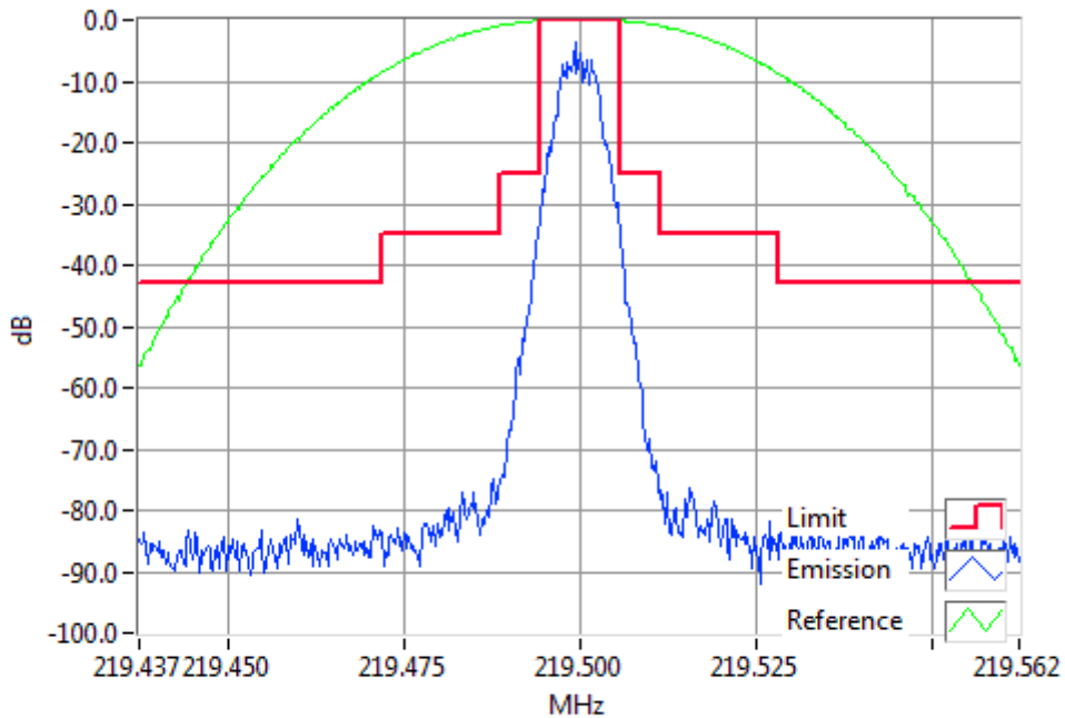
P25II 219.5000MHz Mask B 1W RBW=300Hz, VBW=3000Hz, Detector Mode=Peak Result=Pass
