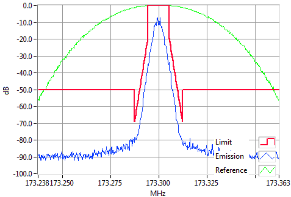
P25I 173.3000MHz Mask D 1W RBW=100Hz, VBW=1000Hz, Detector Mode=Peak Result=Pass
