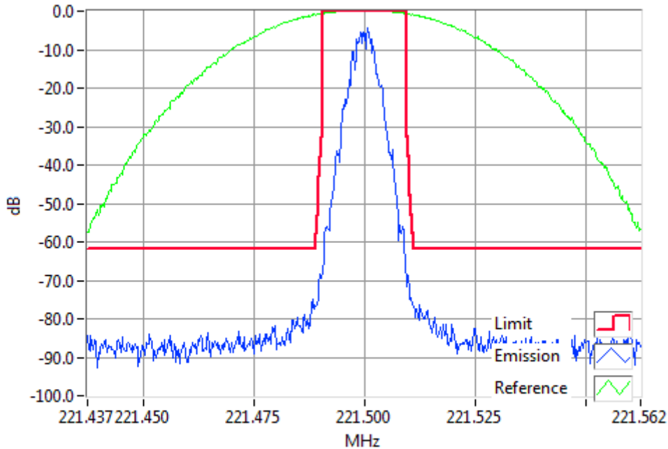
DMR 221.5000MHz Mask Fx4 5W RBW=300Hz, VBW=3000Hz, Detector Mode=Peak Result=Pass
