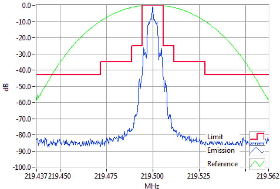
FFSK2400 219.5000MHz Mask B 1W RBW=300Hz, VBW=3000Hz, Detector Mode=Peak Result=Pass
