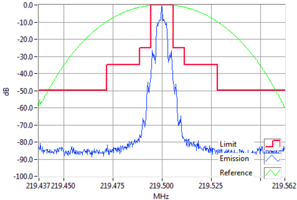
FFSK2400 219.5000MHz Mask B 5W RBW=300Hz, VBW=3000Hz, Detector Mode=Peak Result=Pass
