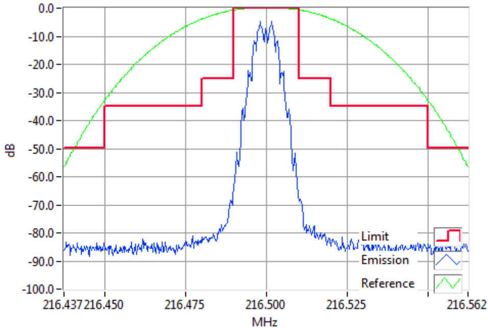
FFSK1200 216.5000MHz Mask B 5W RBW=300Hz, VBW=3000Hz, Detector Mode=Peak Result=Pass
