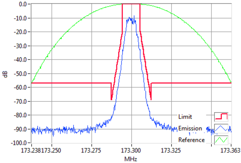
P25II 173.3000MHz Mask D 5W RBW=100Hz, VBW=1000Hz, Detector Mode=Peak Result=Pass
