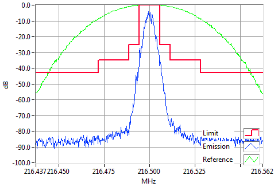
P25I 216.5000MHz Mask B 1W RBW=300Hz, VBW=3000Hz, Detector Mode=Peak Result=Pass
