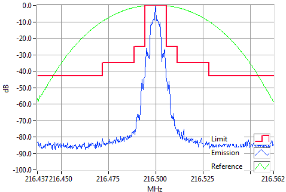
FFSK2400 216.5000MHz Mask B 1W RBW=300Hz, VBW=3000Hz, Detector Mode=Peak Result=Pass
