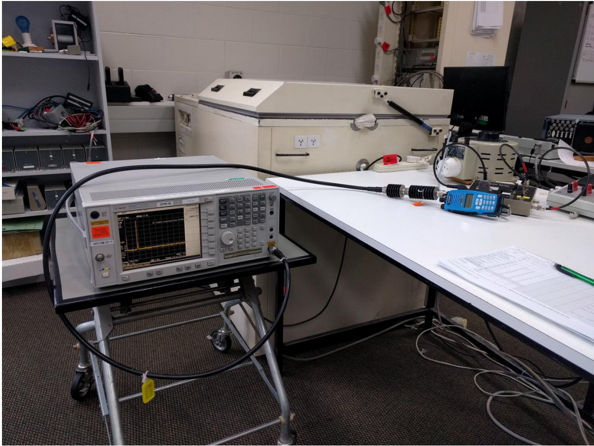
TRANSMITTER SPURIOUS EMISSIONS (CONDUCTED) SETUP
