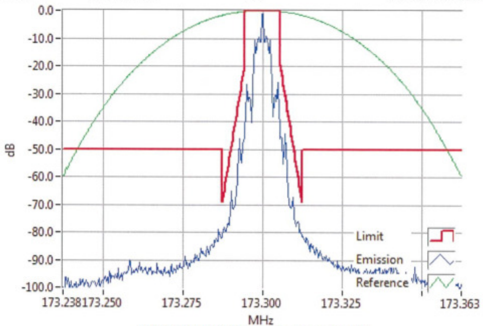
FFSK2400 173.3000MHz Mask D 1W RBW=100Hz, VBW=1000Hz, Detector Mode=Peak Result=Pass
