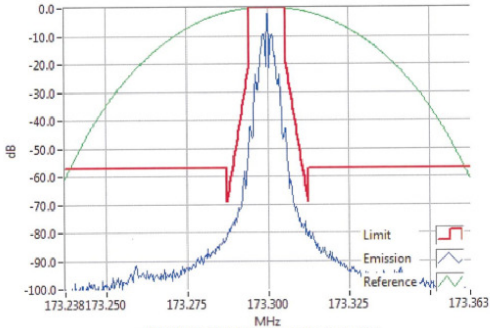
FFSK1200 173.3000MHz Mask D 5W RBW=100Hz, VBW=1000Hz, Detector Mode=Peak Result=Pass
