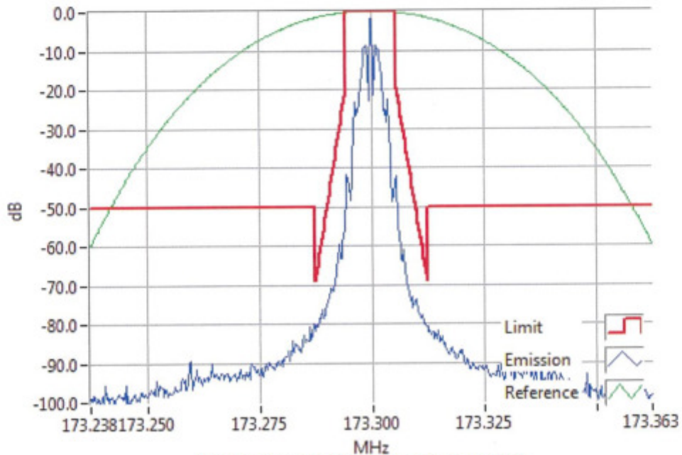
FFSK1200 173.3000MHz Mask D 1W RBW=100Hz, VBW=1000Hz, Detector Mode=Peak Result=Pass
