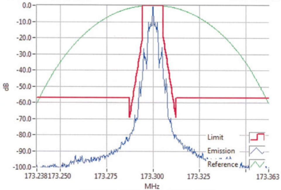
FFSK2400 173.3000MHz Mask D 5W RBW=100Hz, VBW=1000Hz, Detector Mode=Peak Result=Pass
