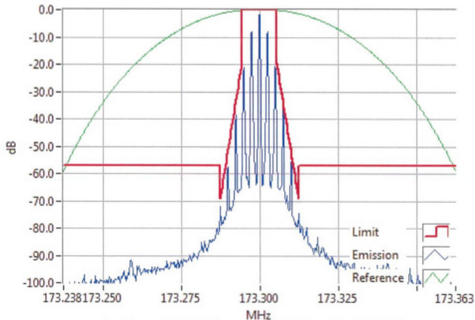
Analogue Modulation 173.3000MHz Mask D 5W RBW=100Hz, VBW=1000Hz, Detector Mode=Peak Result=Pass
