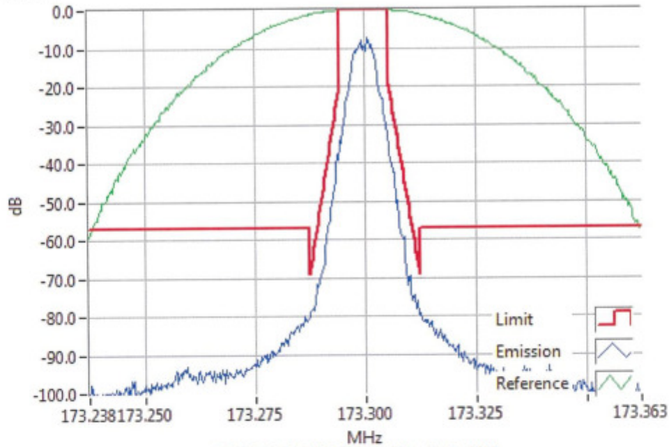
DMR 173.3000MHz Mask D 5W RBW=100Hz, VBW=1000Hz, Detector Mode=Peak Result=Pass
