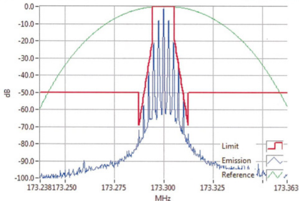
Analogue Modulation 173.3000MHz Mask D 1W RBW=100Hz, VBW=1000Hz, Detector Mode=Peak Result=Pass
