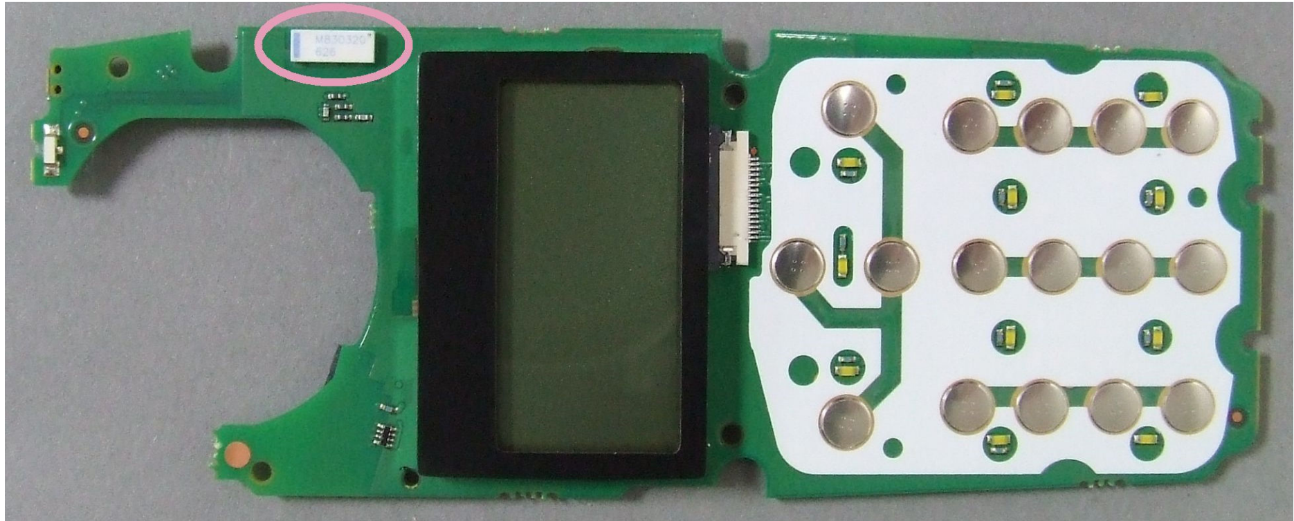
Photograph 02: Control PCB – bottom. BT antenna circled.
