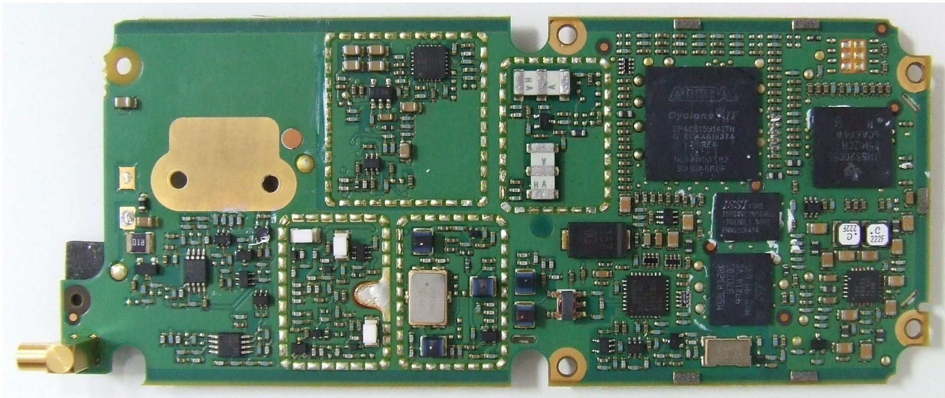
Photograph 05: Rx-Tx PCB - bottom (without shields)
