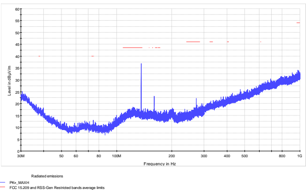
Figure 8.6-30: d spurious emissions below 1 GHz with VHF radio turned on
