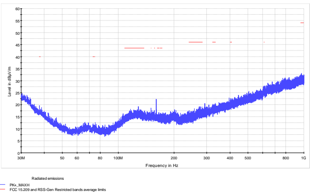
Figure 8.6-28: Radiated spurious emissions below 1 GHz at mid channel
