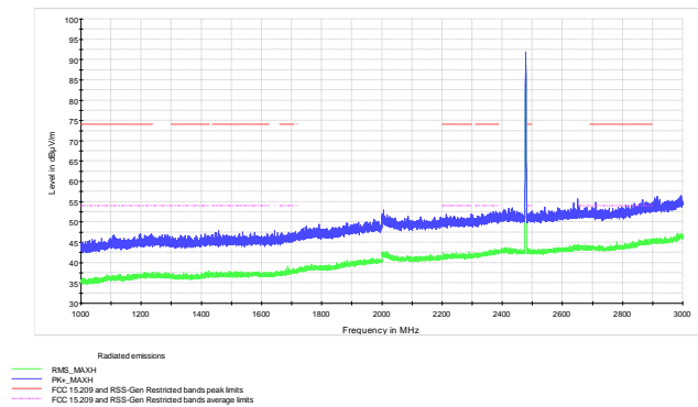
Figure 8.6-33: Radiated spurious emissions within 1–3 GHz, high channel
