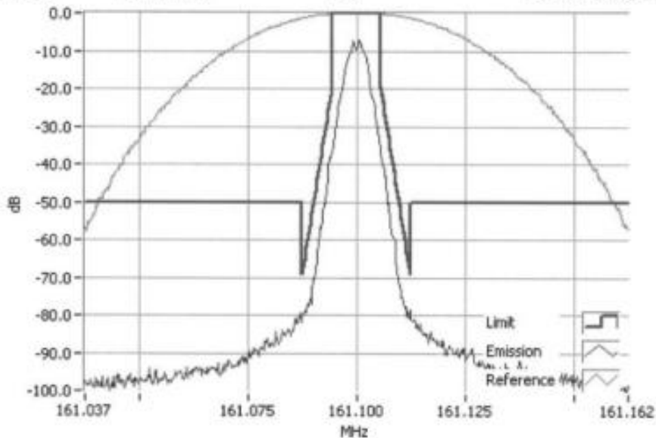
DMR 161.1000MHz Mask D 1W RBW=100Hz, VBW=1000Hz, Detector Mode=Peak Result=Pass
