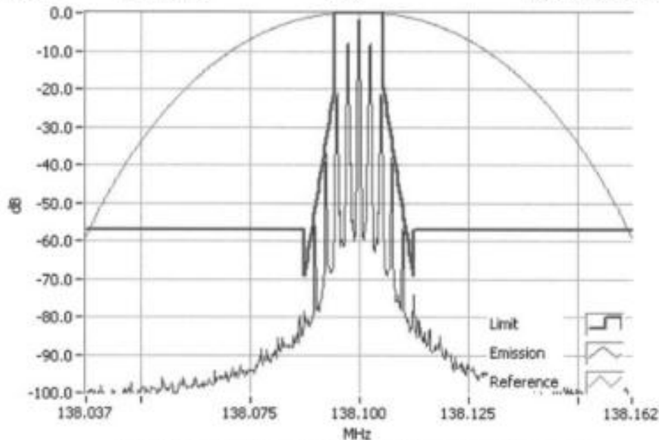
Analogue Modulation 138.1000MHz Mask D 5W RBW=100Hz, VBW=1000Hz, Detector Mode=Peak Result=Pass
