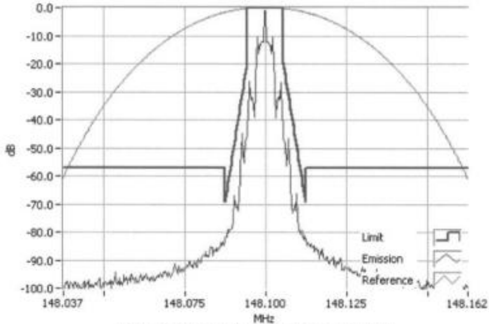
FFSK 2400 148.1000MHz Mask D 5W RBW=100Hz, VBW=1000Hz, Detector Mode=Peak Result=Pass
