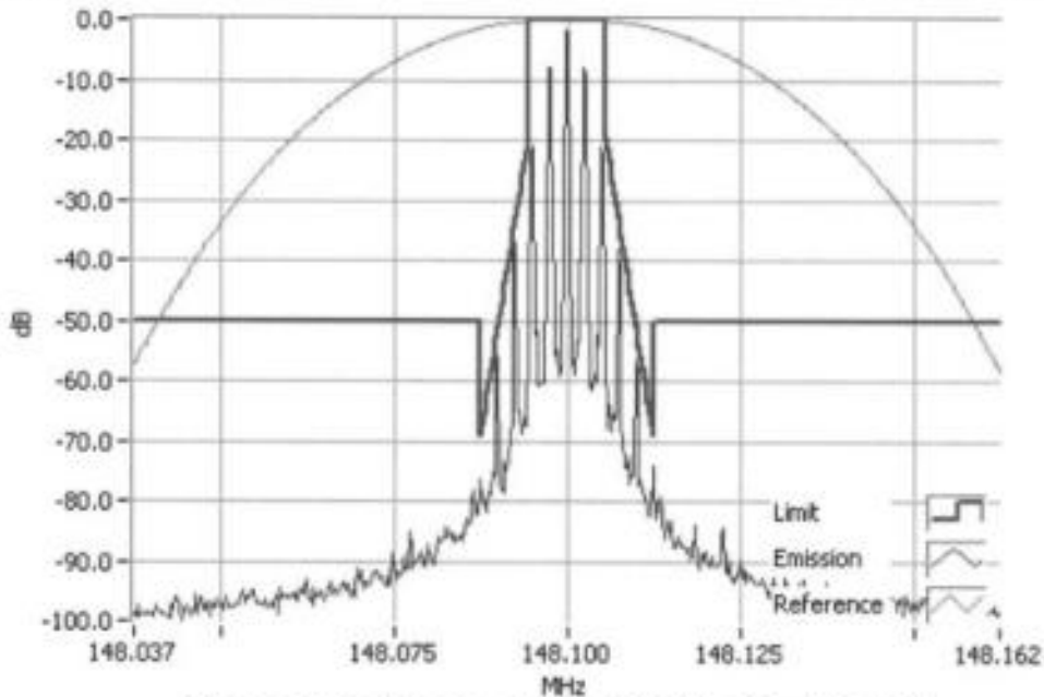
Analogue Modulation 148.1000MHz Mask D 1W RBW=100Hz, VBW=1000Hz, Detector Mode=Peak Result=Pass
