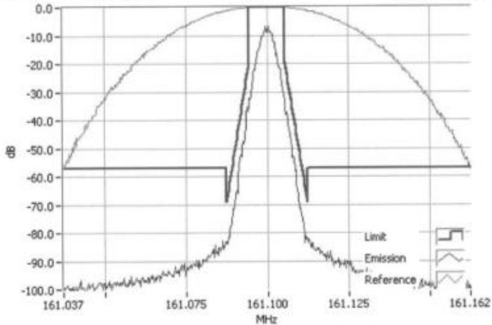
P25 Ph 1 161.1000MHz Mask D 5W RBW=100Hz, VBW=1000Hz, Detector Mode=Peak Result=Pass
