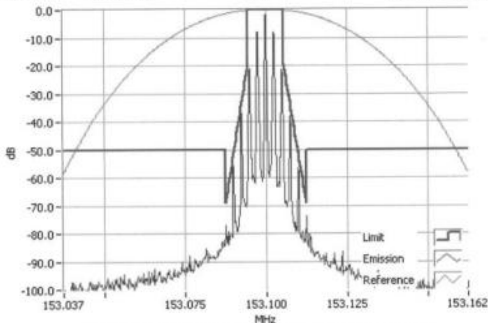
Analogue Modulation 153.1000MHz Mask D 1W RBW=100Hz, VBW=1000Hz, Detector Mode=Peak Result=Pass
