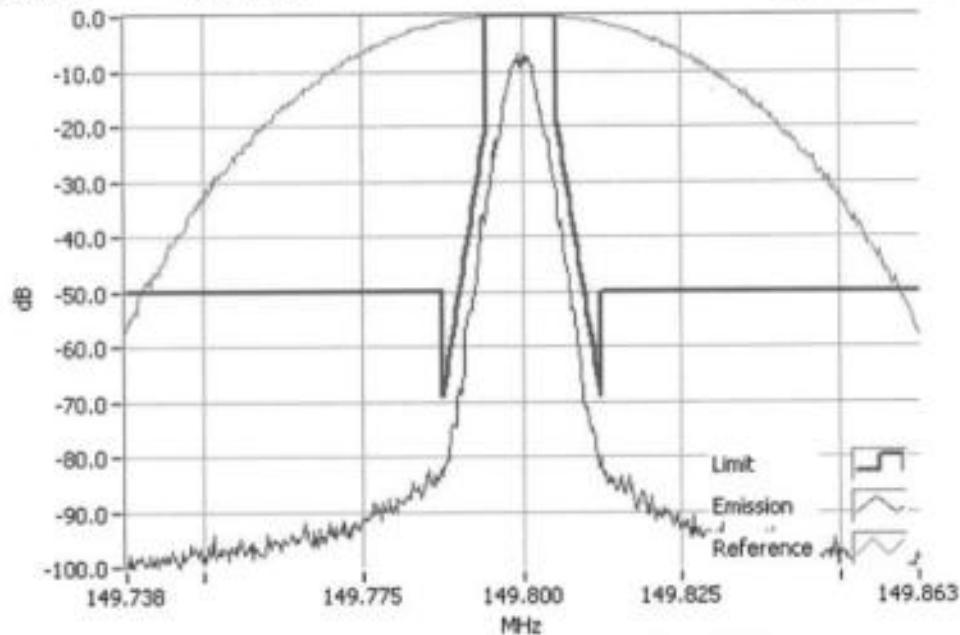
P25 Ph 1 149.8000MHz Mask D 1W RBW=100Hz, VBW=1000Hz, Detector Mode=Peak Result=Pass
