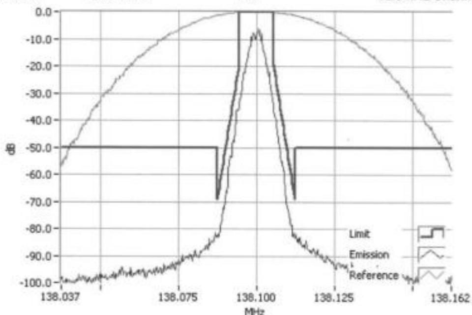
P25 Ph 1 138.1000MHz Mask D 1W RBW=100Hz, VBW=1000Hz, Detector Mode=Peak Result=Pass
