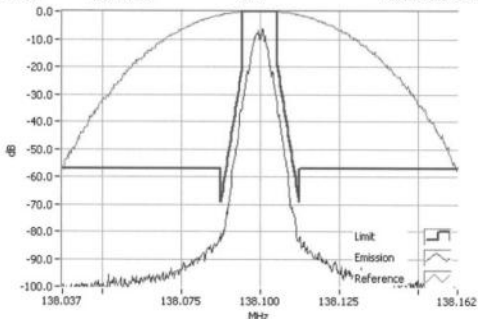
P25 Ph 1 138.1000MHz Mask D 5W RBW=100Hz, VBW=1000Hz, Detector Mode=Peak Result=Pass
