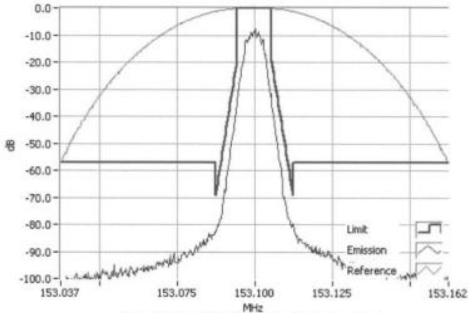
P25 Ph 2 153.1000MHz Mask D 5W RBW=100Hz, VBW=1000Hz, Detector Mode=Peak Result=Pass
