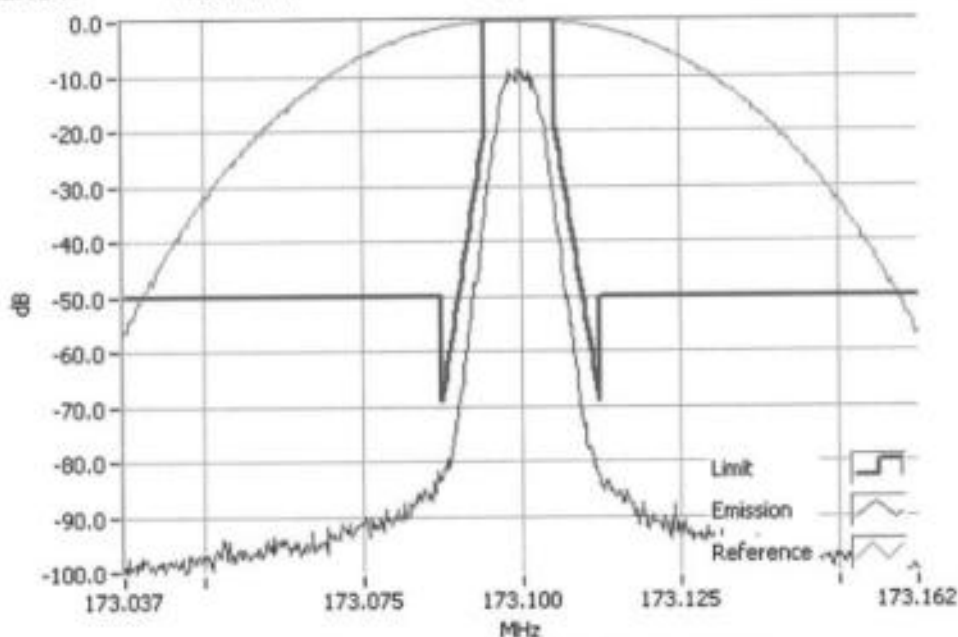
P25 Ph 2 173.1000MHz Mask D 1W RBW=100Hz, VBW=1000Hz, Detector Mode=Peak Result=Pass
