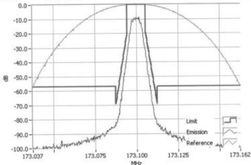
P25 Ph 2 173.1000MHz Mask D 5W RBW=100Hz, VBW=1000Hz, Detector Mode=Peak Result=Pass
