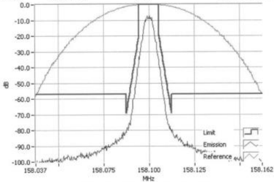
DMR 158.1000MHz Mask D 5W RBW=100Hz, VBW=1000Hz, Detector Mode=Peak Result=Pass
