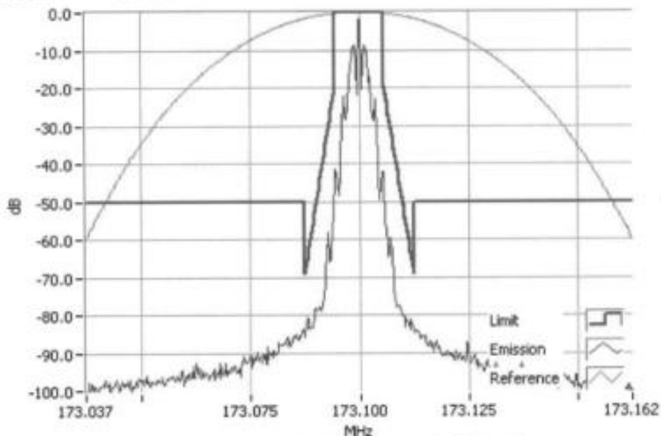
FFSK 1200 173.1000MHz Mask D 1W RBW=100Hz, VBW=1000Hz, Detector Mode=Peak Result=Pass
