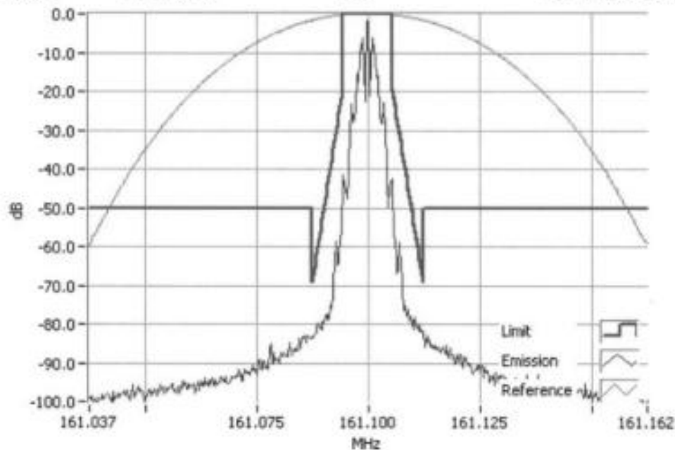
FFSK 1200 161.1000MHz Mask D 1W RBW=100Hz, VBW=1000Hz, Detector Mode=Peak Result=Pass
