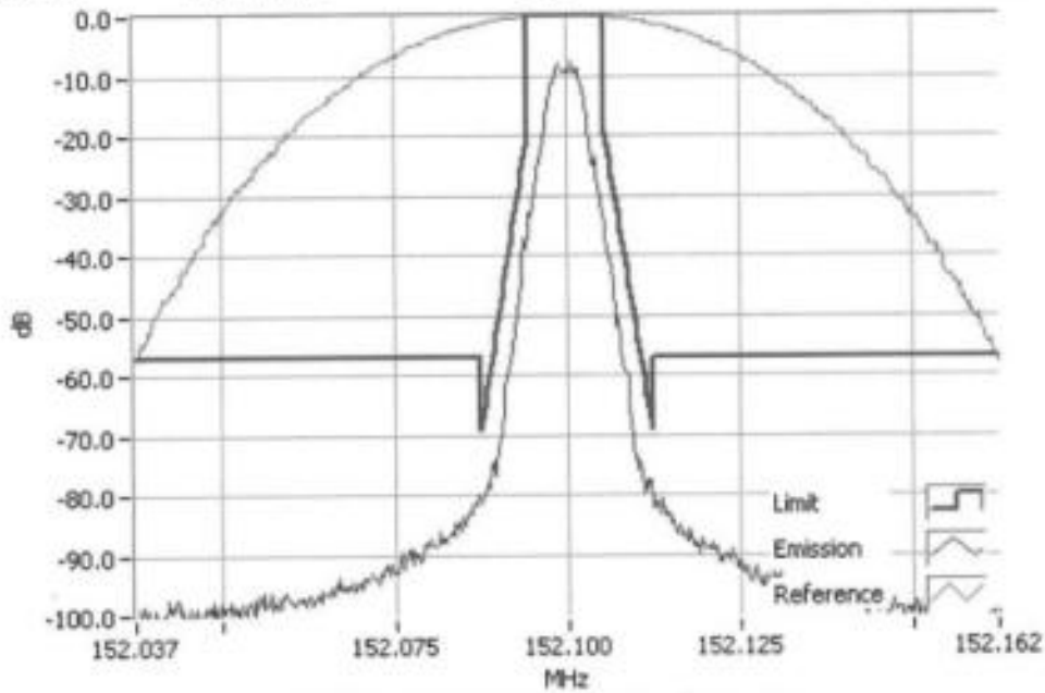
DMR 152.1000MHz Mask D 5W RBW=100Hz, VBW=1000Hz, Detector Mode=Peak Result=Pass
