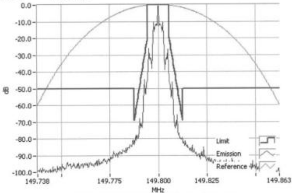
FFSK 2400 149.8000MHz Mask D 1W RBW=100Hz, VBW=1000Hz, Detector Mode=Peak Result=Pass
