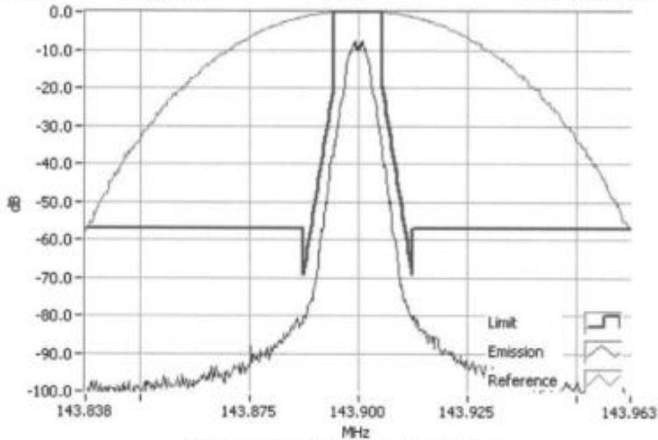
DMR 143.9000MHz Mask D 5W RBW=100Hz, VBW=1000Hz, Detector Mode=Peak Result=Pass
