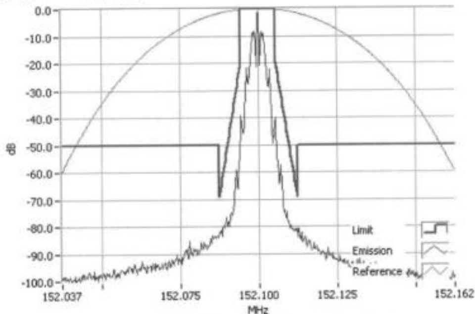
FFSK 1200 152.1000MHz Mask D 1W RBW=100Hz, VBW=1000Hz, Detector Mode=Peak Result=Pass
