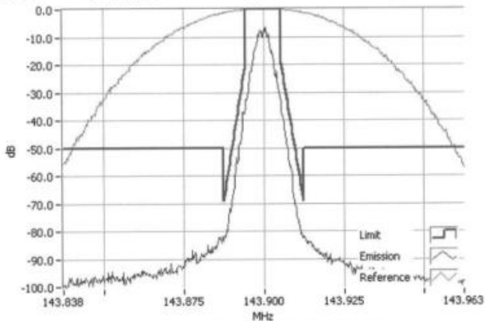
P25 Ph 1 143.9000MHz Mask D 1W RBW=100Hz, VBW=1000Hz, Detector Mode=Peak Result=Pass
