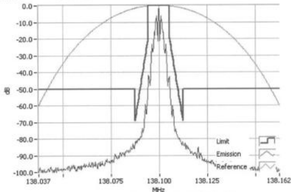
FFSK 1200 138.1000MHz Mask D 1W RBW=100Hz, VBW=1000Hz, Detector Mode=Peak Result=Pass
