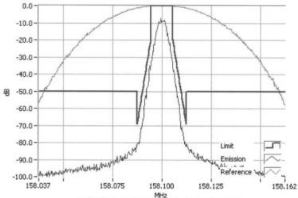
P25 Ph 1 158.1000MHz Mask D 1W RBW=100Hz, VBW=1000Hz, Detector Mode=Peak Result=Pass
