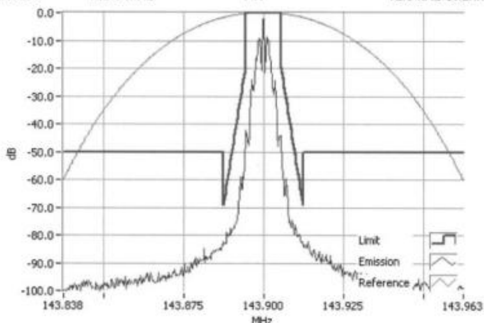
FFSK 1200 143.9000MHz Mask D 1W RBW=100Hz, VBW=1000Hz, Detector Mode=Peak Result=Pass
