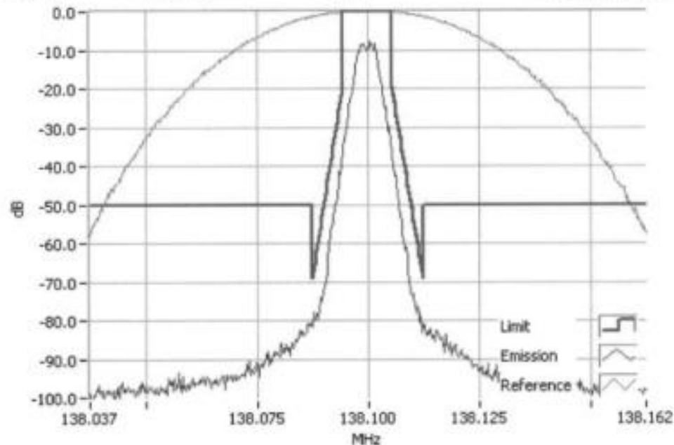
DMR 138.1000MHz Mask D 1W RBW=100Hz, VBW=1000Hz, Detector Mode=Peak Result=Pass
