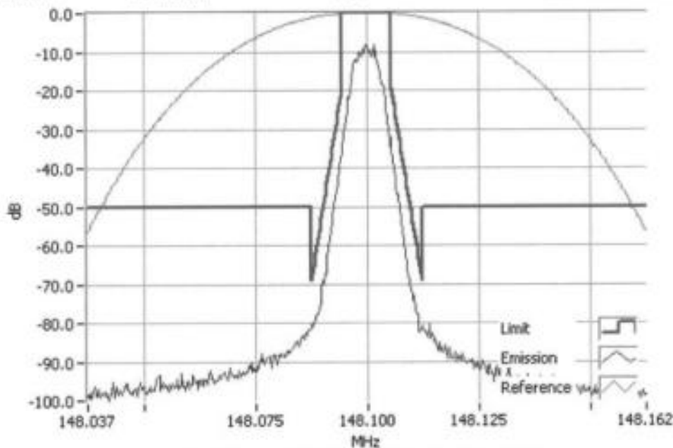
P25 Ph 2 148.1000MHz Mask D 1W RBW=100Hz, VBW=1000Hz, Detector Mode=Peak Result=Pass
