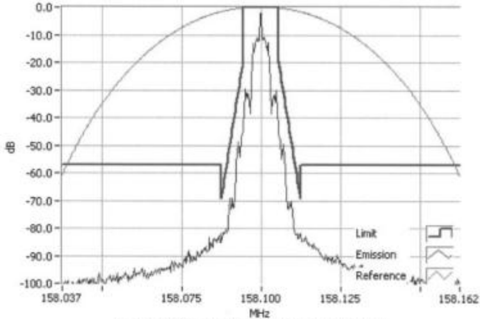
FFSK 2400 158.1000MHz Mask D 5W RBW=100Hz, VBW=1000Hz, Detector Mode=Peak Result=Pass
