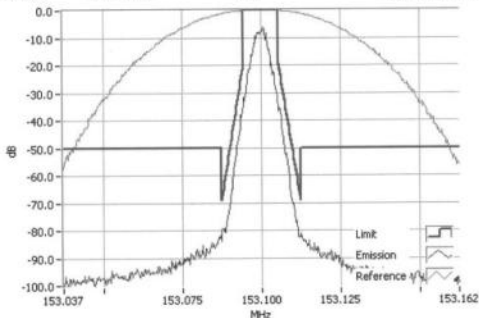
P25 Ph 1 153.1000MHz Mask D 1W RBW=100Hz, VBW=1000Hz, Detector Mode=Peak Result=Pass
