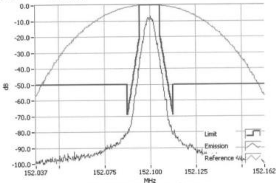
DMR 152.1000MHz Mask D 1W RBW=100Hz, VBW=1000Hz, Detector Mode=Peak Result=Pass
