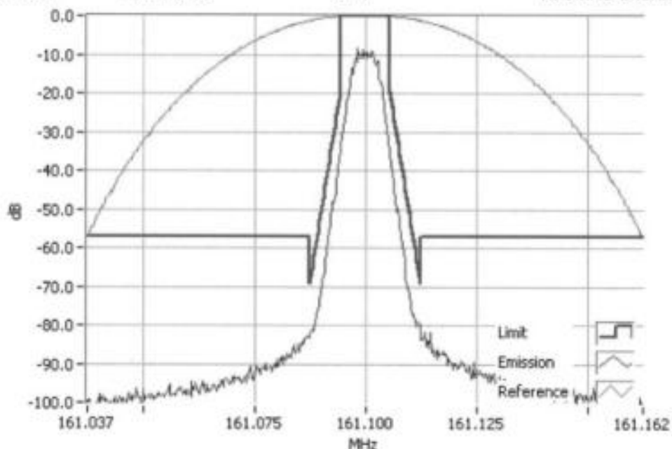
P25 Ph 2 161.1000MHz Mask D 5W RBW=100Hz, VBW=1000Hz, Detector Mode=Peak Result=Pass
