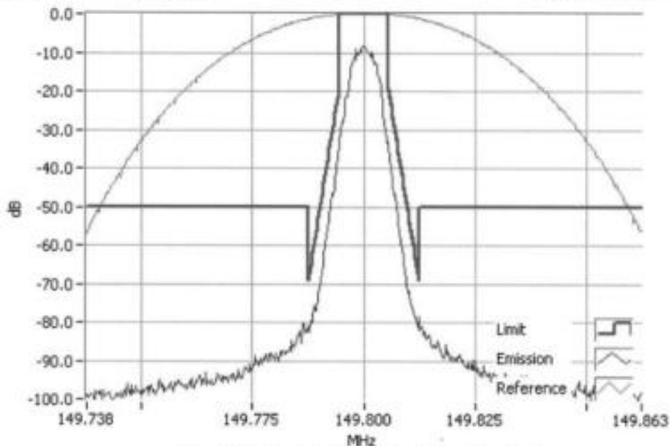
P25 Ph 2 149.8000MHz Mask D 1W RBW=100Hz, VBW=1000Hz, Detector Mode=Peak Result=Pass
