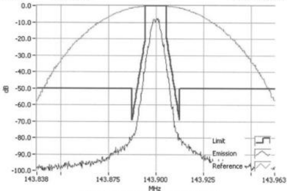
DMR 143.9000MHz Mask D 1W RBW=100Hz, VBW=1000Hz, Detector Mode=Peak Result=Pass
