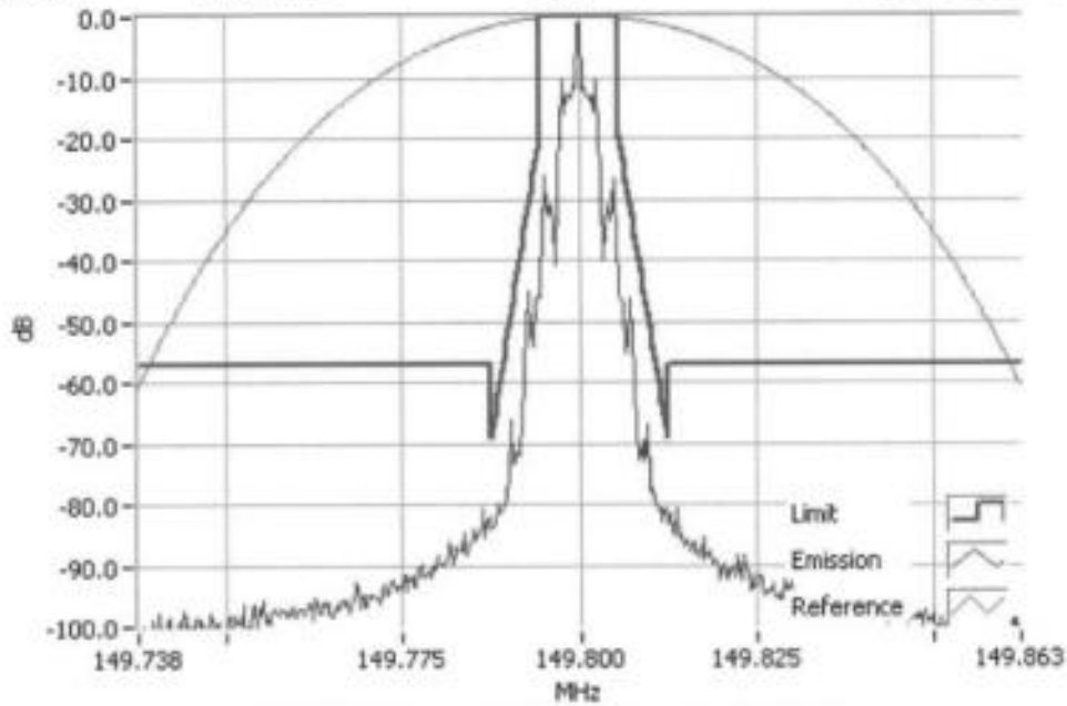
FFSK 2400 149.8000MHz Mask D 5W RBW=100Hz, VBW=1000Hz, Detector Mode=Peak Result=Pass
