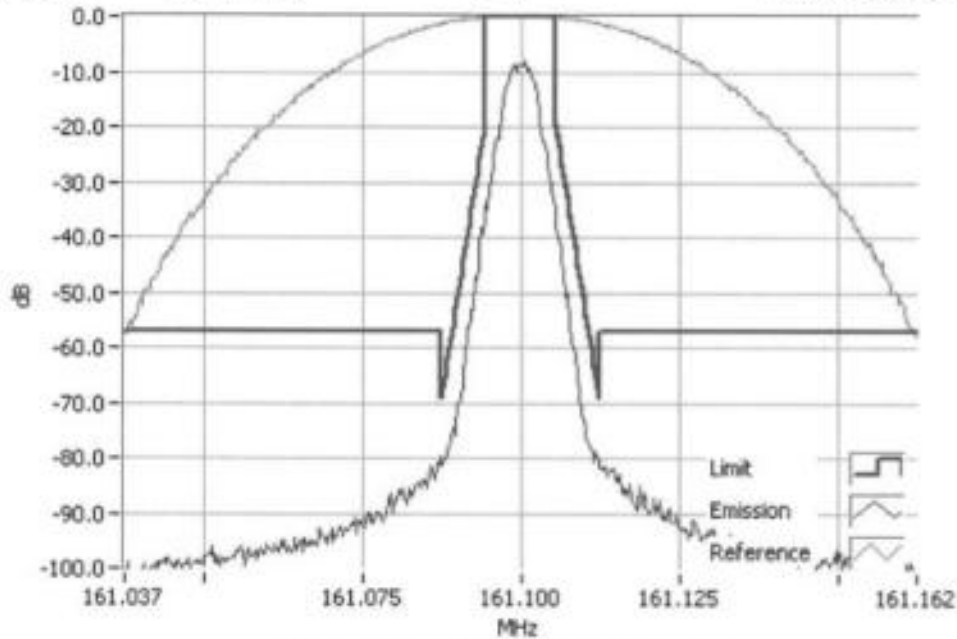
DMR 161.1000MHz Mask D 5W RBW=100Hz, VBW=1000Hz, Detector Mode=Peak Result=Pass
