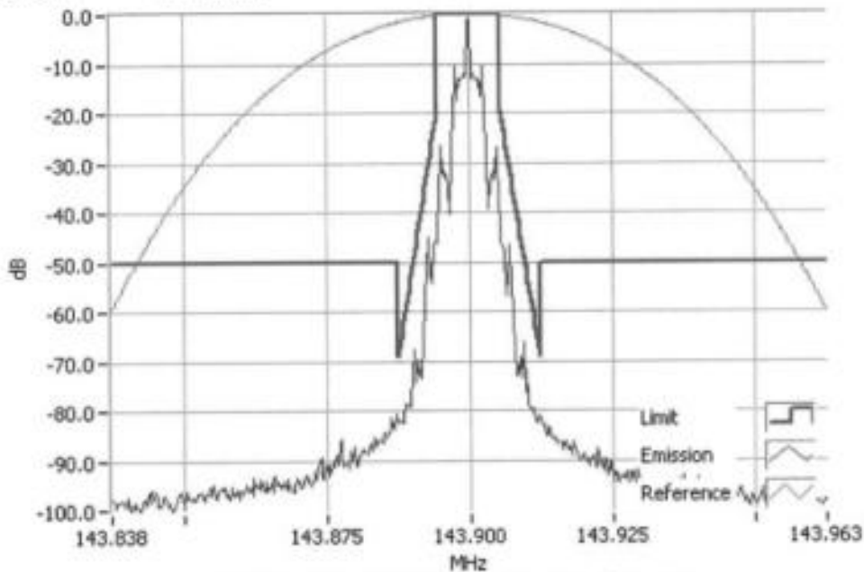
FFSK 2400 143.9000MHz Mask D 1W RBW=100Hz, VBW=1000Hz, Detector Mode=Peak Result=Pass
