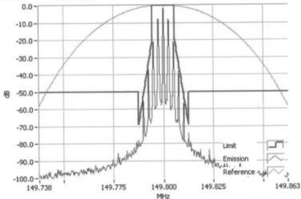
Analogue Modulation 149.8000MHz Mask D 1W RBW=100Hz, VBW=1000Hz, Detector Mode=Peak Result=Pass
