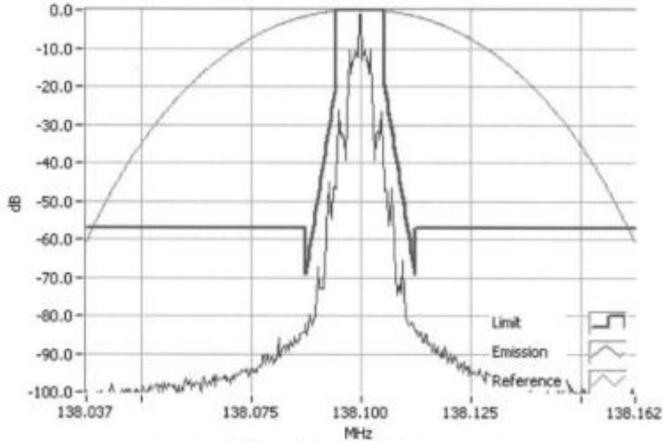
FFSK 2400 138.1000MHz Mask D 5W RBW=100Hz, VBW=1000Hz, Detector Mode=Peak Result=Pass
