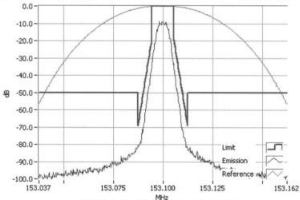
P25 Ph 2 153.1000MHz Mask D 1W RBW=100Hz, VBW=1000Hz, Detector Mode=Peak Result=Pass
