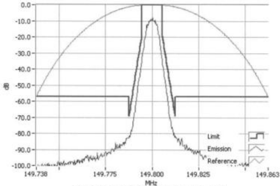
P25 Ph 2 149.8000MHz Mask D 5W RBW=100Hz, VBW=1000Hz, Detector Mode=Peak Result=Pass
