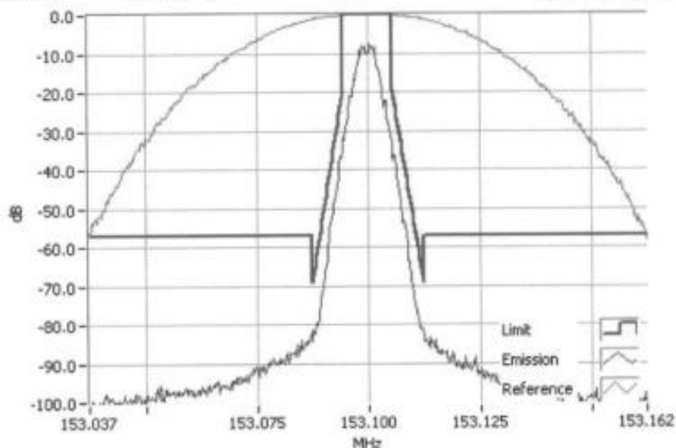
P25 Ph 1 153.1000MHz Mask D 5W RBW=100Hz, VBW=1000Hz, Detector Mode=Peak Result=Pass
