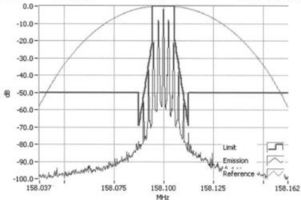
Analogue Modulation 158.1000MHz Mask D 1W RBW=100Hz, VBW=1000Hz, Detector Mode=Peak Result=Pass
