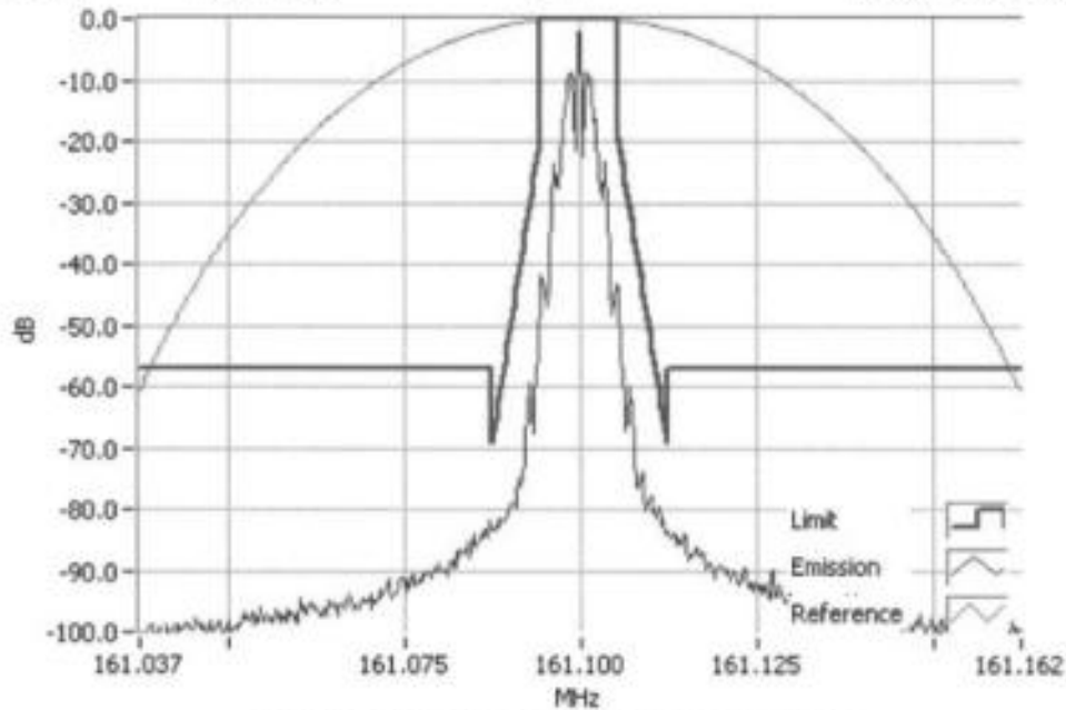
FFSK 1200 161.1000MHz Mask D 5W RBW=100Hz, VBW=1000Hz, Detector Mode=Peak Result=Pass
