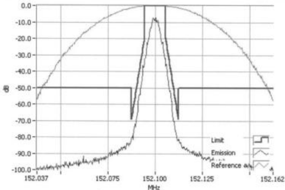
P25 Ph 1 152.1000MHz Mask D 1W RBW=100Hz, VBW=1000Hz, Detector Mode=Peak Result=Pass
