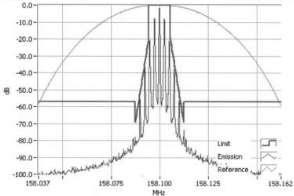
Analogue Modulation 158.1000MHz Mask D 5W RBW=100Hz, VBW=1000Hz, Detector Mode=Peak Result=Pass
