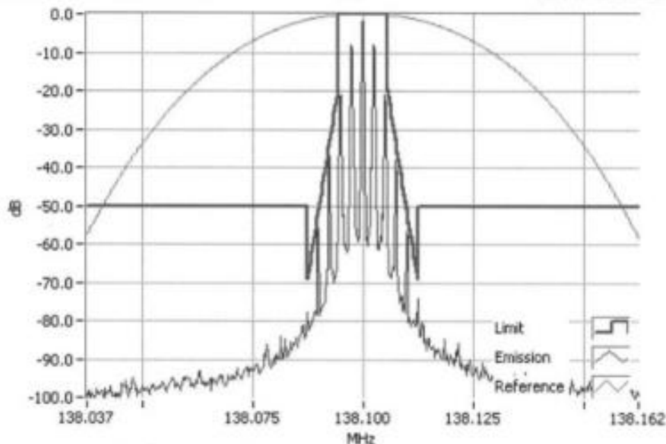
Analogue Modulation 138.1000MHz Mask D 1W RBW=100Hz, VBW=1000Hz, Detector Mode=Peak Result=Pass
