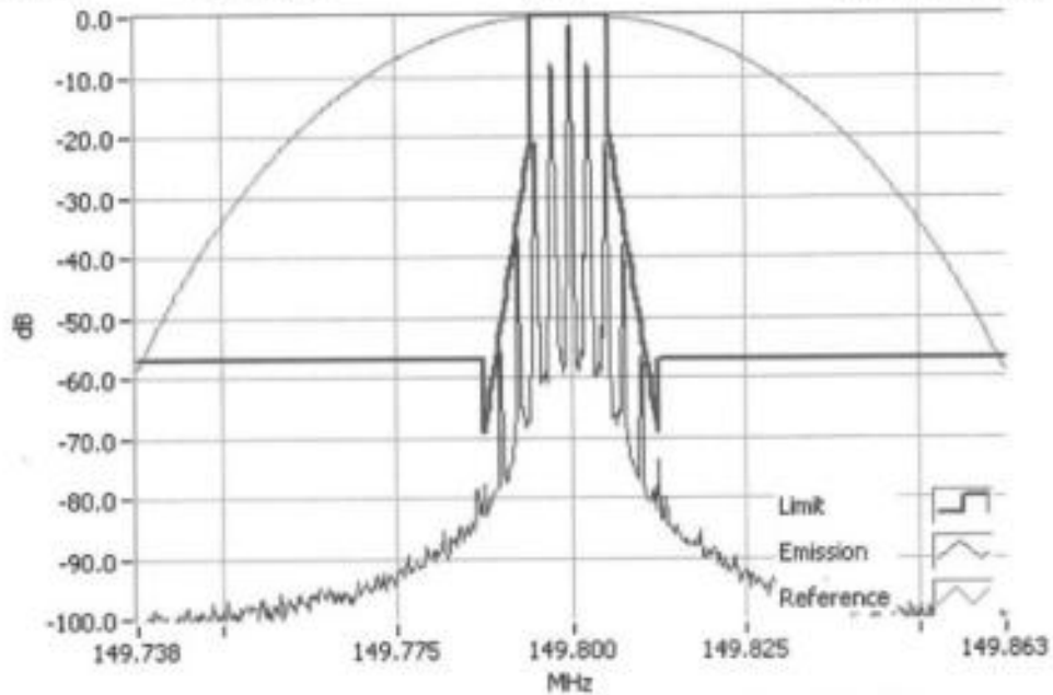
Analogue Modulation 149.8000MHz Mask D 5W RBW=100Hz, VBW=1000Hz, Detector Mode=Peak Result=Pass
