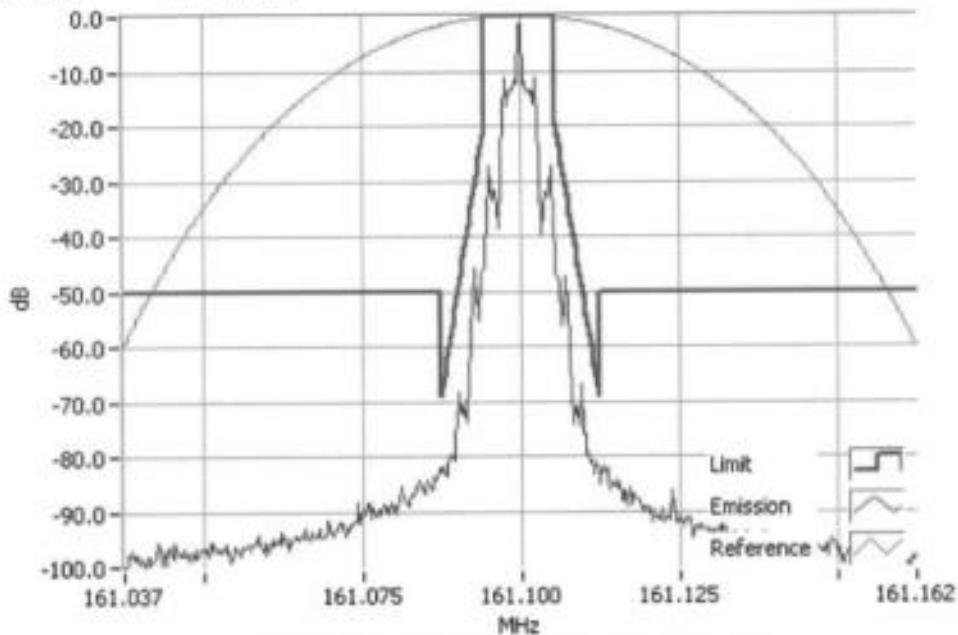
FFSK 2400 161.1000MHz Mask D 1W RBW=100Hz, VBW=1000Hz, Detector Mode=Peak Result=Pass
