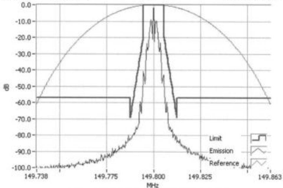
FFSK 1200 149.8000MHz Mask D 5W RBW=100Hz, VBW=1000Hz, Detector Mode=Peak Result=Pass
