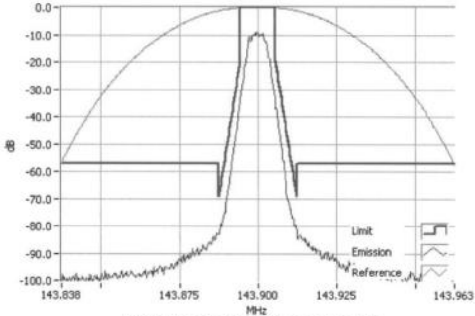
P25 Ph 2 143.9000MHz Mask D 5W RBW=100Hz, VBW=1000Hz, Detector Mode=Peak Result=Pass
