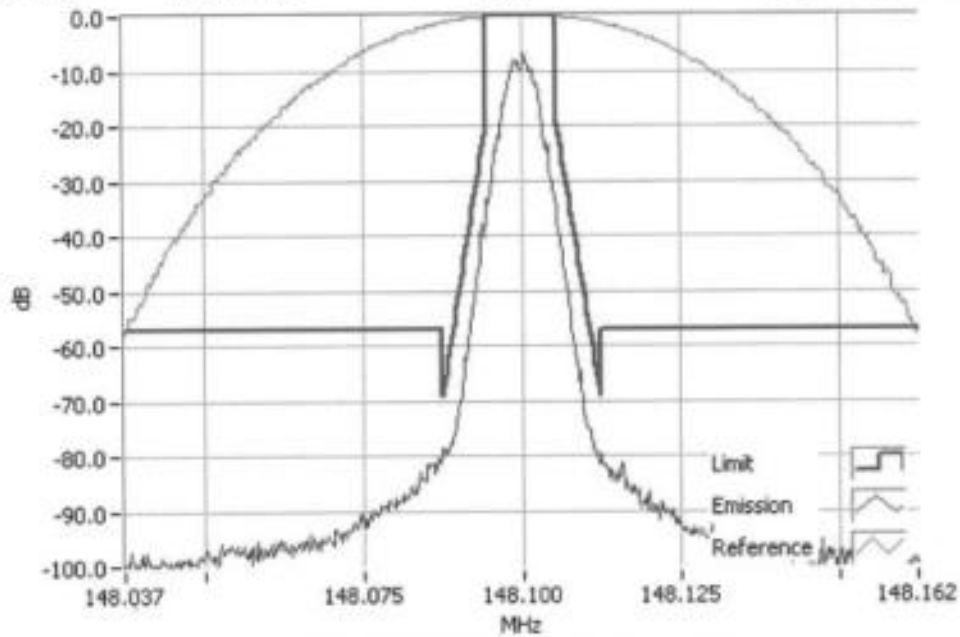
DMR 148.1000MHz Mask D 5W RBW=100Hz, VBW=1000Hz, Detector Mode=Peak Result=Pass
