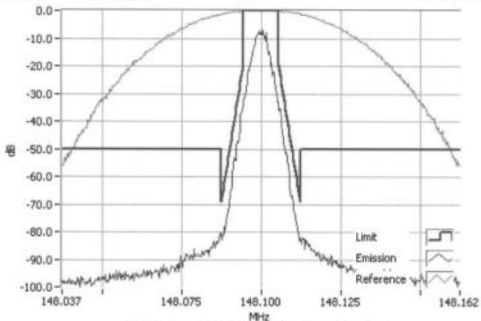
P25 Ph 1 148.1000MHz Mask D 1W RBW=100Hz, VBW=1000Hz, Detector Mode=Peak Result=Pass
