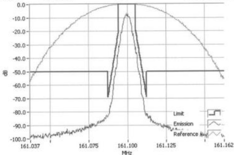
P25 Ph 1 161.1000MHz Mask D 1W RBW=100Hz, VBW=1000Hz, Detector Mode=Peak Result=Pass
