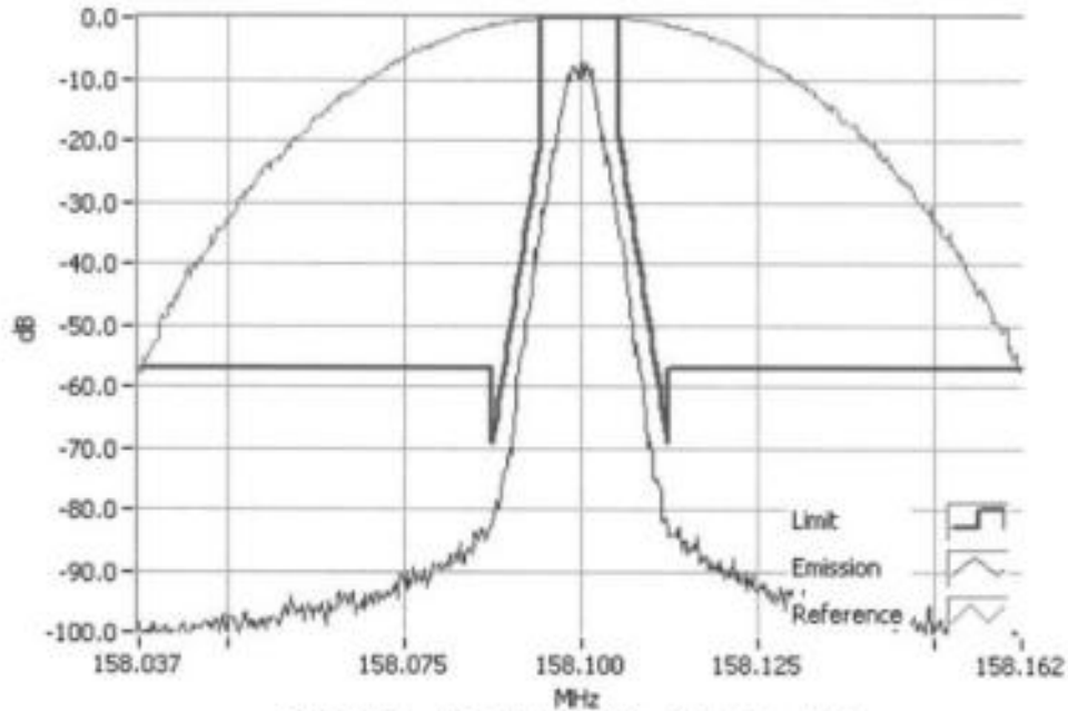
P25 Ph 1 158.1000MHz Mask D 5W RBW=100Hz, VBW=1000Hz, Detector Mode=Peak Result=Pass
