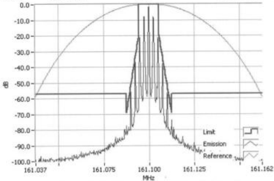
Analogue Modulation 161.1000MHz Mask D 5W RBW=100Hz, VBW=1000Hz, Detector Mode=Peak Result=Pass
