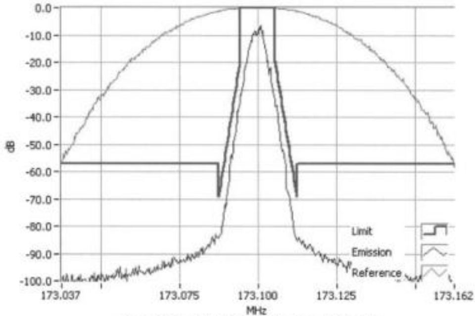
P25 Ph 1 173.1000MHz Mask D 5W RBW=100Hz, VBW=1000Hz, Detector Mode=Peak Result=Pass
