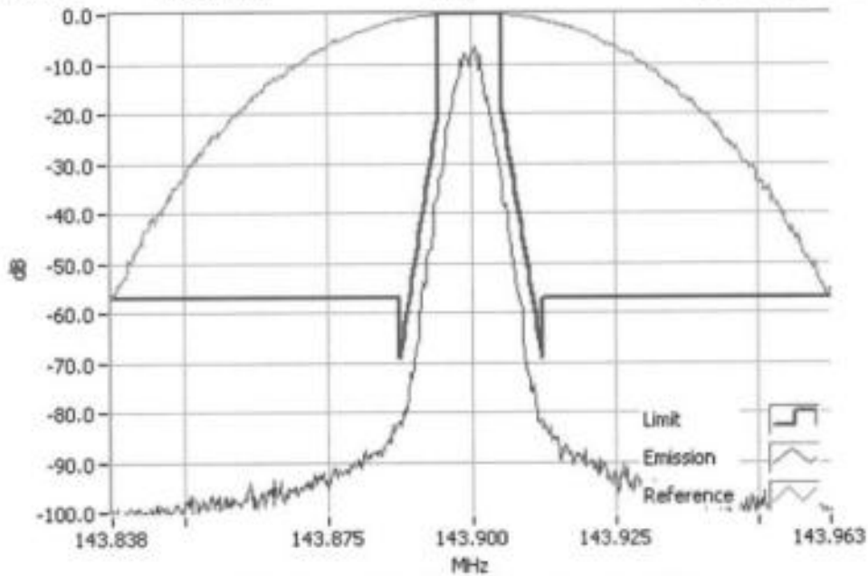
P25 Ph 1 143.9000MHz Mask D 5W RBW=100Hz, VBW=1000Hz, Detector Mode=Peak Result=Pass
