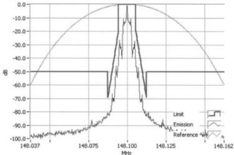
FFSK 2400 148.1000MHz Mask D 1W RBW=100Hz, VBW=1000Hz, Detector Mode=Peak Result=Pass
