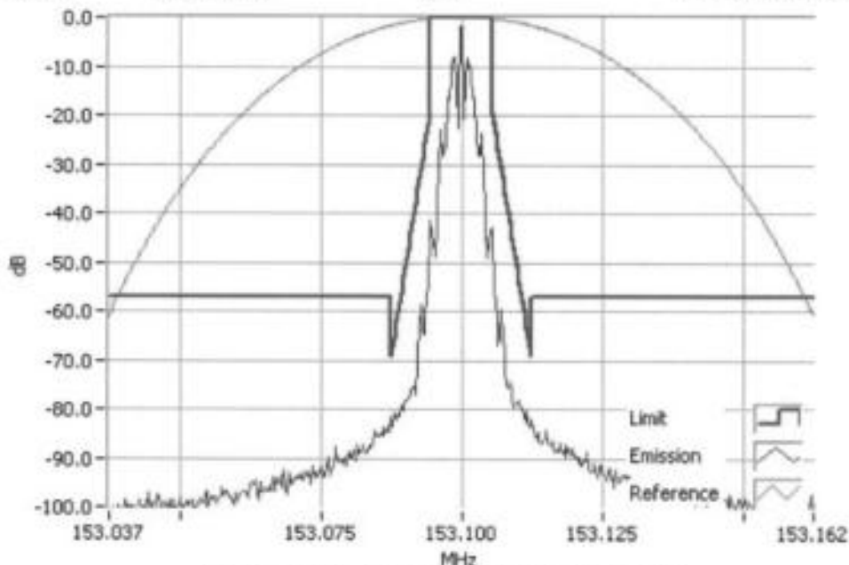
FFSK 1200 153.1000MHz Mask D 5W RBW=100Hz, VBW=1000Hz, Detector Mode=Peak Result=Pass
