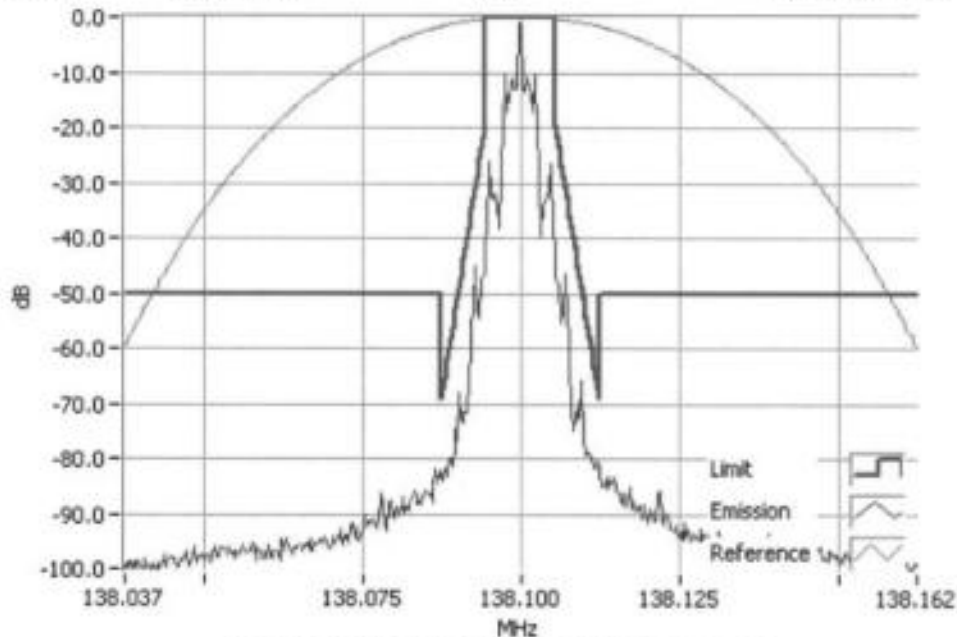
FFSK 2400 138.1000MHz Mask D 1W RBW=100Hz, VBW=1000Hz, Detector Mode=Peak Result=Pass
