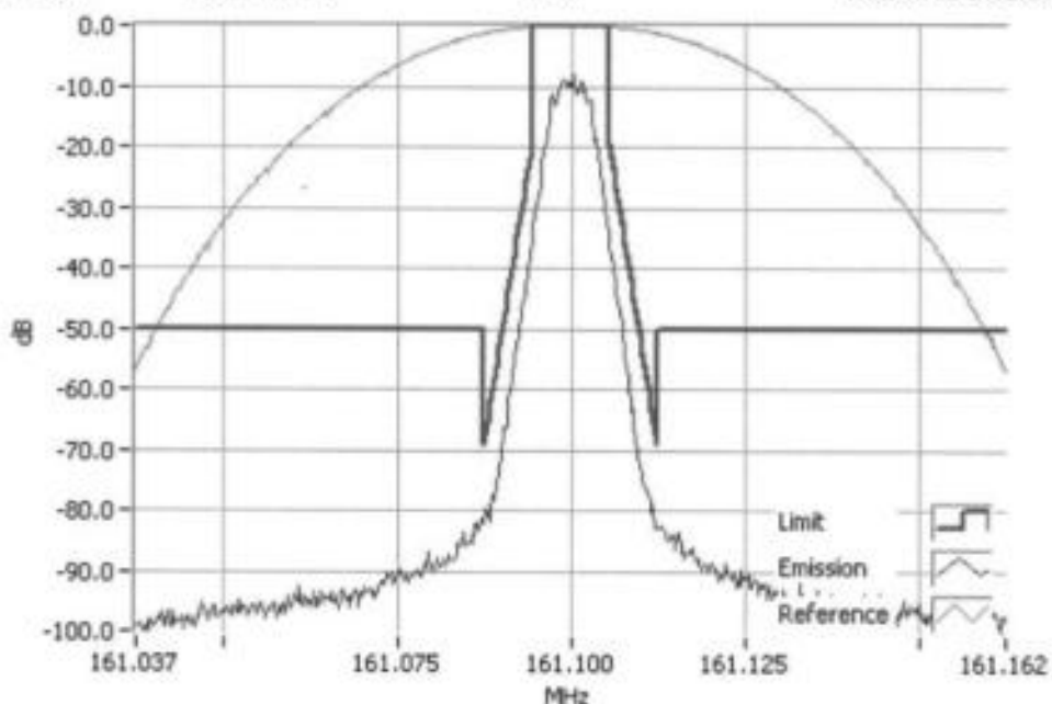
P25 Ph 2 161.1000MHz Mask D 1W RBW=100Hz, VBW=1000Hz, Detector Mode=Peak Result=Pass
