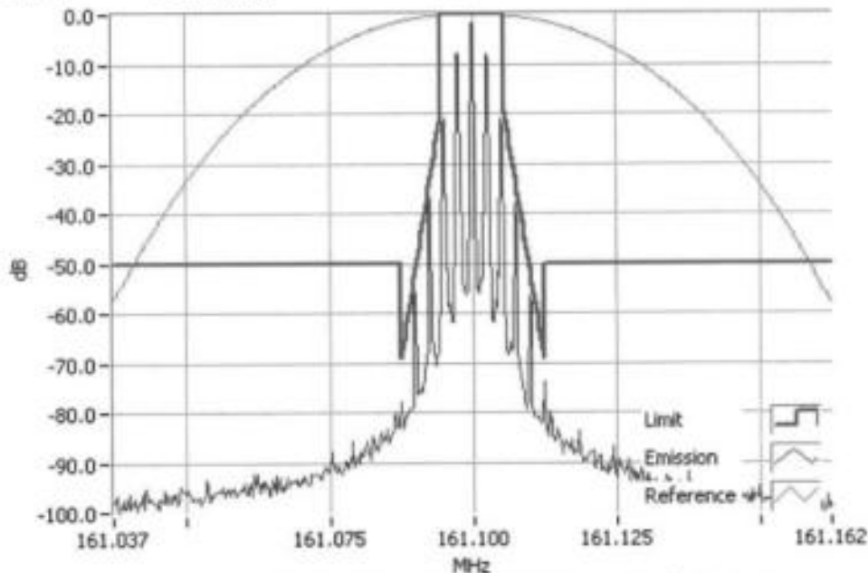
Analogue Modulation 161.1000MHz Mask D 1W RBW=100Hz, VBW=1000Hz, Detector Mode=Peak Result=Pass
