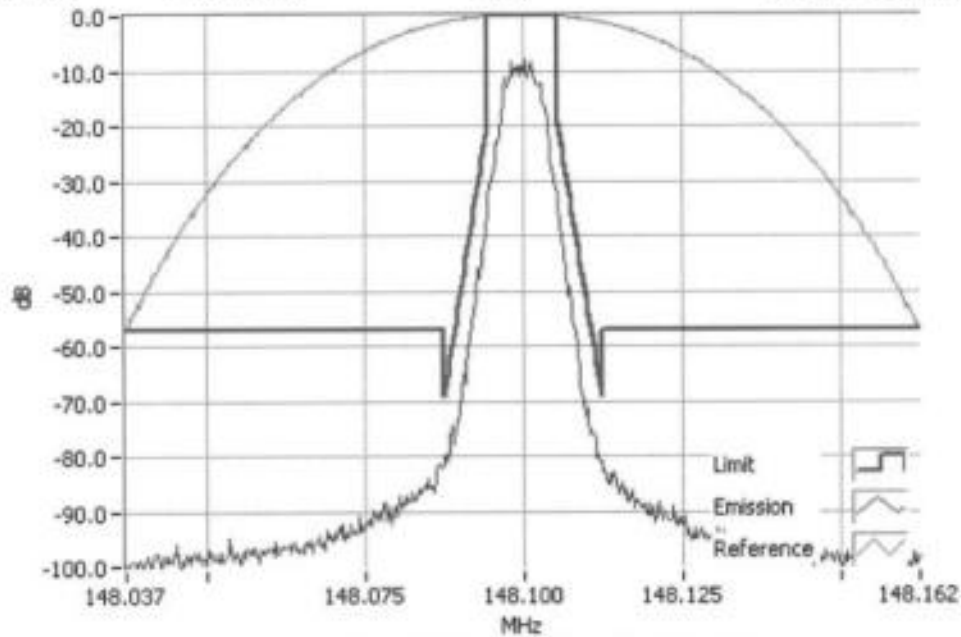
P25 Ph 2 148.1000MHz Mask D 5W RBW=100Hz, VBW=1000Hz, Detector Mode=Peak Result=Pass
