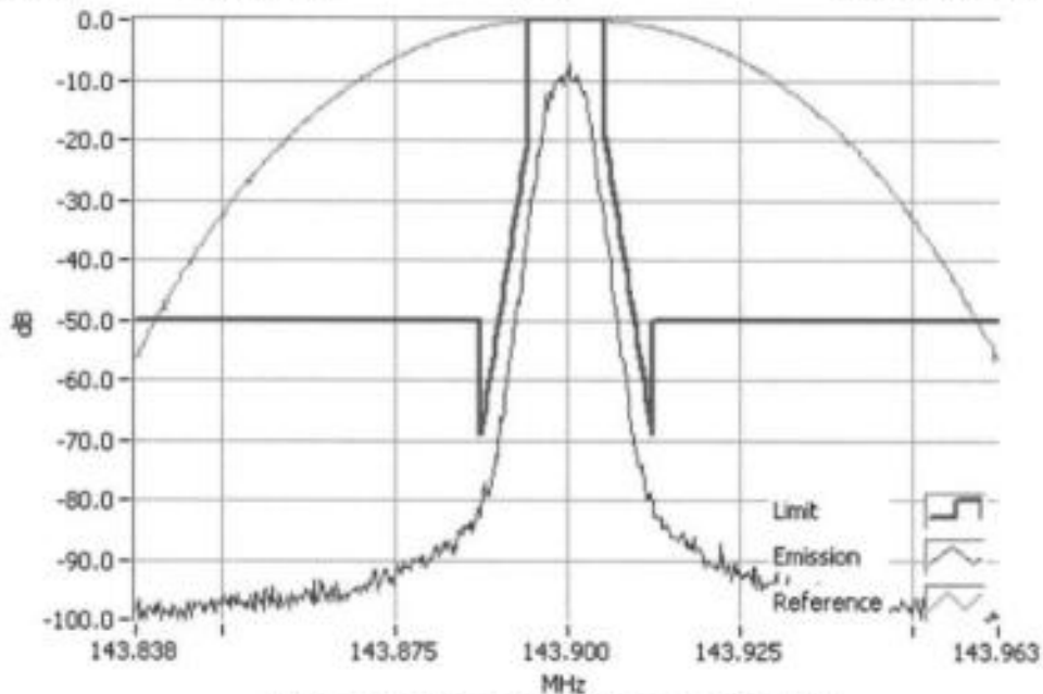
P25 Ph 2 143.9000MHz Mask D 1W RBW=100Hz, VBW=1000Hz, Detector Mode=Peak Result=Pass
