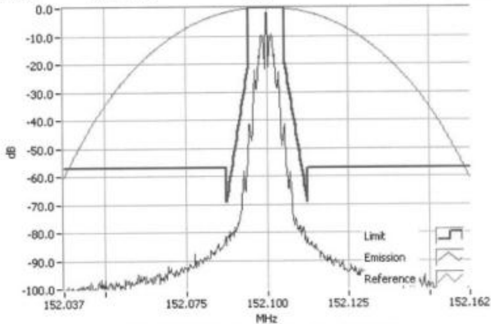
FFSK 1200 152.1000MHz Mask D 5W RBW=100Hz, VBW=1000Hz, Detector Mode=Peak Result=Pass
