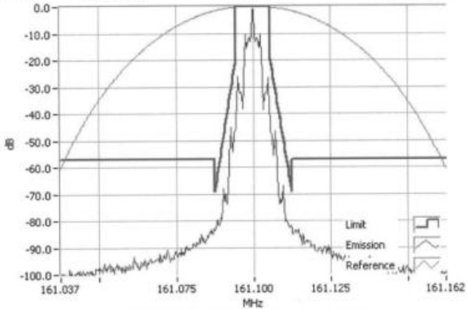
FFSK 2400 161.1000MHz Mask D 5W RBW=100Hz, VBW=1000Hz, Detector Mode=Peak Result=Pass
