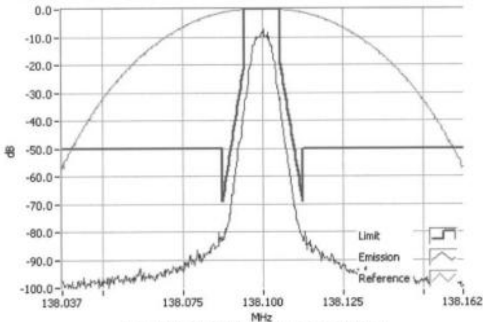
P25 Ph 2 138.1000MHz Mask D 1W RBW=100Hz, VBW=1000Hz, Detector Mode=Peak Result=Pass
