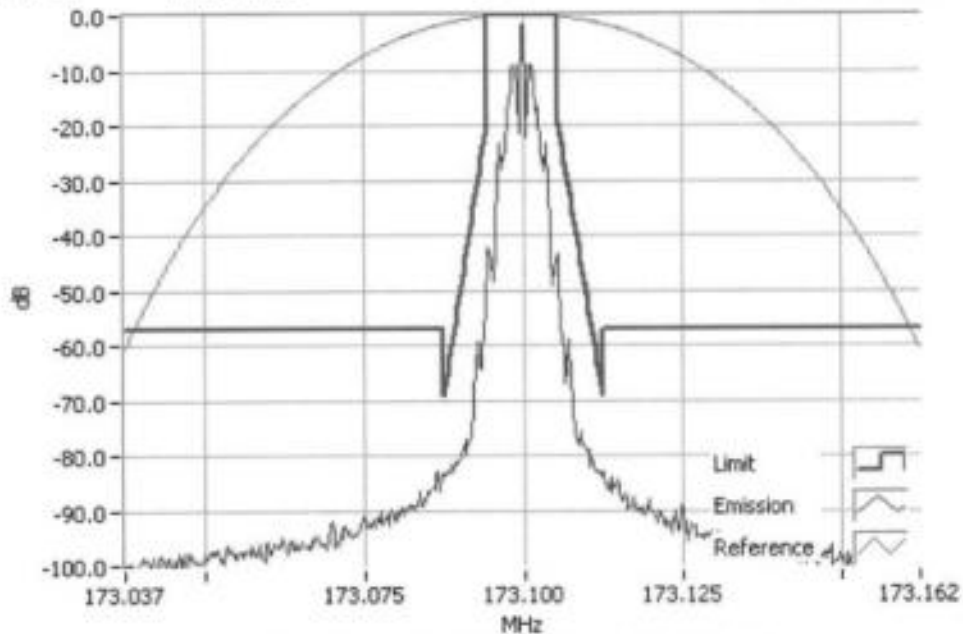
FFSK 1200 173.1000MHz Mask D 5W RBW=100Hz, VBW=1000Hz, Detector Mode=Peak Result=Pass
