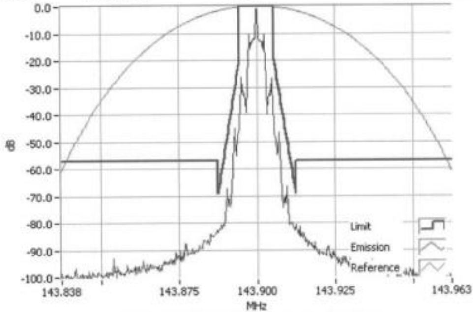
FFSK 2400 143.9000MHz Mask D 5W RBW=100Hz, VBW=1000Hz, Detector Mode=Peak Result=Pass
