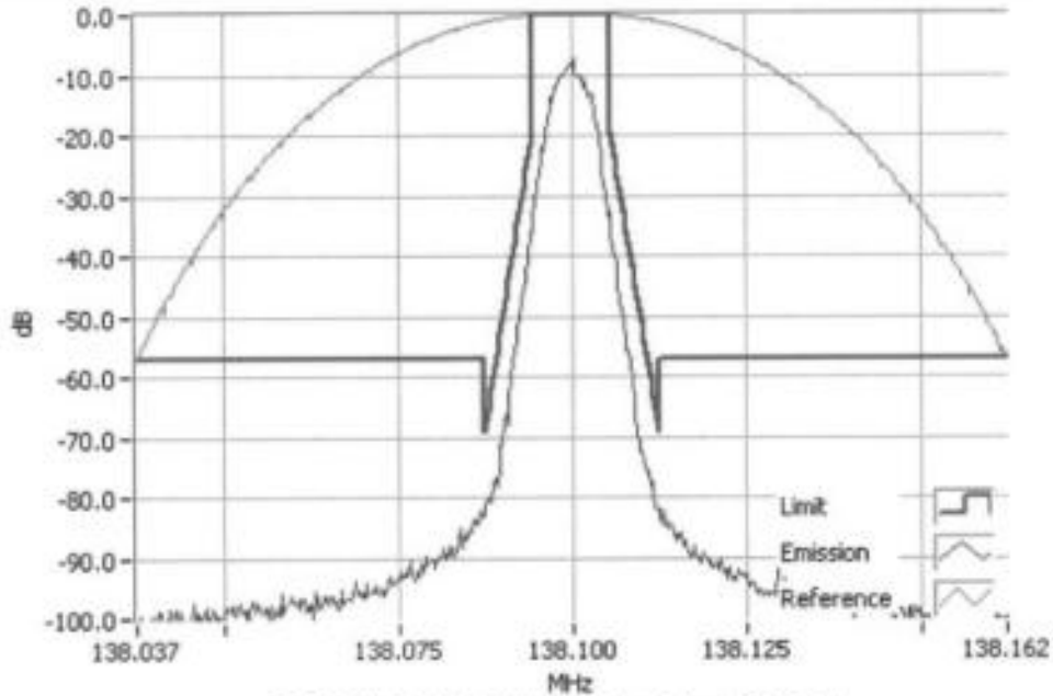
P25 Ph 2 138.1000MHz Mask D 5W RBW=100Hz, VBW=1000Hz, Detector Mode=Peak Result=Pass
