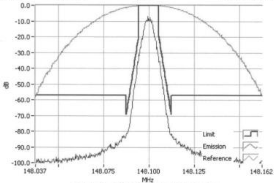
P25 Ph 1 148.1000MHz Mask D 5W RBW=100Hz, VBW=1000Hz, Detector Mode=Peak Result=Pass
