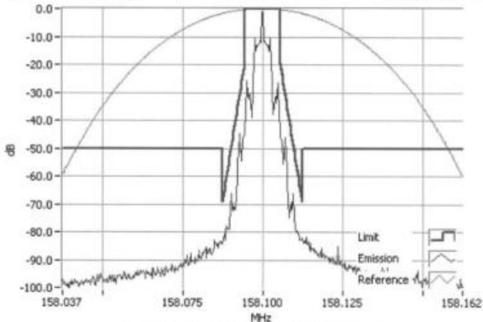
FFSK 2400 158.1000MHz Mask D 1W RBW=100Hz, VBW=1000Hz, Detector Mode=Peak Result=Pass
