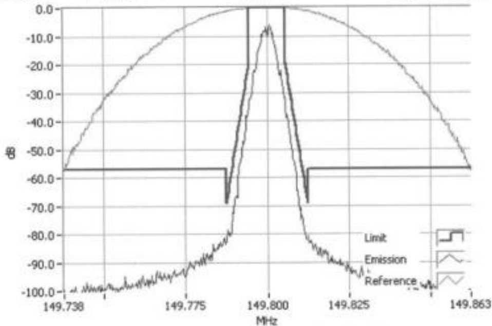
P25 Ph 1 149.8000MHz Mask D 5W RBW=100Hz, VBW=1000Hz, Detector Mode=Peak Result=Pass
