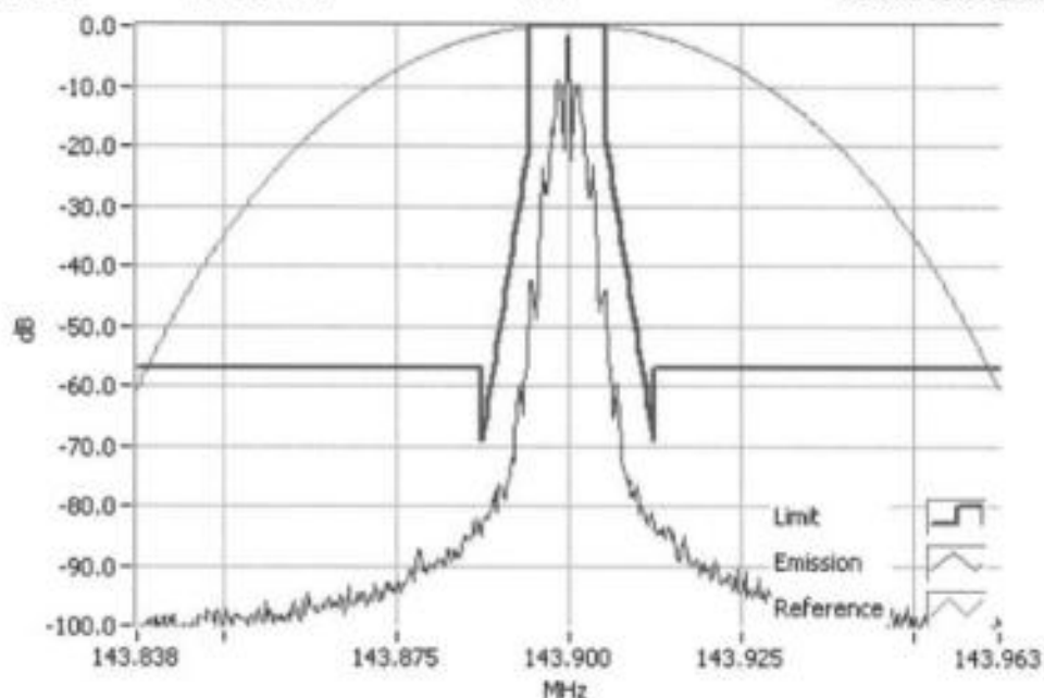
FFSK 1200 143.9000MHz Mask D 5W RBW=100Hz, VBW=1000Hz, Detector Mode=Peak Result=Pass
