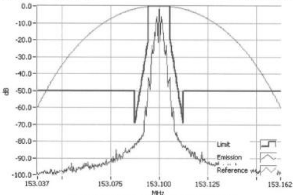
FFSK 1200 153.1000MHz Mask D 1W RBW=100Hz, VBW=1000Hz, Detector Mode=Peak Result=Pass
