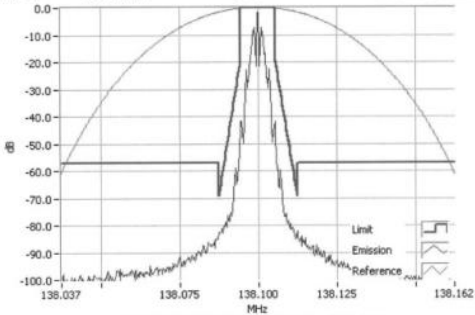
FFSK 1200 138.1000MHz Mask D 5W RBW=100Hz, VBW=1000Hz, Detector Mode=Peak Result=Pass
