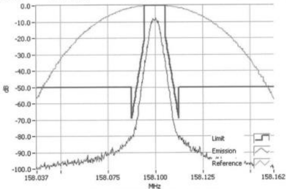
DMR 158.1000MHz Mask D 1W RBW=100Hz, VBW=1000Hz, Detector Mode=Peak Result=Pass
