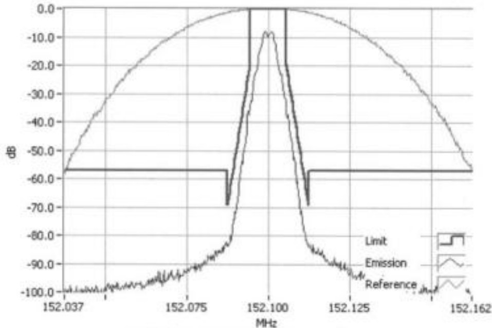
P25 Ph 1 152.1000MHz Mask D 5W RBW=100Hz, VBW=1000Hz, Detector Mode=Peak Result=Pass
