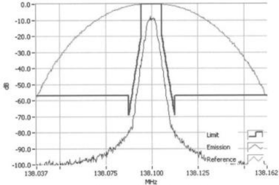
DMR 138.1000MHz Mask D 5W RBW=100Hz, VBW=1000Hz, Detector Mode=Peak Result=Pass
