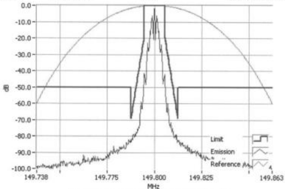
FFSK 1200 149.8000MHz Mask D 1W RBW=100Hz, VBW=1000Hz, Detector Mode=Peak Result=Pass
