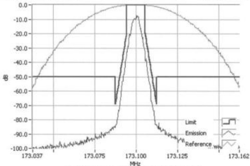
P25 Ph 1 173.1000MHz Mask D 1W RBW=100Hz, VBW=1000Hz, Detector Mode=Peak Result=Pass
