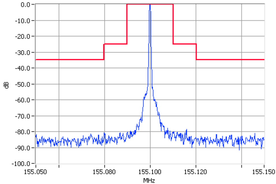
Unmodulated 155.1000MHz Mask B 5W Pass RBW=300Hz VBW=3000Hz
