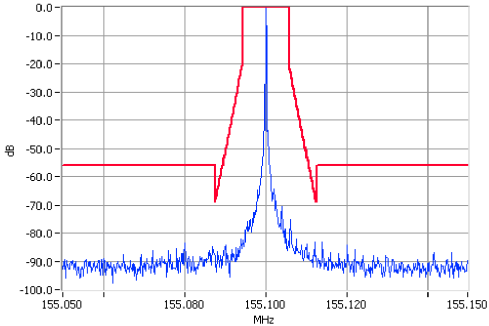
Unmodulated 155.1000MHz Mask D 5W Pass RBW=100Hz VBW=1000Hz
