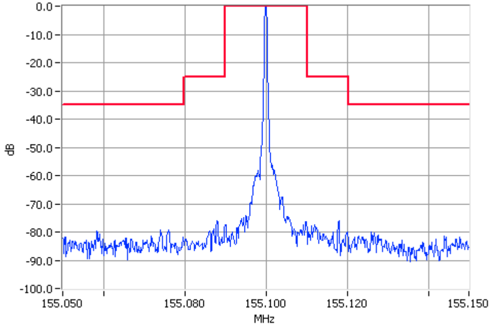
Unmodulated 155.1000MHz Mask B 1W Pass RBW=300Hz VBW=3000Hz
