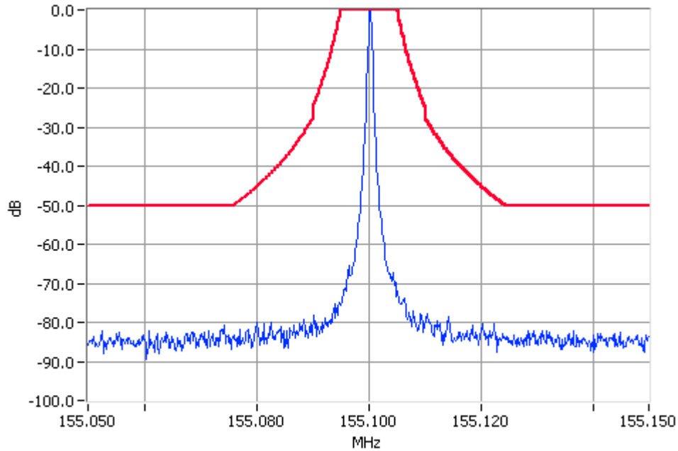
Unmodulated 155.1000MHz Mask C 5W Pass RBW=300Hz VBW=3000Hz
