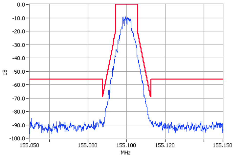
Digital Modulation 155.1000MHz Mask D 5W Pass RBW=100Hz VBW=1000Hz
