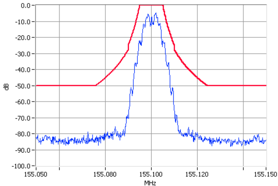
Digital Modulation 155.1000MHz Mask C 5W Pass RBW=300Hz VBW=3000Hz
