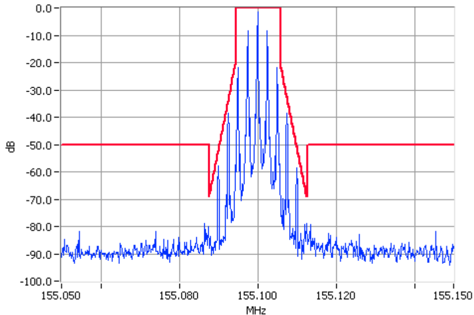
Analogue Modulation 155.1000MHz Mask D 1W Pass RBW=100Hz VBW=1000Hz
