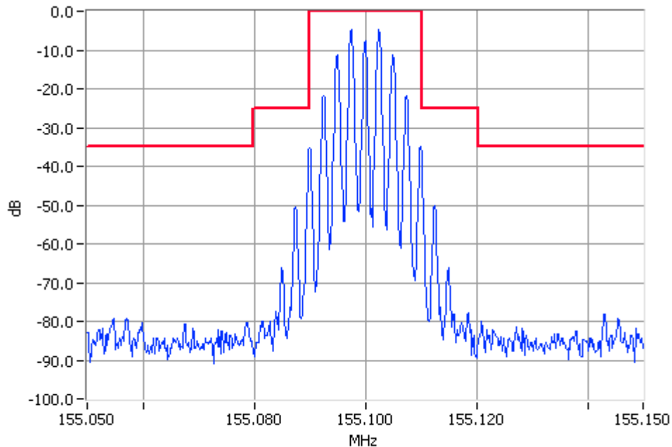
Analogue Modulation 155.1000MHz Mask B 5W Pass RBW=300Hz VBW=3000Hz
