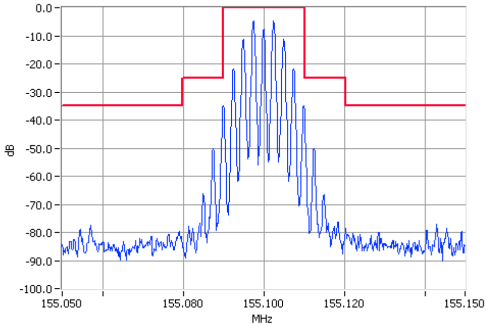
Analogue Modulation 155.1000MHz Mask B 1W Pass RBW=300Hz VBW=3000Hz
