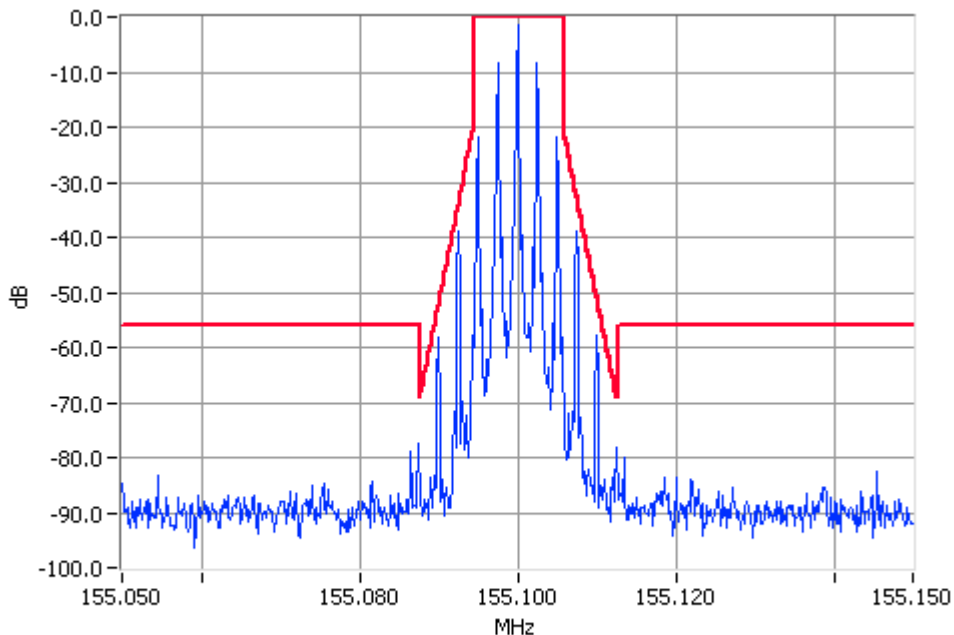
Analogue Modulation 155.1000MHz Mask D 5W Pass RBW=100Hz VBW=1000Hz
