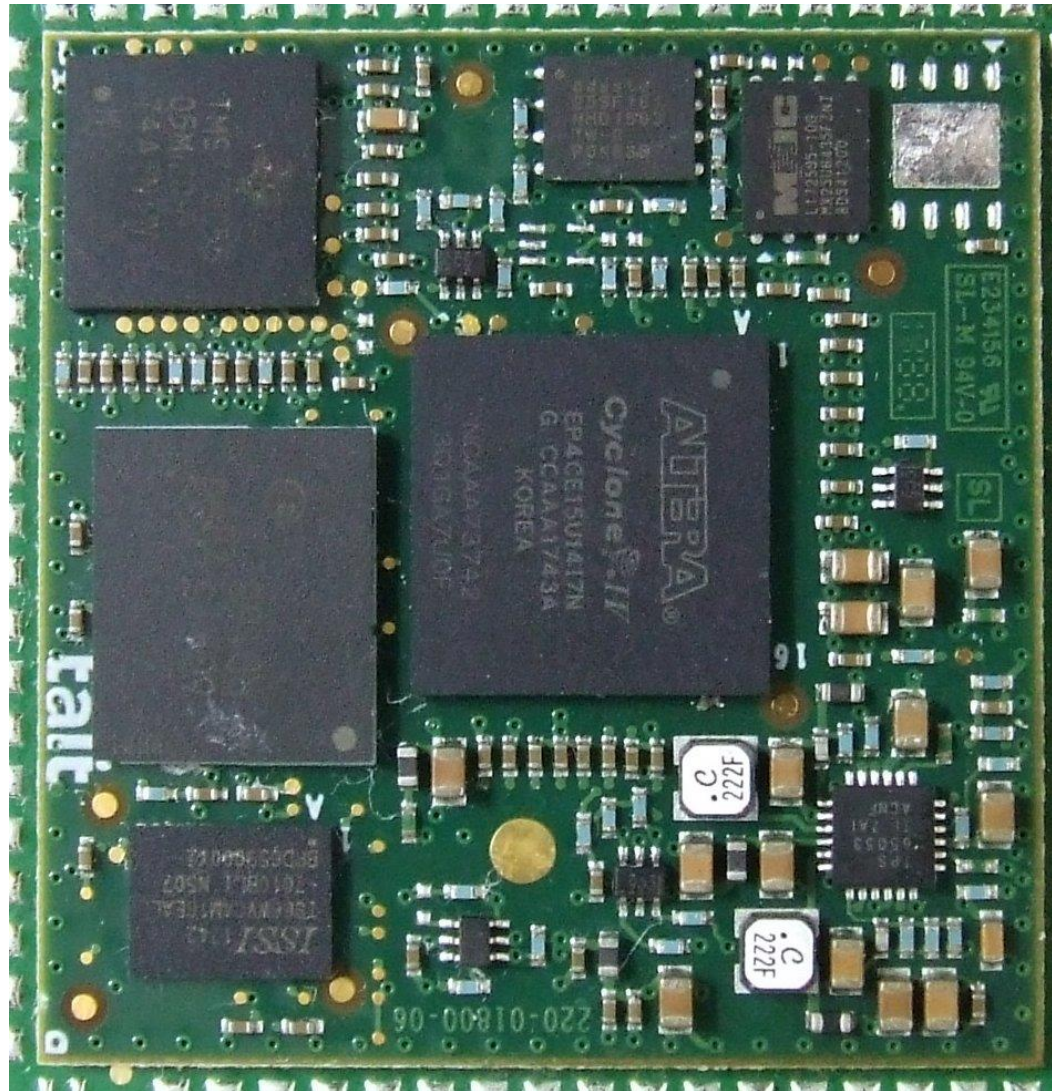
Photograph 03: Radio – Main PCB top without shields, close up of IC devices
