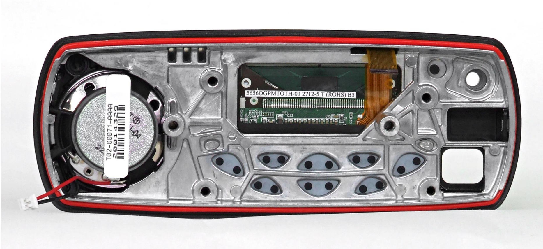
Photograph 08: Control Head – Internal with main PCB removed
