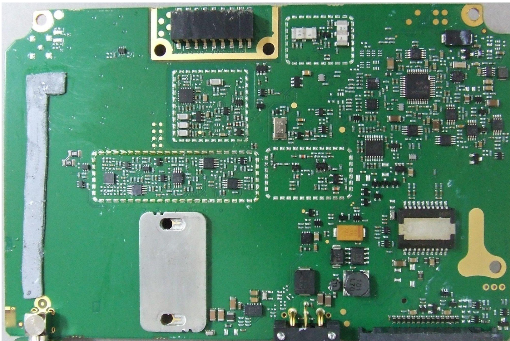
Photograph 05: Radio - Main PCB bottom without shields
