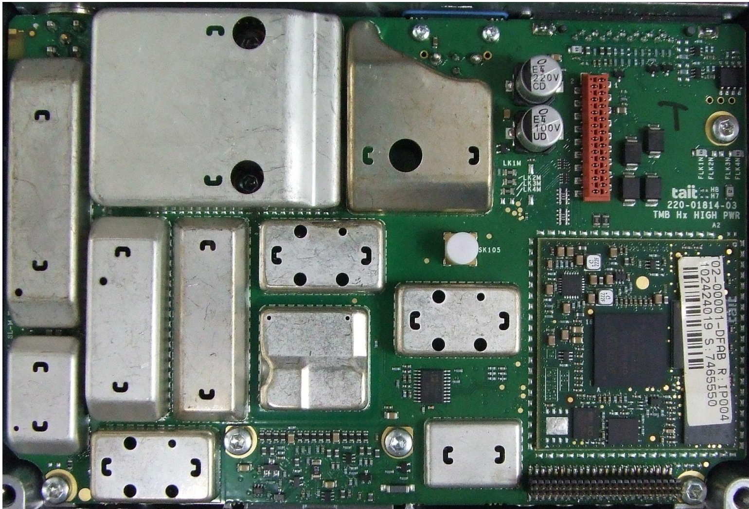
Photograph 01: Radio - Main PCB top with shields
