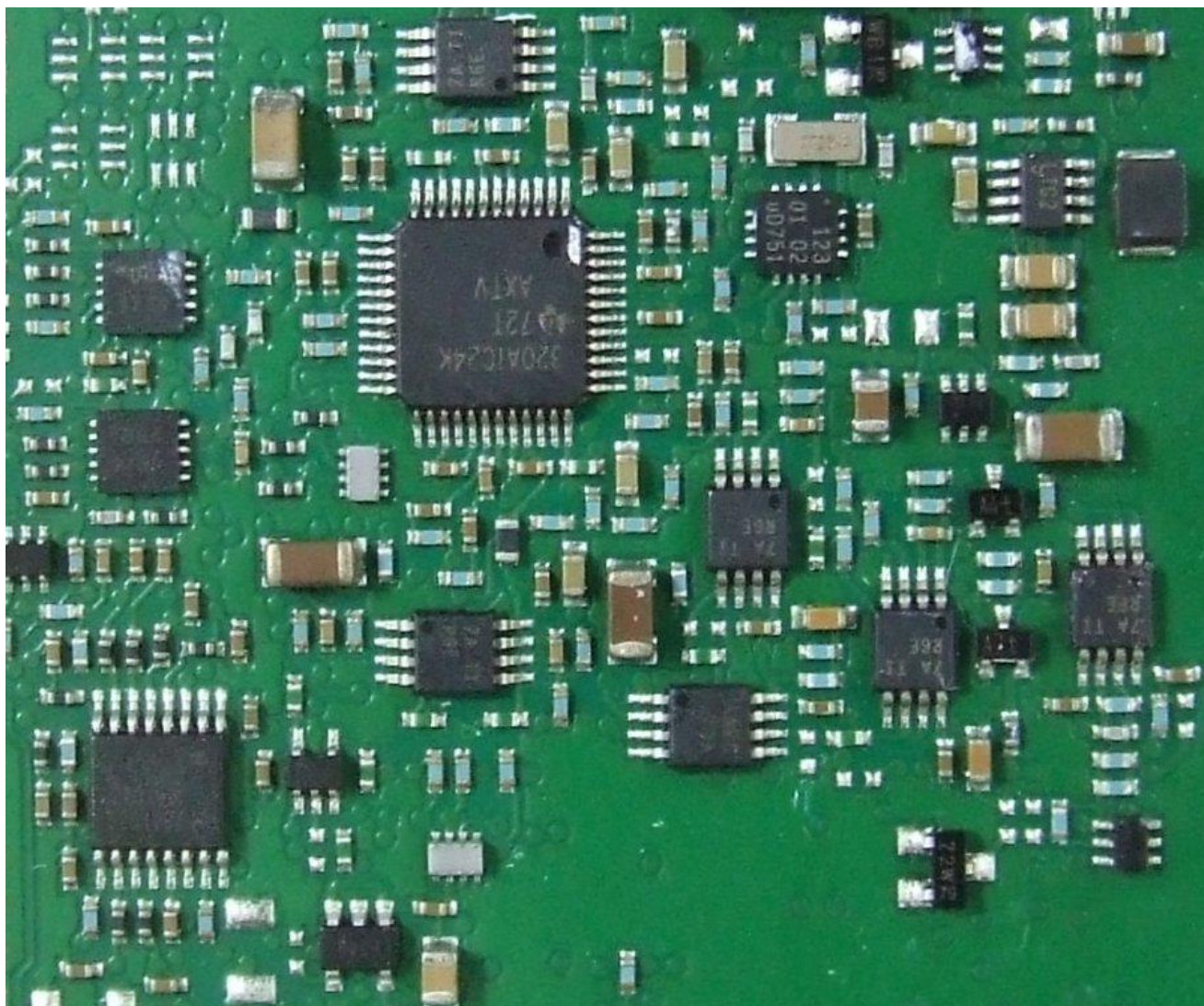
Photograph 06: Radio – Main PCB bottom without shields, close up of IC devices
