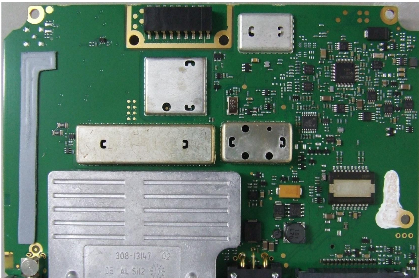
Photograph 04: Radio - Main PCB bottom with shields
