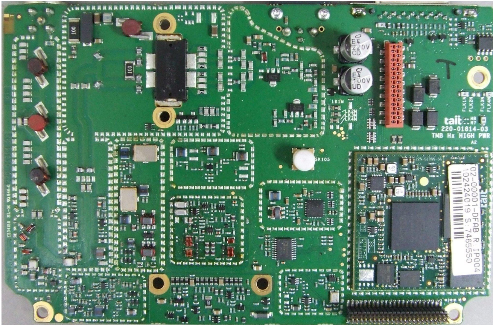
Photograph 02: Radio - Main PCB top without shields
