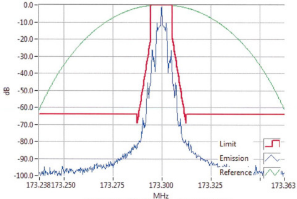
FFSK2400 173.3000MHz Mask D 25W RBW=100Hz, VBW=1000Hz, Detector Mode=Peak Result=Pass
