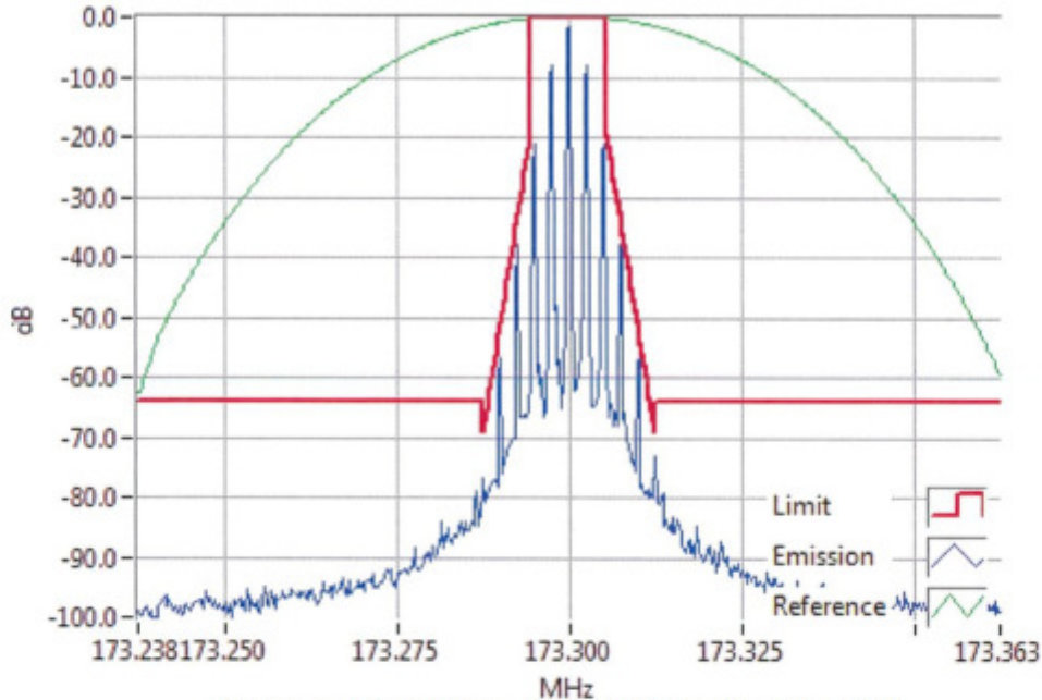
Analogue Modulation 173.3000MHz Mask D 25W RBW=100Hz, VBW=1000Hz, Detector Mode=Peak Result=Pass
