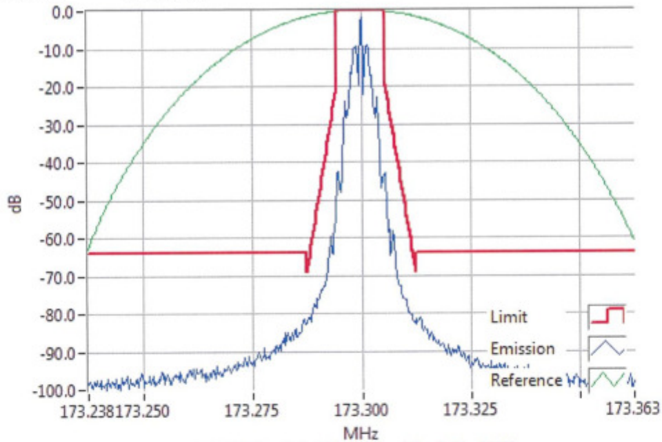
FFSK1200 173.3000MHz Mask D 25W RBW=100Hz, VBW=1000Hz, Detector Mode=Peak Result=Pass
