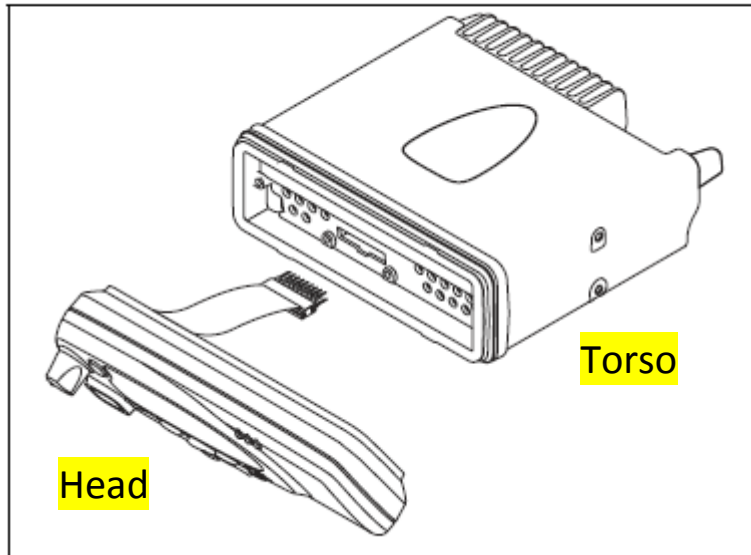
Figure 4.1 Mounting the control head
