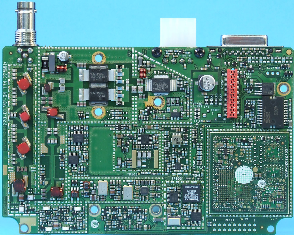
TMAC0C Internal PCB Top View (cans removed)
