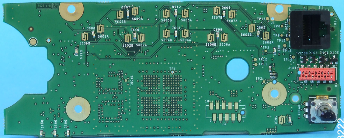
TMAC0C Internal Controlhead PCB Front View
