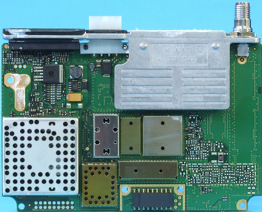
TMAC0C Internal PCB Bottom Side
