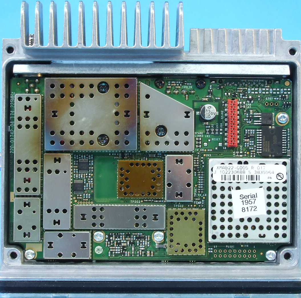
TMAC0C Internal Top View
