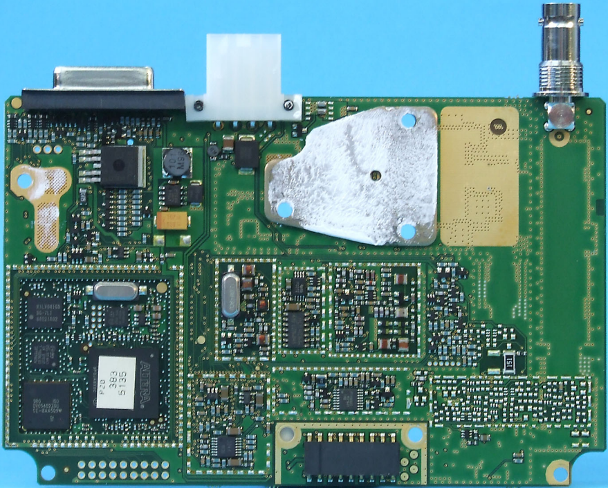
TMAC0C Internal PCB Bottom View (cans removed)
