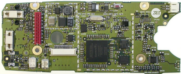
TMAC0C Internal Controlhead Rear View (No Cans)
