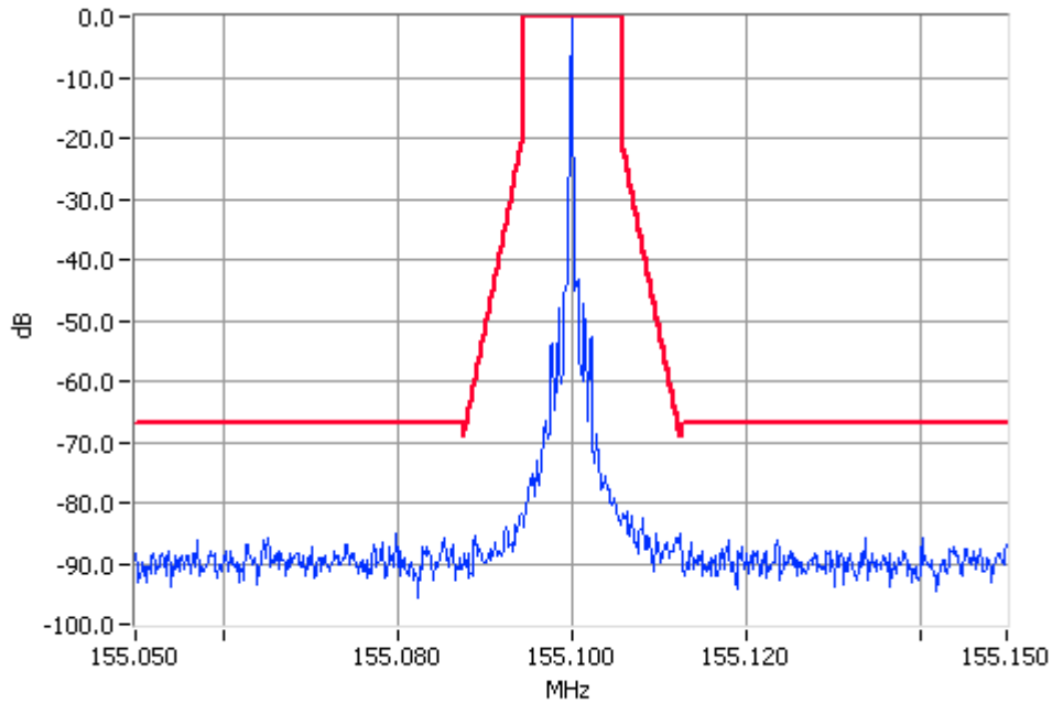
Unmodulated 155.100MHz Mask D 50W Pass RBW=100Hz VBW=1000Hz
