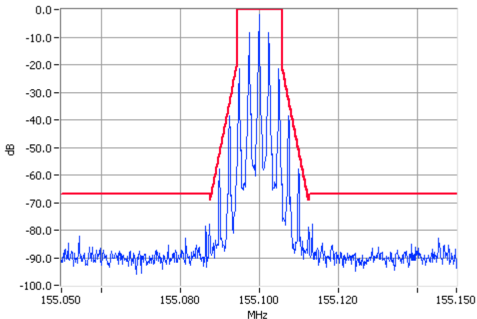
Analogue Modulation 155.100MHz Mask D 50W Pass
