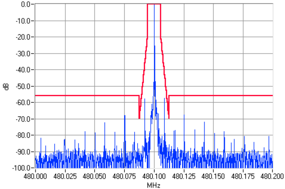
Unmodulated 480.1000MHz Mask D 4W Pass
