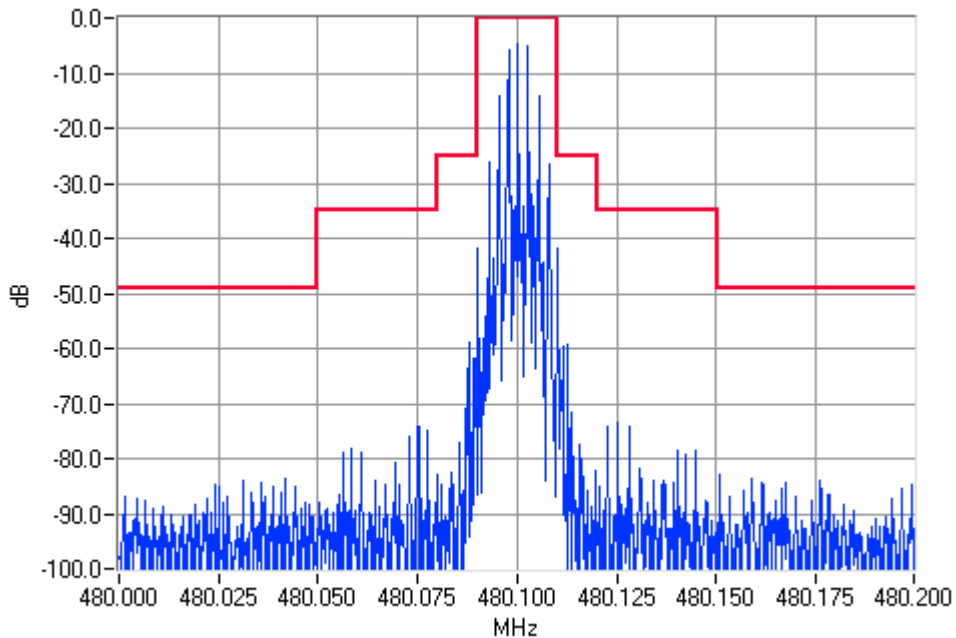
Analogue Modulation 480.1000MHz Mask B 4W Pass
