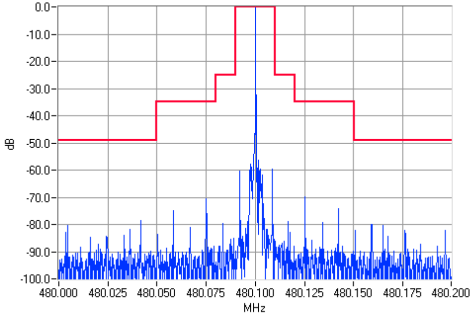
Unmodulated 480.1000MHz Mask B 4W Pass
