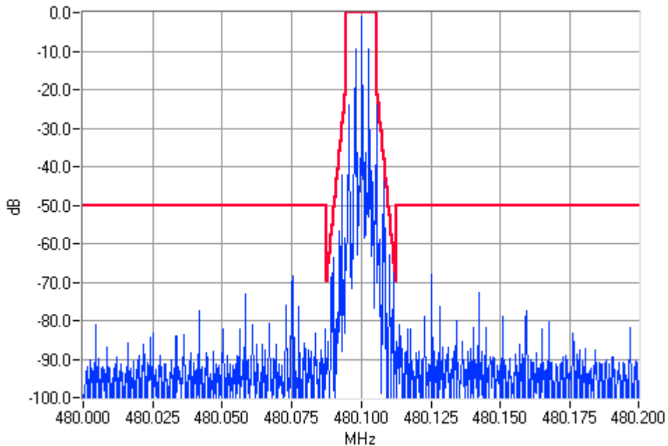
Analogue Modulation 480.1000MHz Mask D 1W Pass
