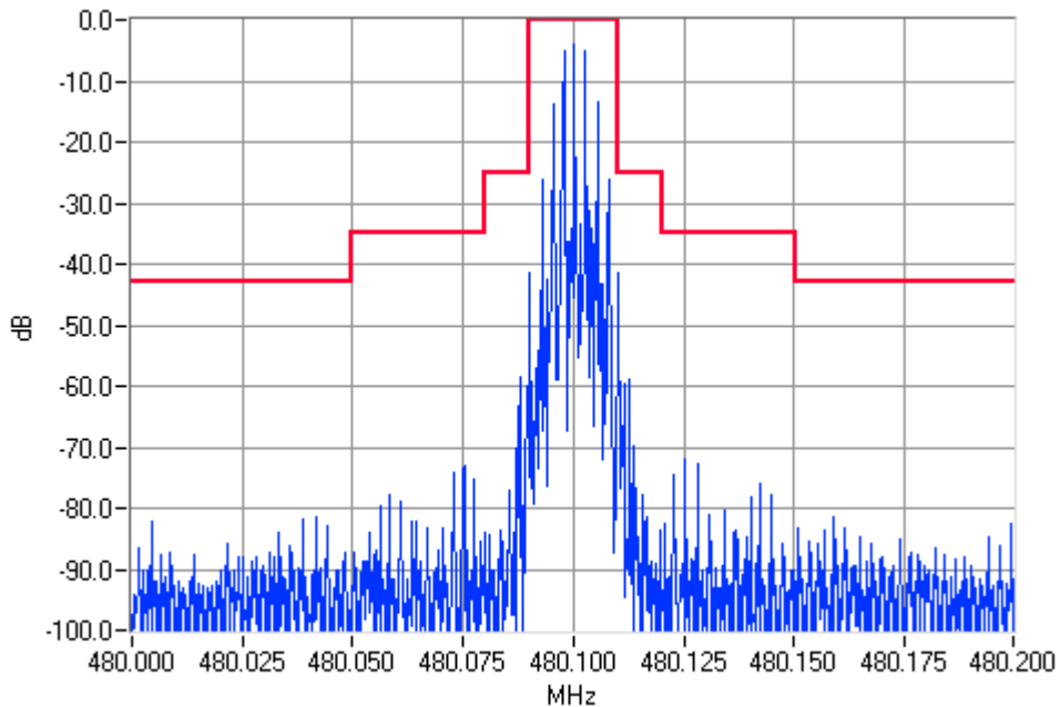
Analogue Modulation 480.1000MHz Mask B 1W Pass
