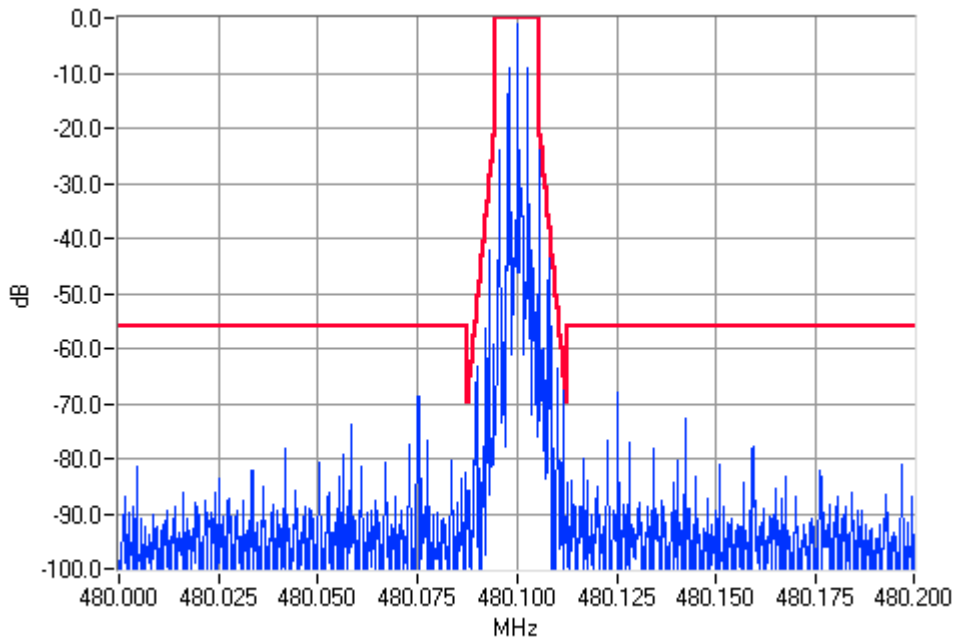
Analogue Modulation 480.1000MHz Mask D 4W Pass
