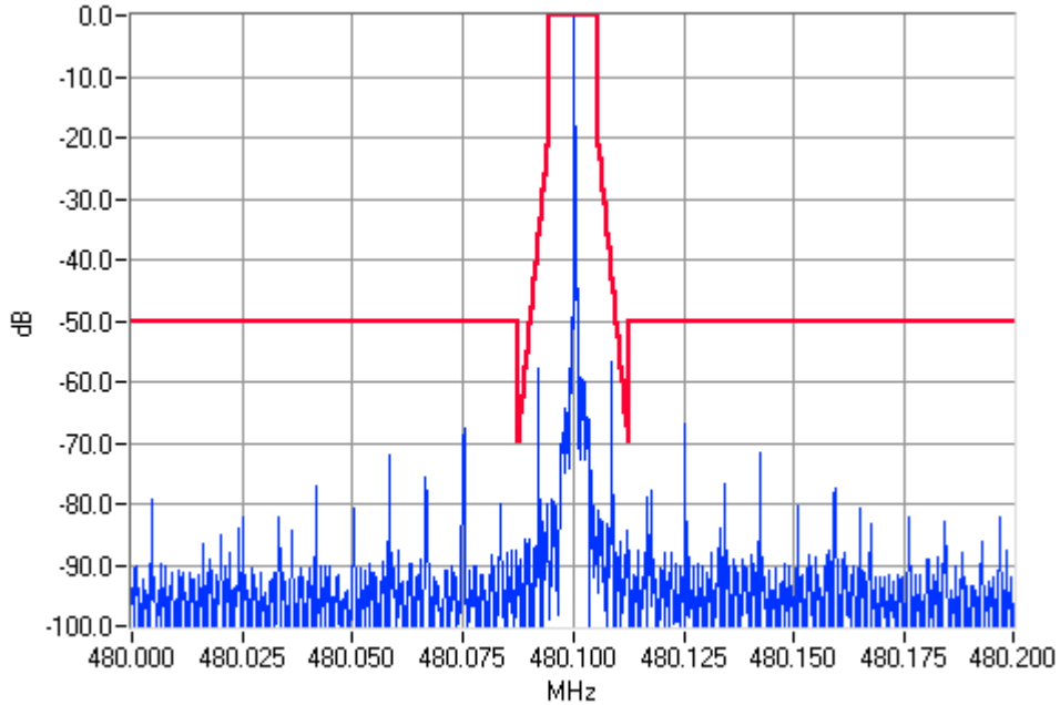
Unmodulated 480.1000MHz Mask D 1W Pass
