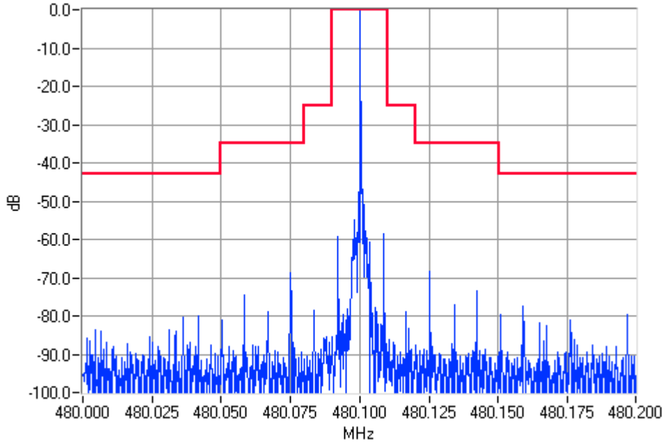
Unmodulated 480.1000MHz Mask B 1W Pass
