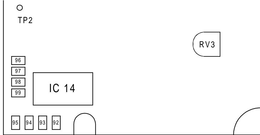
Figure 6 Location of Zero Ohm Resistors
