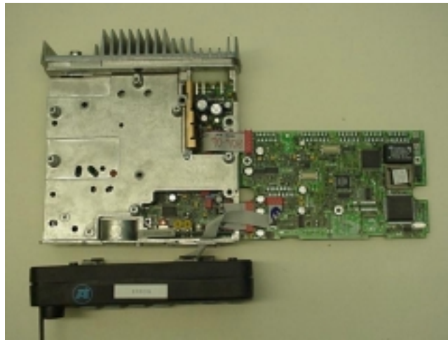
TOP of logic PCB and chassis, looking from top
