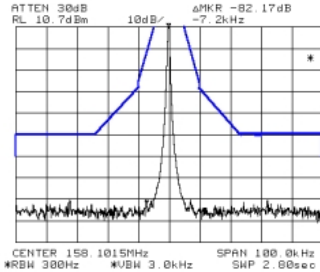
Tarf 1541 @ 50W, 158.10 MHz with T837-26-1021 unmodulated
