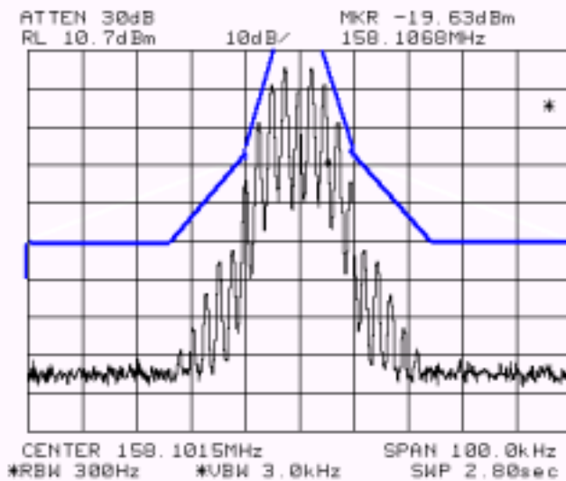
Tarf 1541@ 50W ,158.1 MHz with T837-26-1021 modulated
