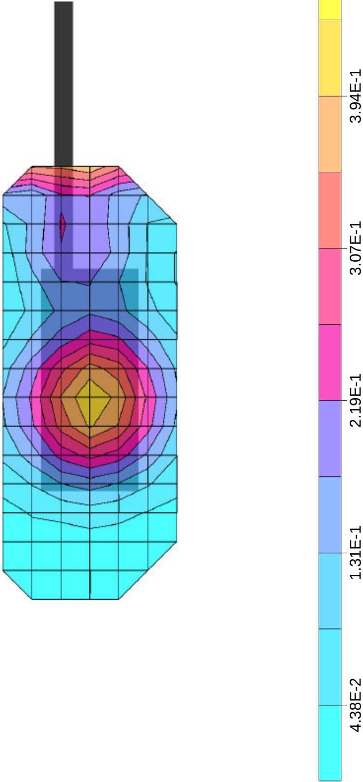
SAR Measurement Plot 14
