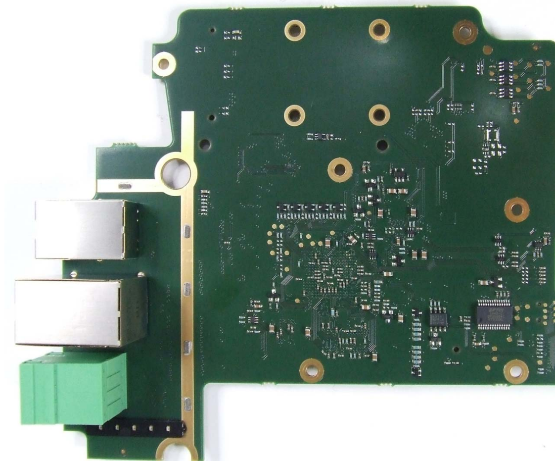
Photograph 03: Main PCB bottom
