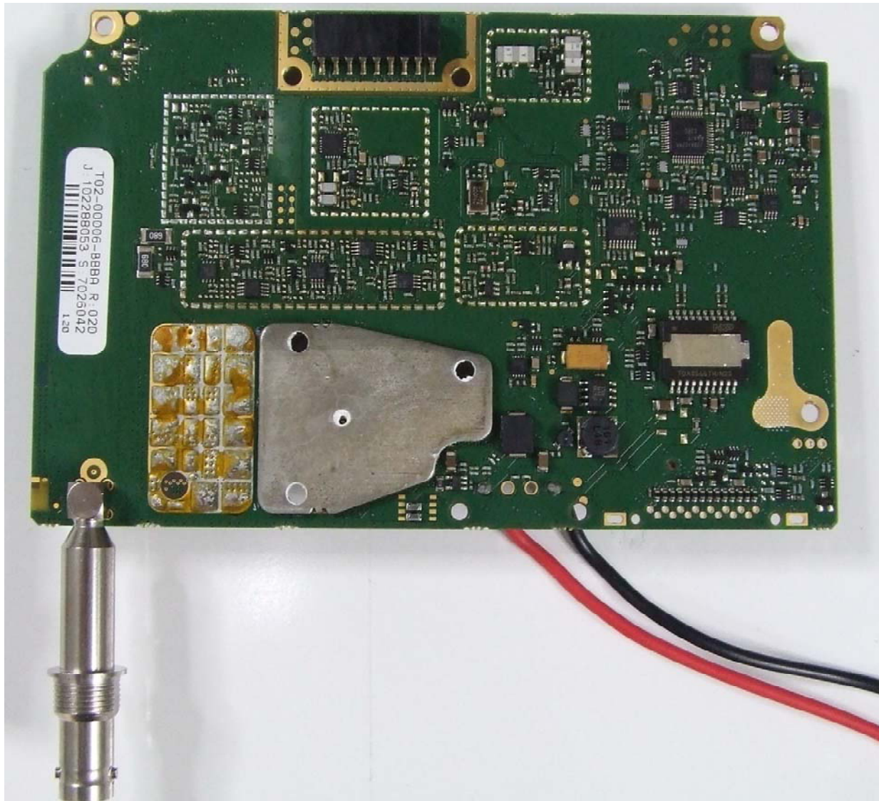
Photograph 07: RF PCB bottom without shields
