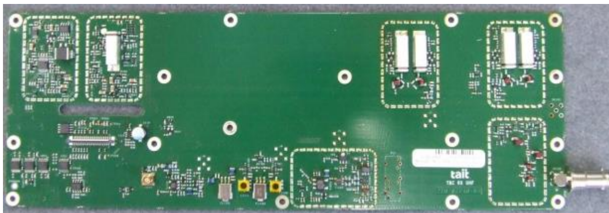
Photograph 18: Receiver Board (RXB) – Top (cans off)
