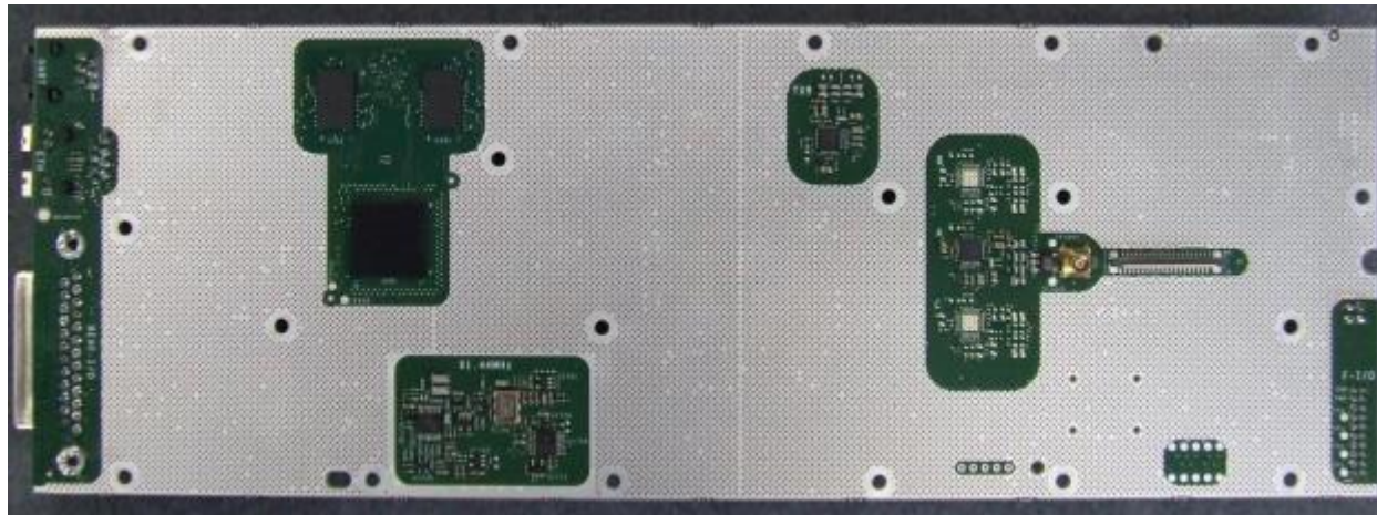
Photograph 16: Reciter Control Board (RCB) – Bottom
