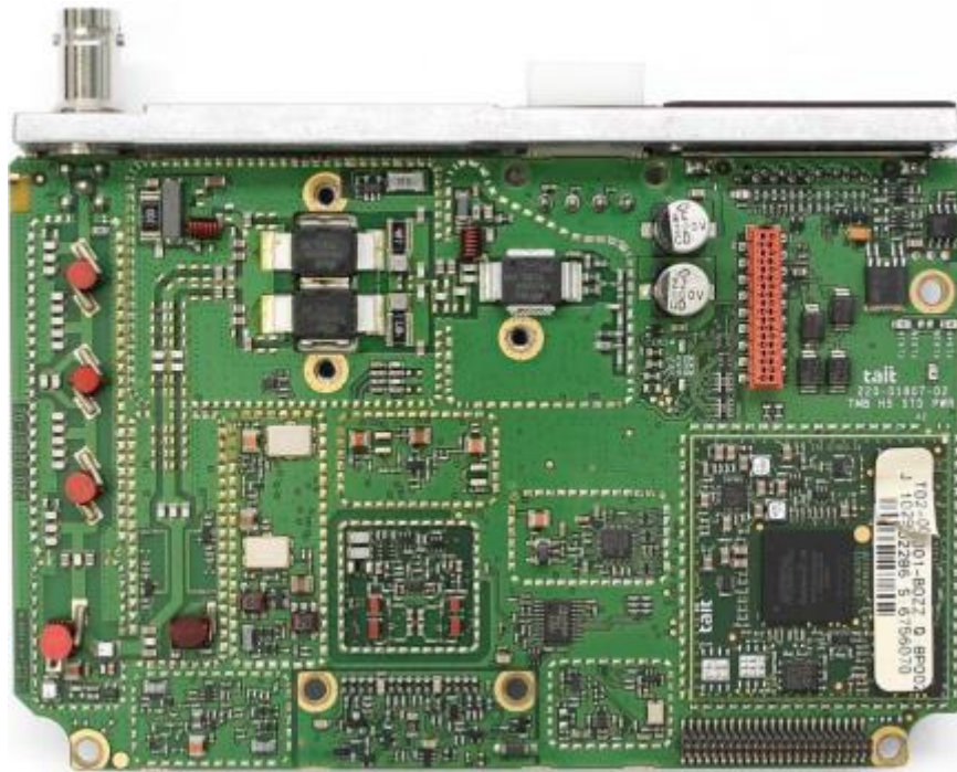
Photograph 12: Power Amplifier PCB – Top, cans off
