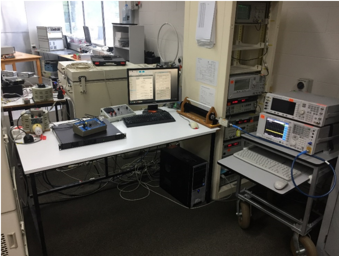
TRANSMITTER SPURIOUS EMISSIONS (CONDUCTED) SETUP
