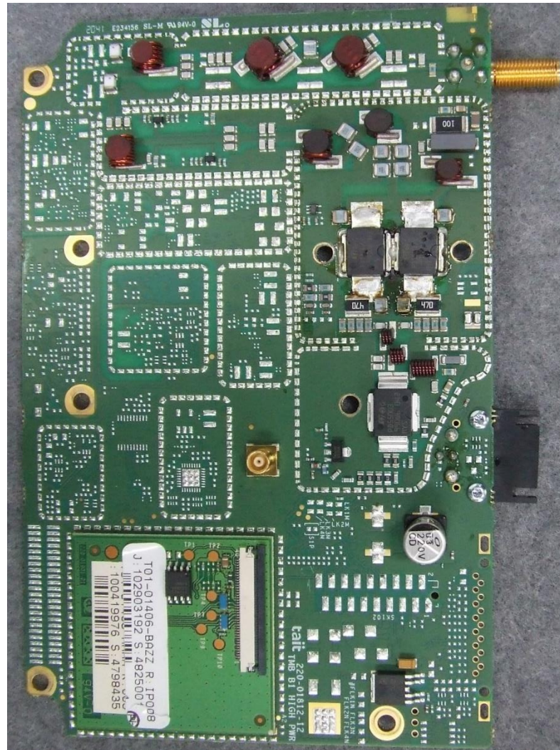
Photograph 10: Power Amplifier PCB – Top, cans off
