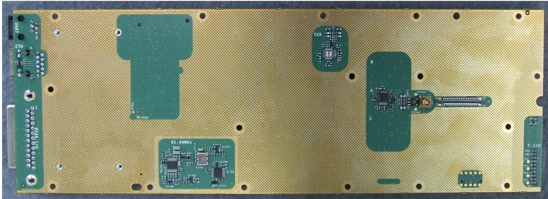
Photograph 17: Reciter Control Board (RCB) – Bottom
