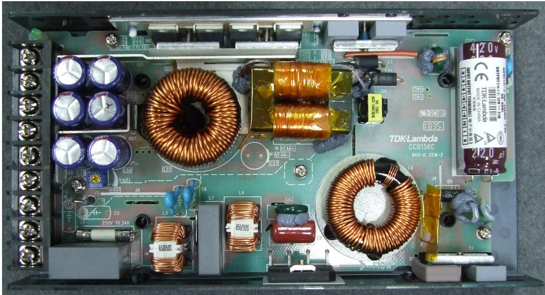
Photograph 05: AC Power Supply PCB - Top
