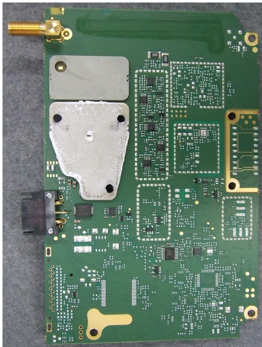
Photograph 12: Power Amplifier PCB – Bottom, cans off
