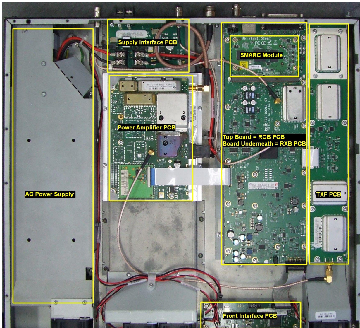
Photograph 02: Internal view – Labelled
