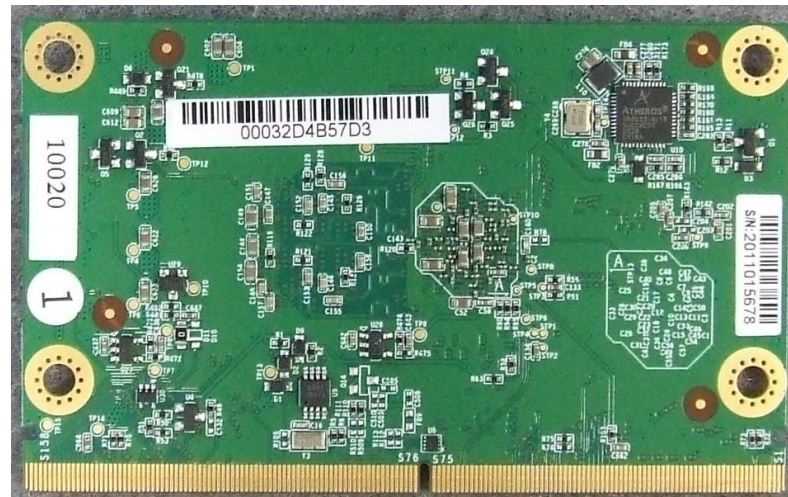
Photograph 16: RCB Smarc Module – Bottom
