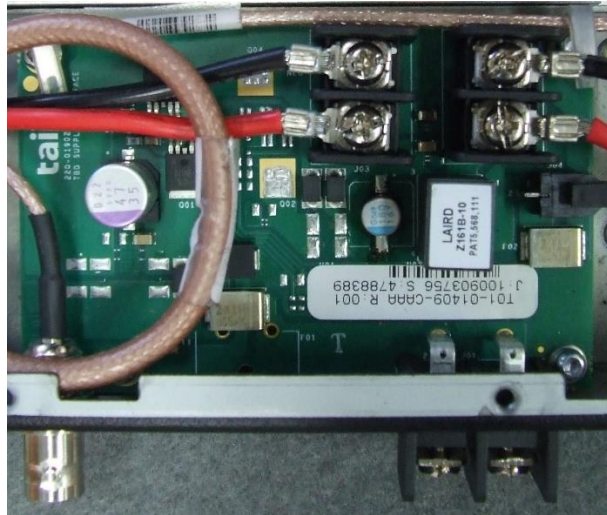
Photograph 07: Supply Interface PCB - Top
