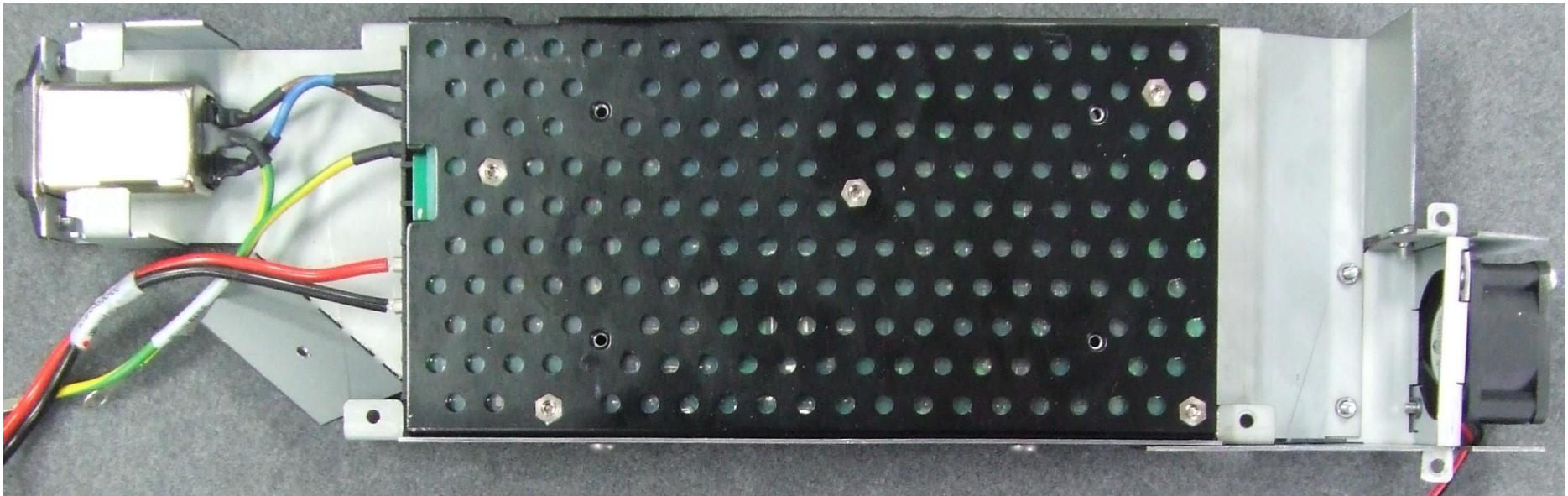
Photograph 06: AC Power Supply PCB - Bottom
